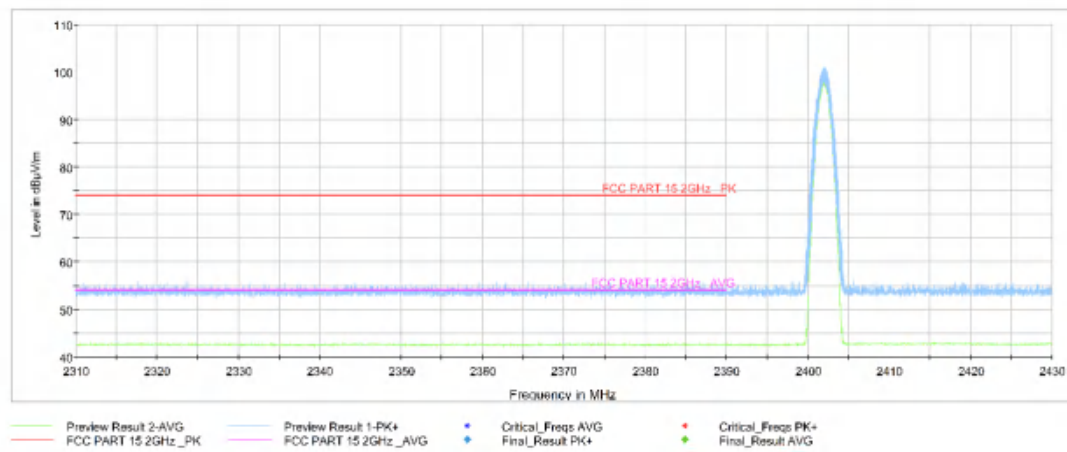
Fig.17. Frequency Band Edges: 8DPSK, Channel 0, 2.31 GHz - 2.45GHz
