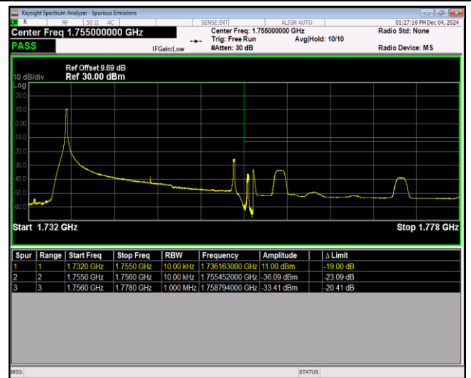
Band4-20MHz-16QAM-20300-100RB#0
