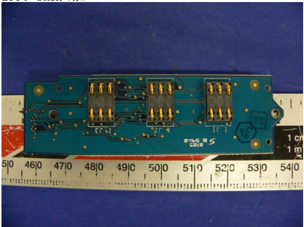
EUT 6 – Solder View
