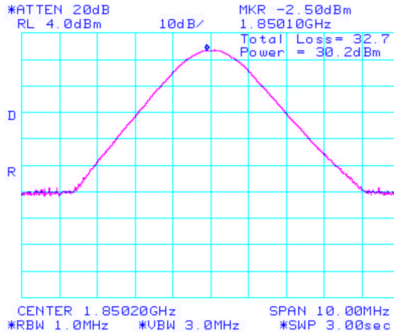
Figure 01: Channel 512 Peak Power
