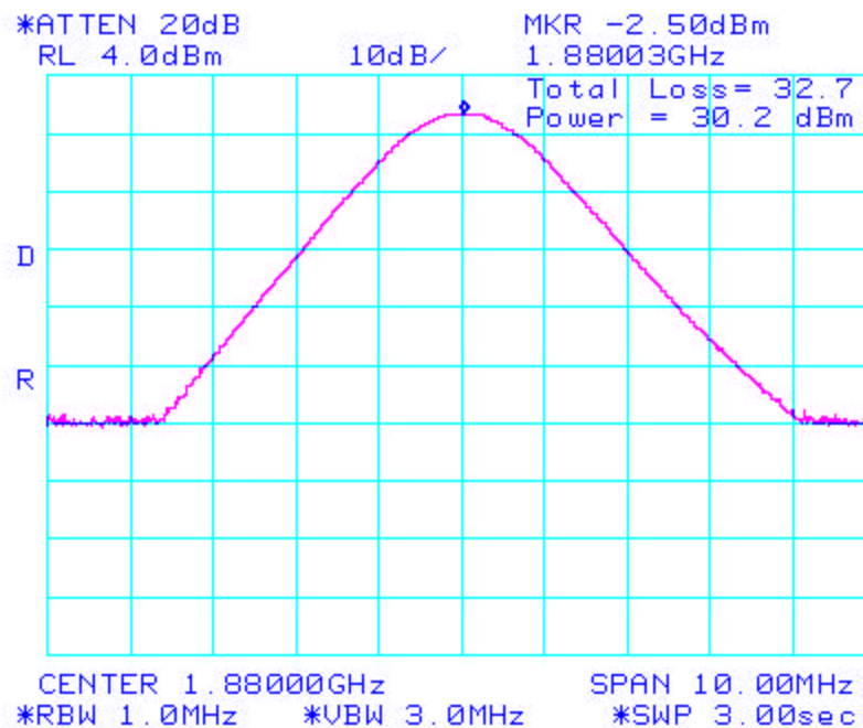
Figure 02: Channel 661 Peak Power
