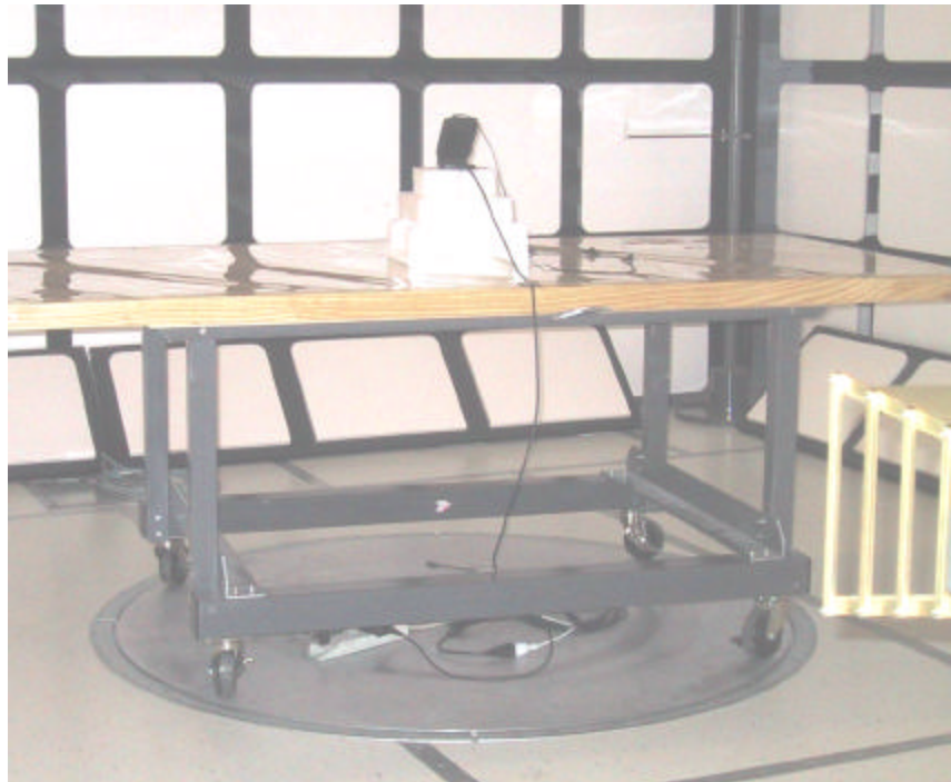
Radiated Emissions at 3.0 metres
