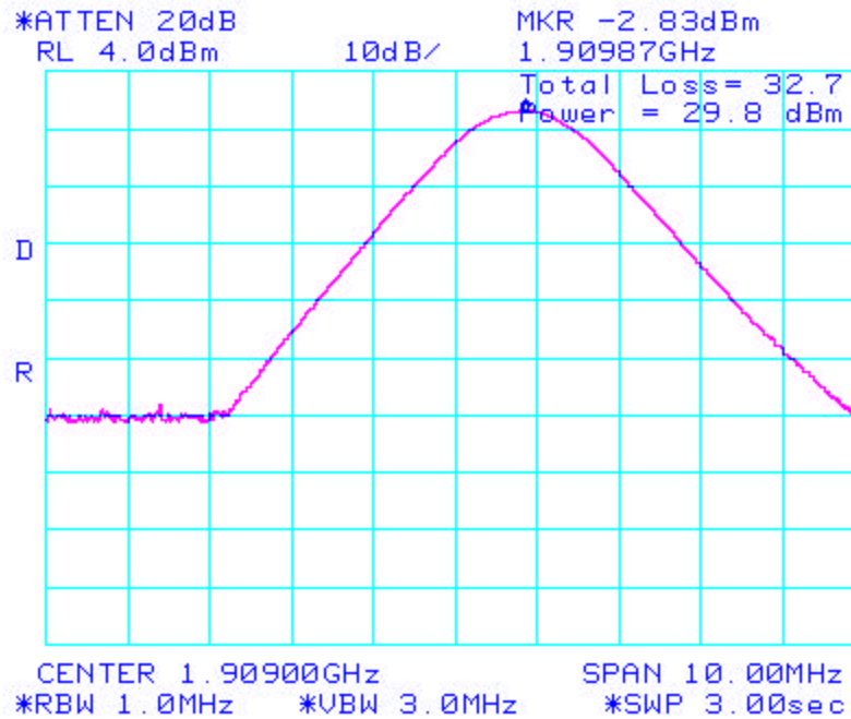
Figure 03: Channel 810 Peak Power
