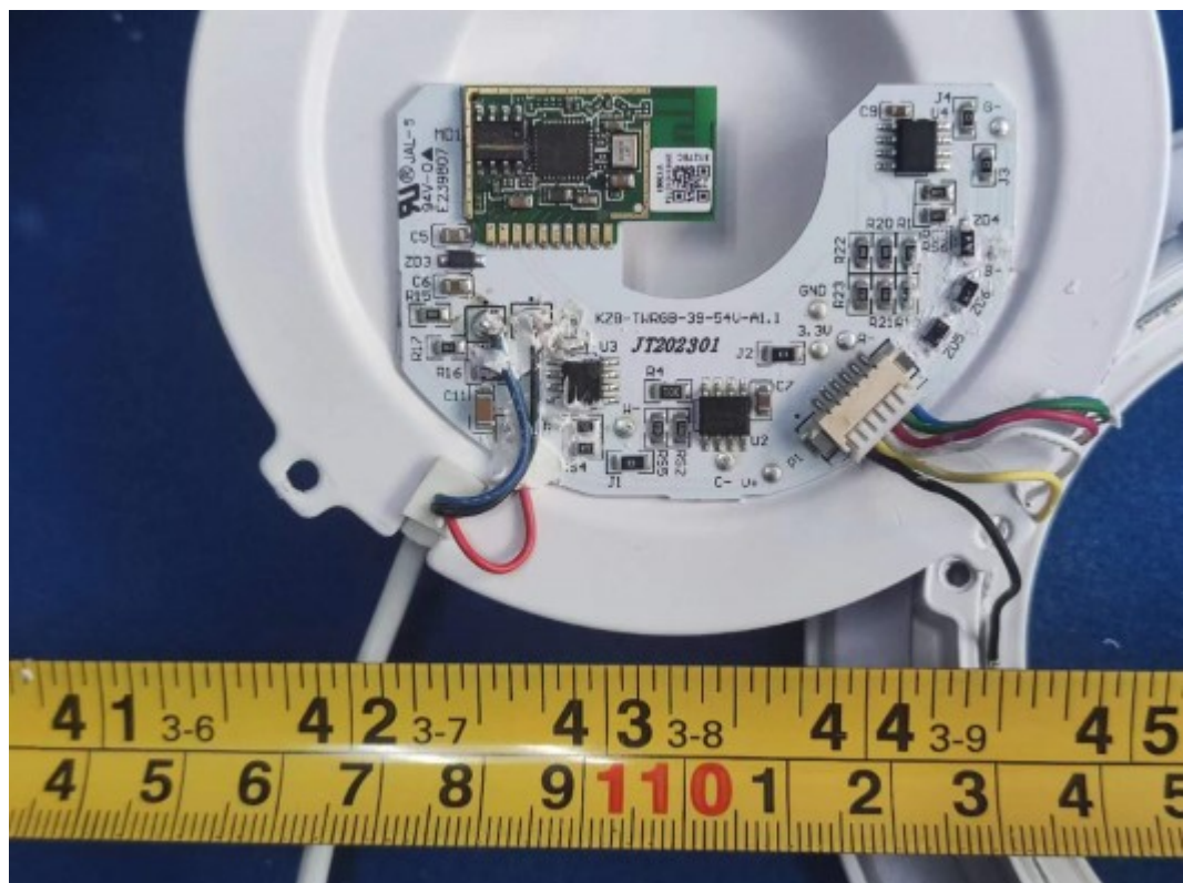
FIGURE 8 DOWNLIGHT (M/N: CFIXCNLR4SD) MAIN BOARD (COMPONENT SIDE)
