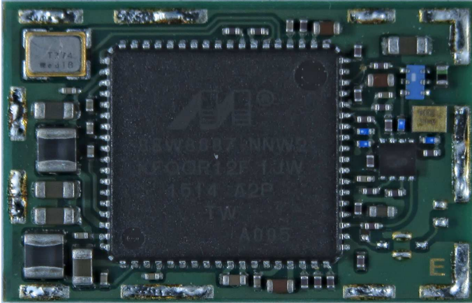
Figure 1: EMMY-W161 top view internal photo
