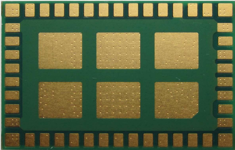
Figure 6: EMMY-W161, EMMY-W163, and EMMY-W165 bottom view
