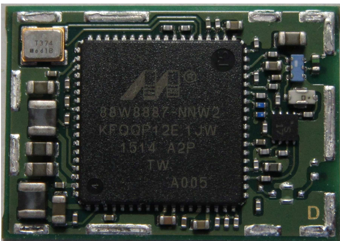
Figure 3: EMMY-W165 top view internal photo
