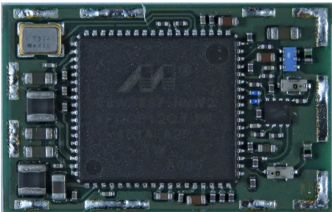
Figure 2: EMMY-W163 top view internal photo
