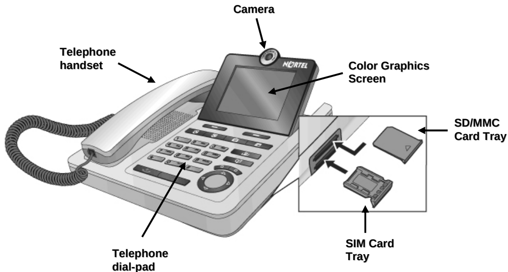
Fig. 1. Front view of the Videophone
