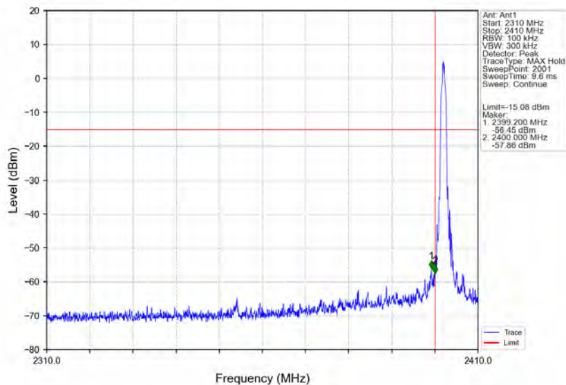
Pi/4DQPSK_2DH5_LCH_2402MHz_Ant1 NTN
