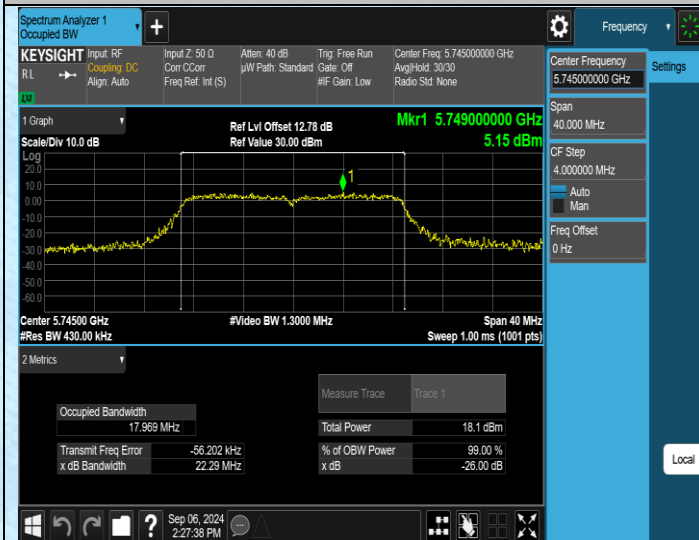
11AC20MIMO-Ant3-5745
