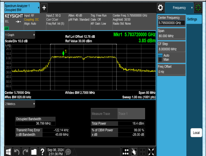
11AC40MIMO-Ant4-5795
