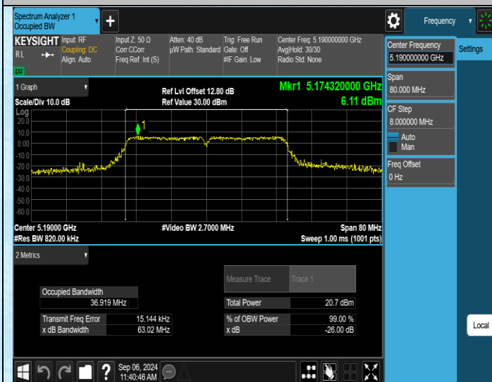
11AC40SISO-Ant3-5190
