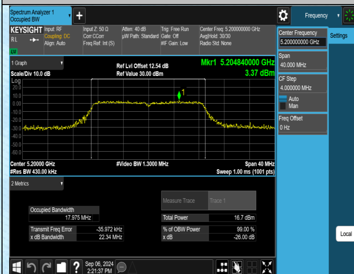
11AC20MIMO-Ant3-5200
