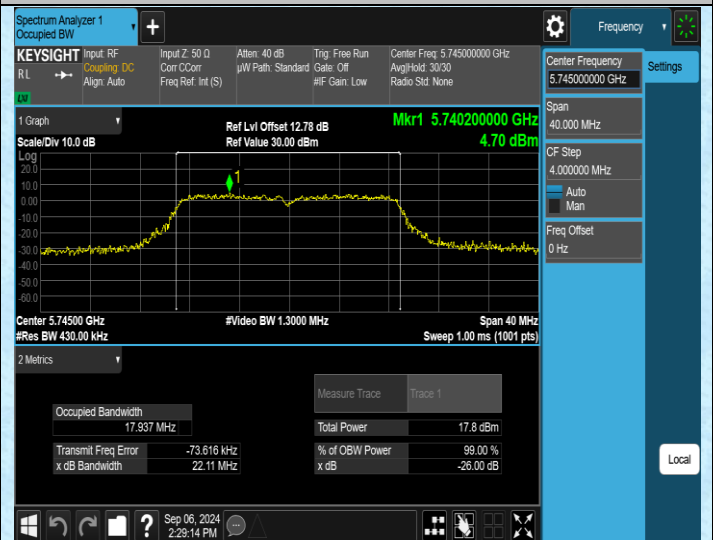
11AC20MIMO-Ant4-5745
