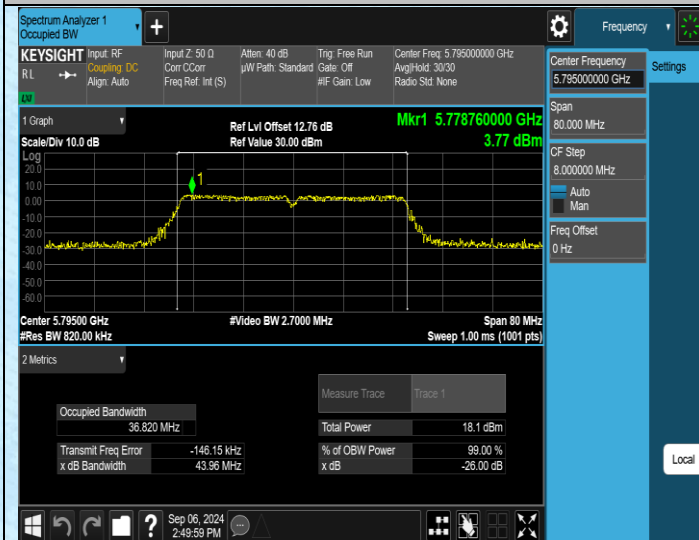
11AC40MIMO-Ant3-5795
