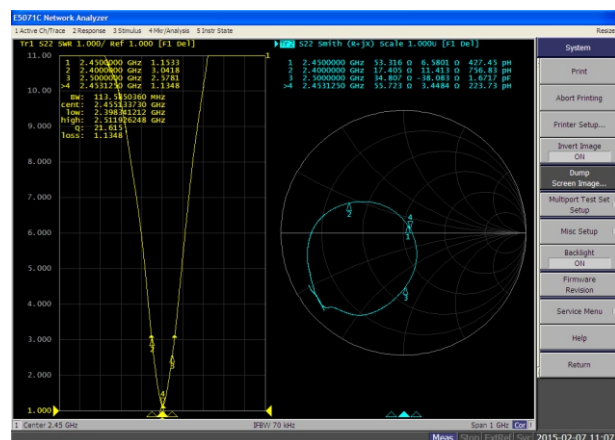
Fig.1 驻波比 VSWR
