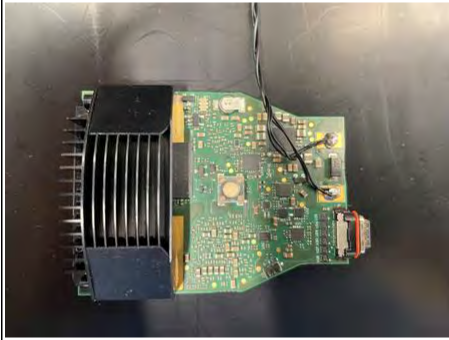
PROCESSORBOARD BOTTOM SIDE
