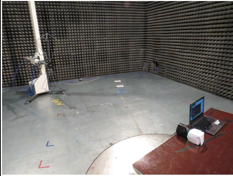
RADIATED EMISSION - 30 MHz to 200 MHz – EUT CONFIGURATION 1 / 3
