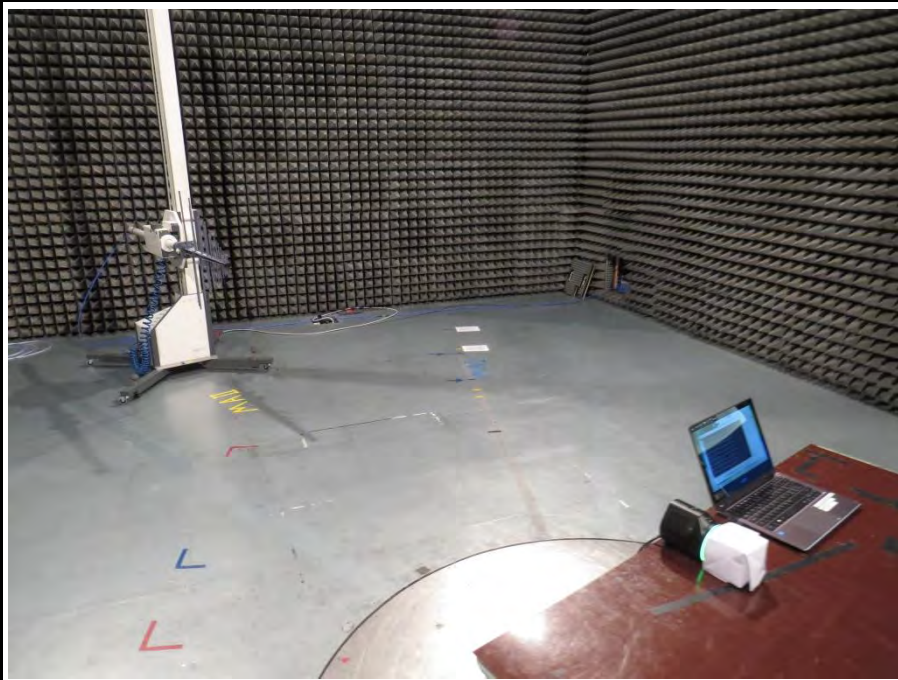
RADIATED EMISSION - 200 MHz to 1 GHz – EUT CONFIGURATION 1 / 3
