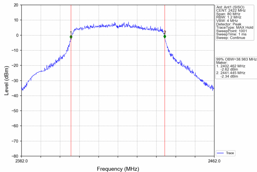
802.11ax(HEW40)_LCH_2422MHz_RU484_Left_Ant1 (SISO)_NTNV
