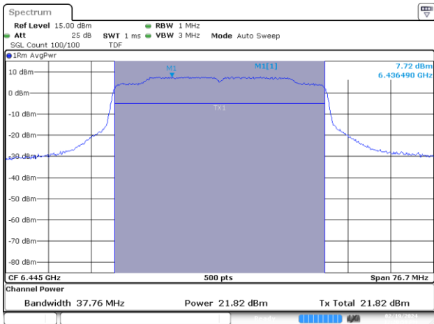
MIMO A-802.11ax/be-40MHz-Ch99-6445MHz-MCS0
