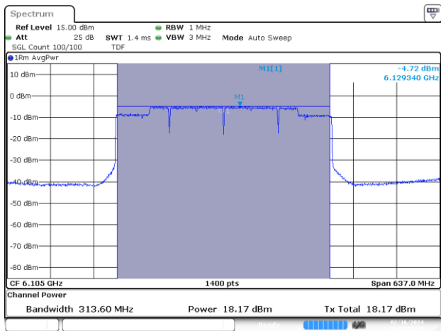
MIMO A-802.11be-320MHz-Ch31-6105MHz-MCS0
