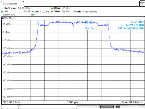
UNII6 SISO A 802.11ax/be160 ch111 6505MHz 99%
