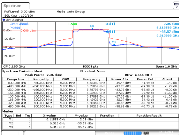
MIMO A-802.11be-320MHz-Ch31-6105MHz-MCS0
