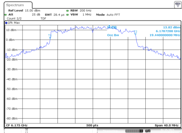
UNII5 SISO B 802.11ax/be20 ch45 6175MHz 99%
