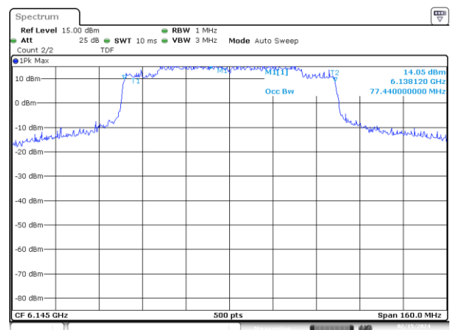
UNII5 SISO B 802.11ax/be80 ch39 6145MHz 99%
