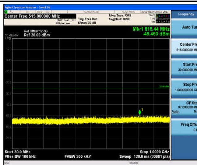
Band7_10MHz_16QAM_21400_1RB#0_Range2:1000~26000MHz_-32.84_PASS
