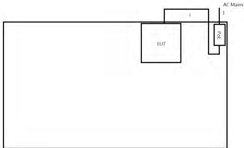
Test Setup Diagram – AC Line Conducted Emission Test <Sample 1>
