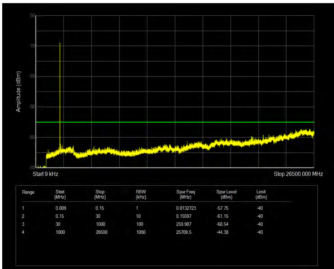
Band40(2305-2315) QPSK BW=5MHz Channel=38775 RB Size=1 Position=#0
