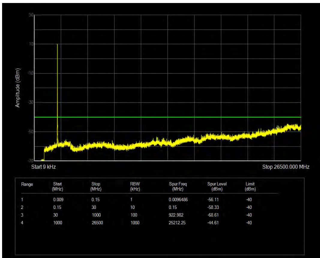
Band40(2305-2315) 16QAM BW=10MHz Channel=38750 RB Size=1 Position=#0
