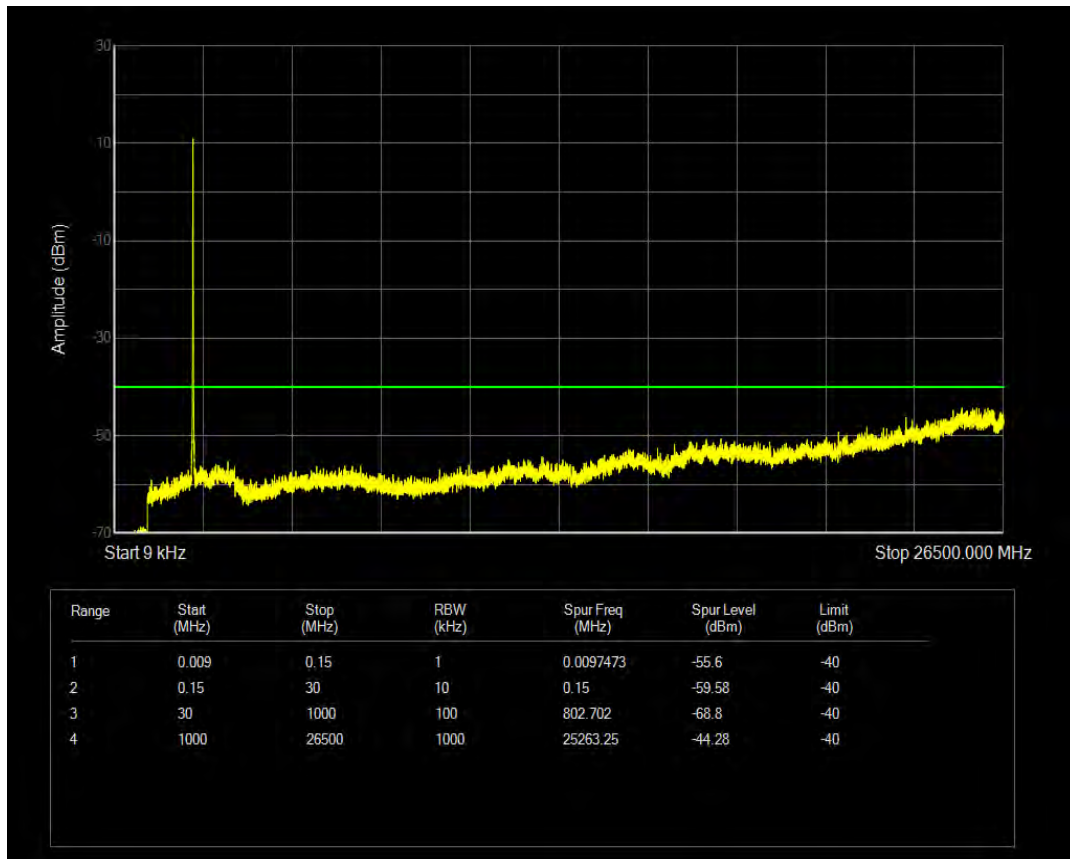
Band41(2555-2655) QPSK BW=5MHz Channel=40265 RB Size=1 Position=#0
