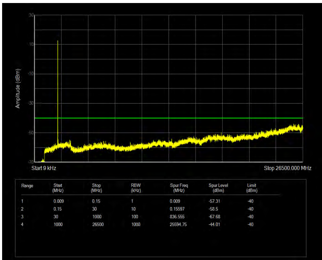
Band40(2305-2315) 16QAM BW=5MHz Channel=38725 RB Size=1 Position=#0
