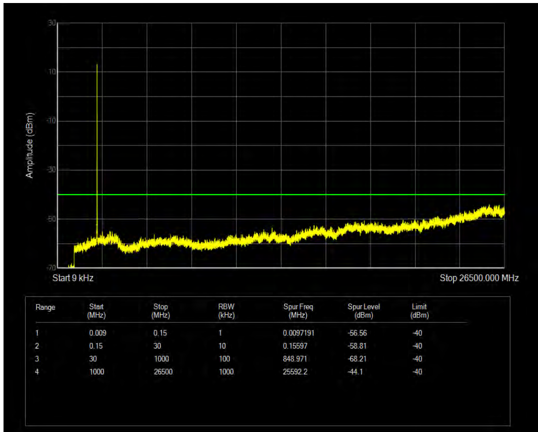
Band40(2350-2360) QPSK BW=5MHz Channel=39225 RB Size=1 Position=#0
