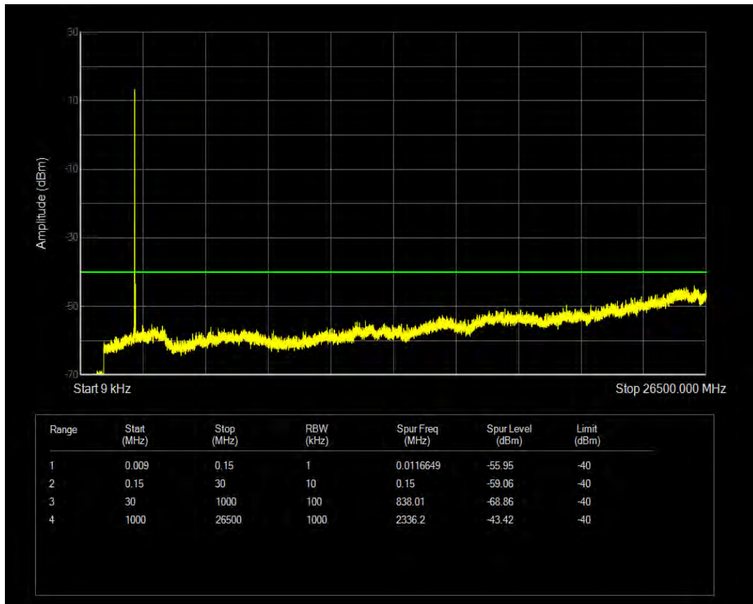
Band40(2305-2315) QPSK BW=5MHz Channel=38750 RB Size=1 Position=#0
