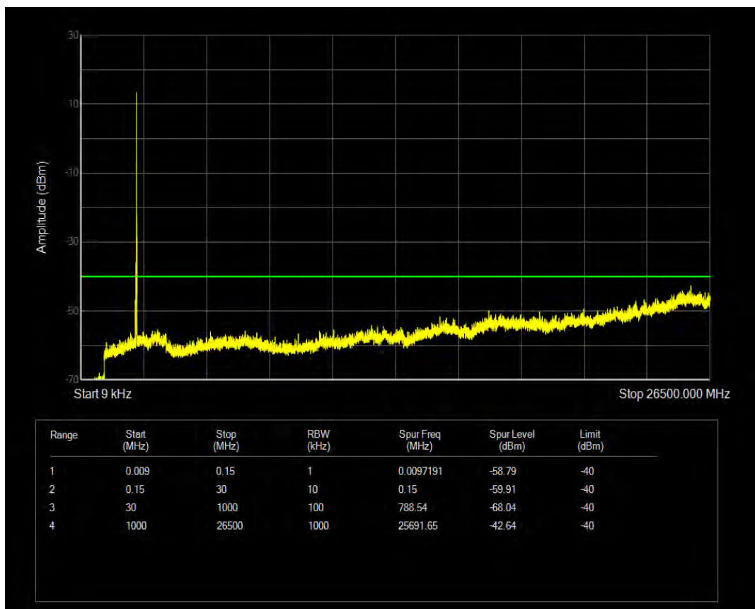
Band40(2350-2360) 16QAM BW=10MHz Channel=39200 RB Size=50 Position=#0
