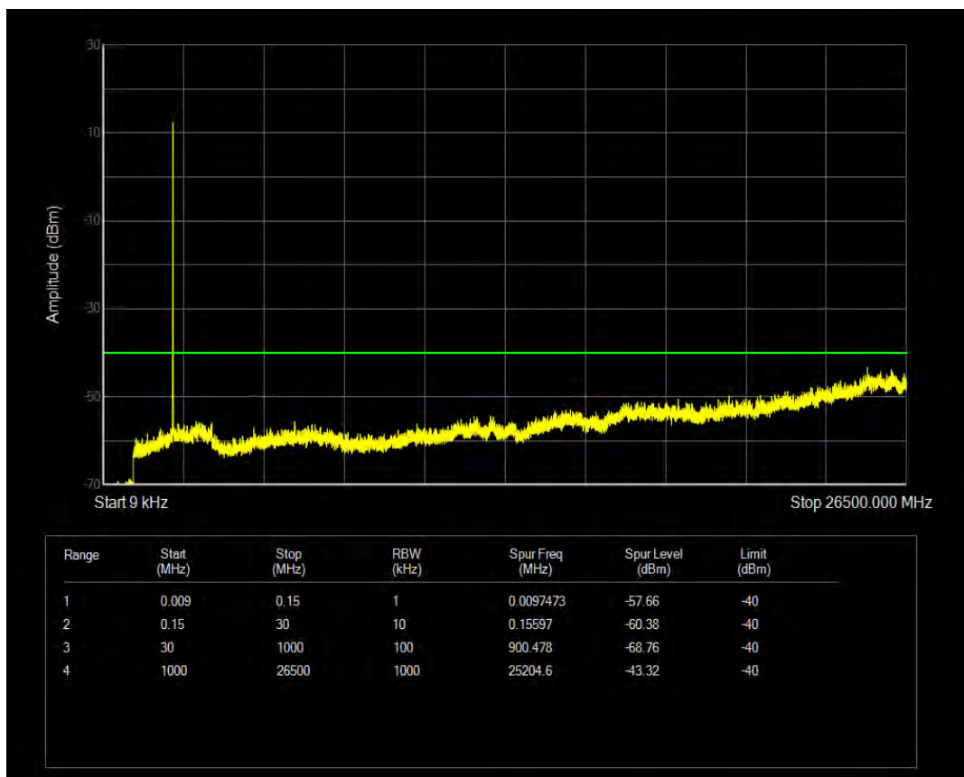
Band40(2305-2315) 16QAM BW=5MHz Channel=38750 RB Size=1 Position=#0
