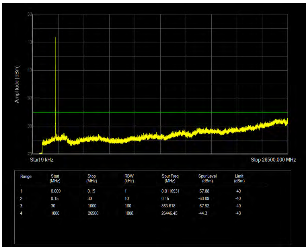
Band40(2350-2360) 16QAM BW=5MHz Channel=39200 RB Size=1 Position=#0
