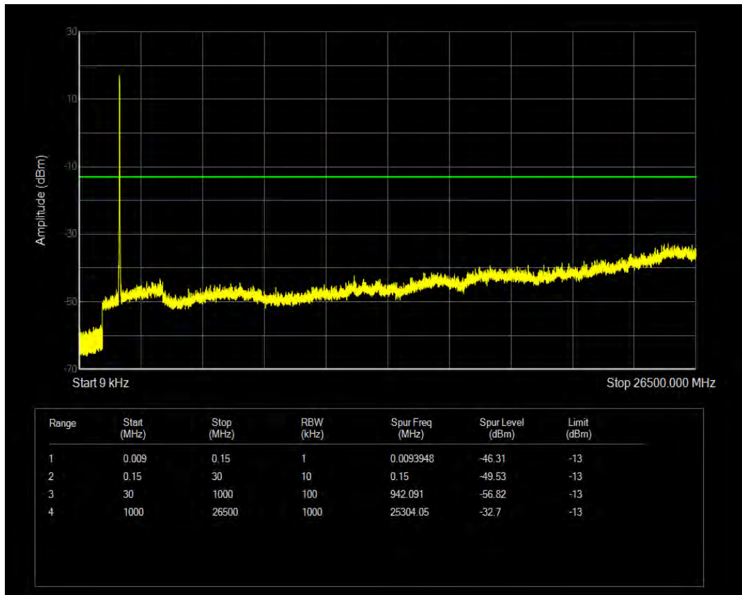
Band40(2305-2315) QPSK BW=5MHz Channel=38725 RB Size=1 Position=#0
