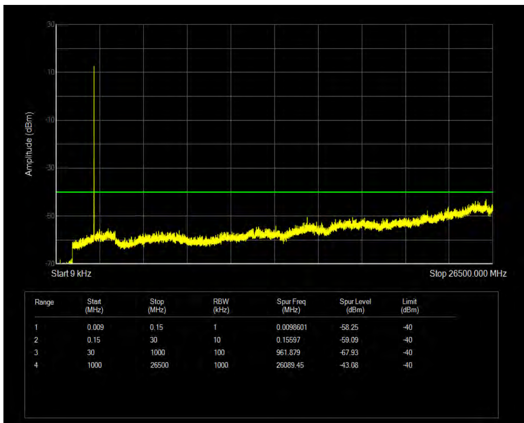
Band40(2305-2315) 16QAM BW=5MHz Channel=38775 RB Size=1 Position=#0
