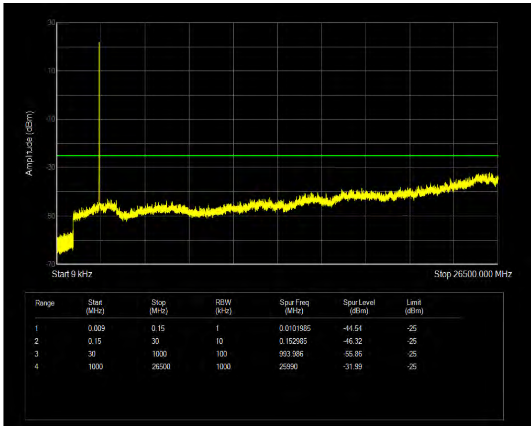
Band41(2555-2655) 16QAM BW=5MHz Channel=40265 RB Size=1 Position=#0
