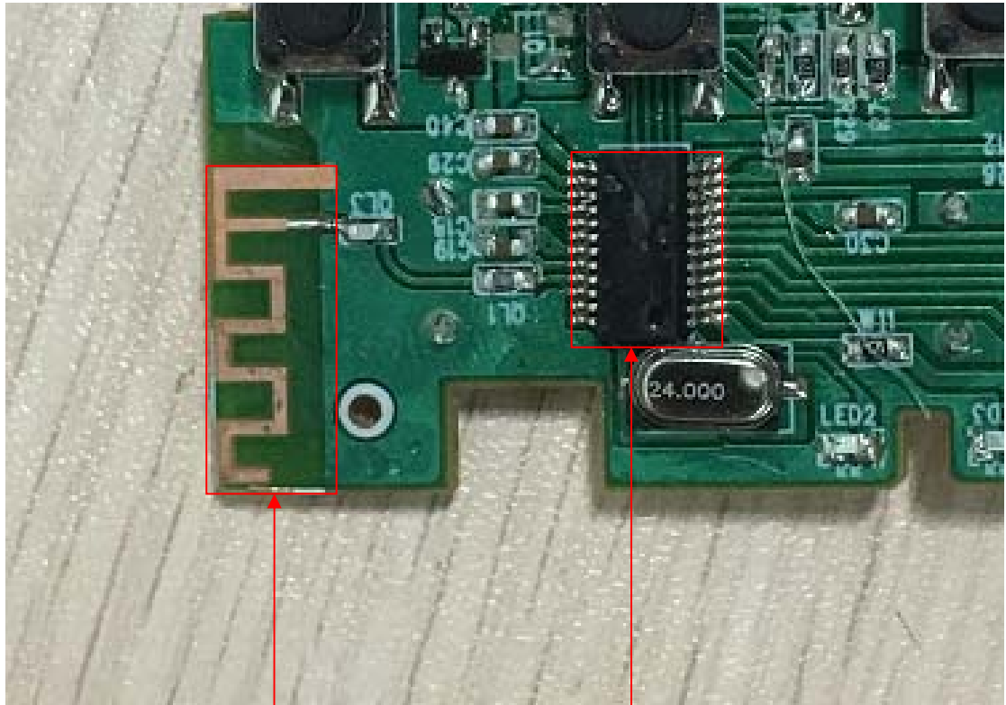
BT Antenna
