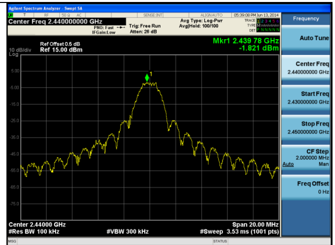
PSD-Zigbee 2440
