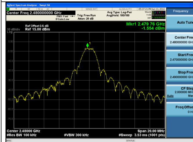
PSD-Zigbee 2480
