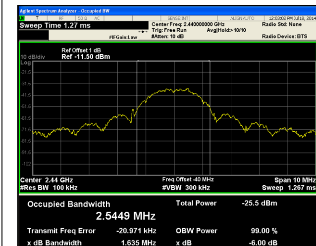
99% BW TX-Zigbee 2440
