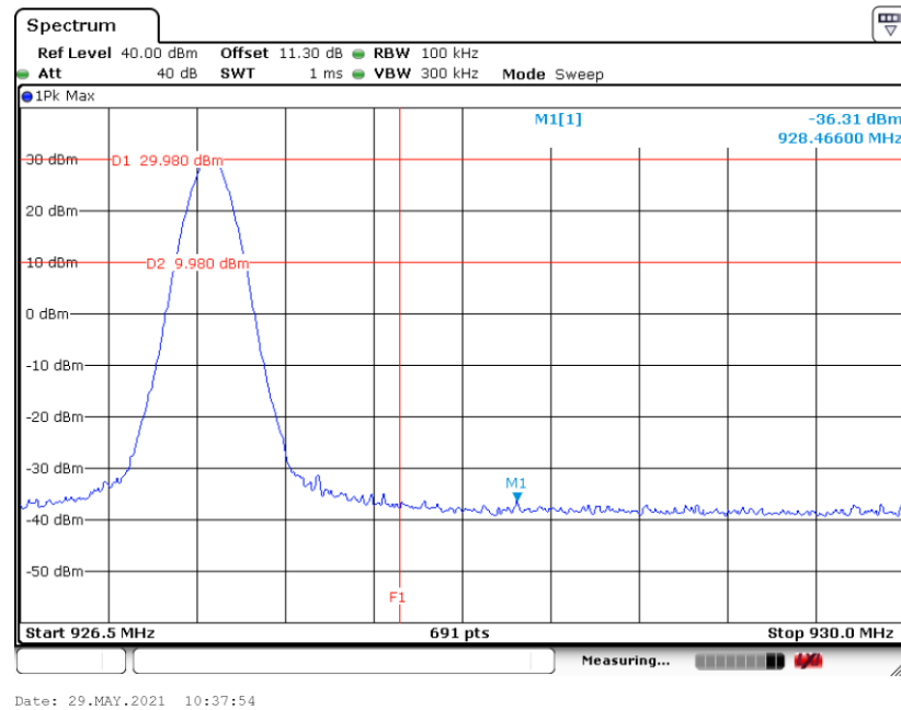
High Band Edge Plot on Channel 49
