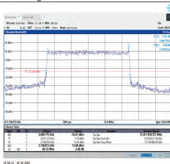
1-N77-3700-3980-PC1-30-60-L-8-CP-64QAM-Outer_Full-162@0-Ant1-57.812-60.120-≤60-PASS
