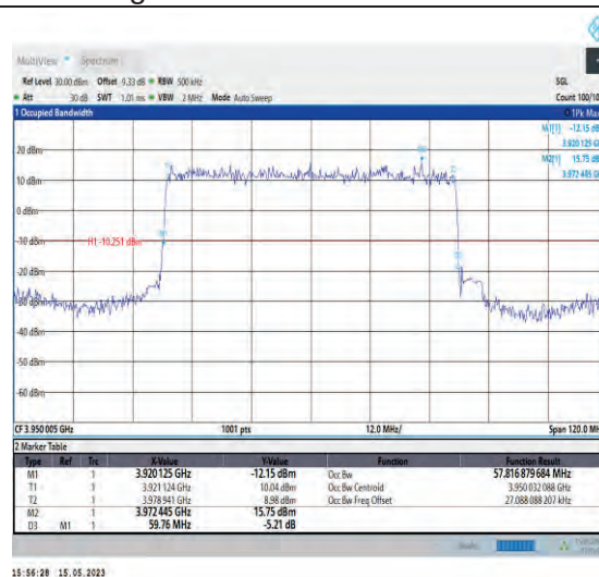
1-N77-3700-3980-PC1-30-60-H-2-DFT-PI2BPSK-Out_ Full-162@0-Ant1-57.817-59.760-≤60-PASS
