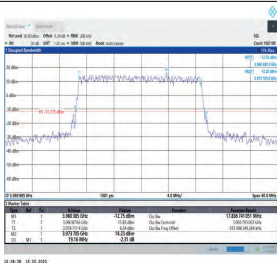
1-N77-3700-3980-PC1-30-20-H-3-DFT-16QAM-Out_ Full-50@0-Ant1-17.837-19.160-≤20-PASS
