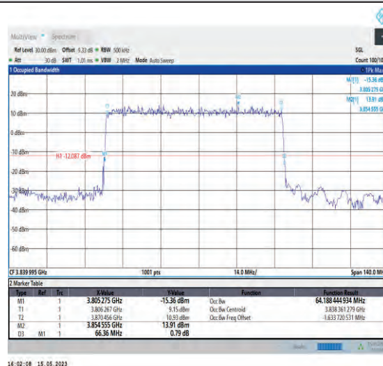
1-N77-3700-3980-PC1-30-70-M-2-DFT-PI2BPSK-Outer_Full-180@0-Ant1-64.188-66.360-≤70-PASS
