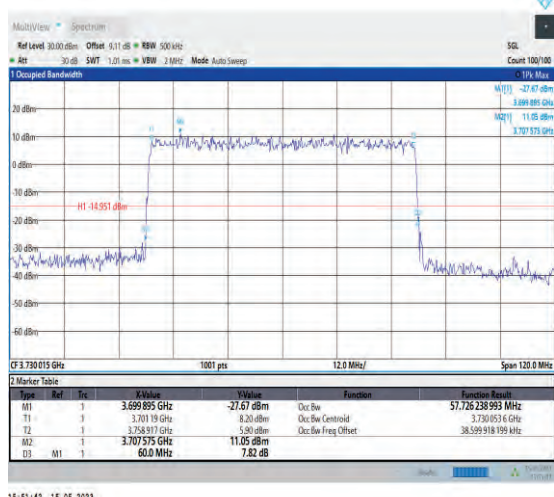
1-N77-3700-3980-PC1-30-60-L-5-DFT-256QAM-Outer_Full-162@0-Ant1-57.726-60.000-≤60-PASS
