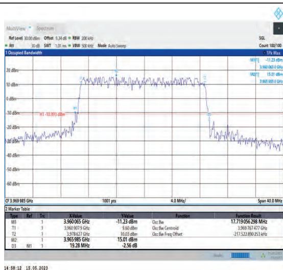
1-N77-3700-3980-PC1-30-20-H-1-DFT-QPSK-Out_ Full-50@0-Ant1-17.719-19.280-≤20-PASS
