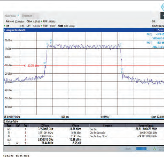
1-N77-3700-3980-PC1-30-30-H-1-DFT-QPSK-Outer_Full-75@0-Ant1-26.812-28.440-≤30-PASS
