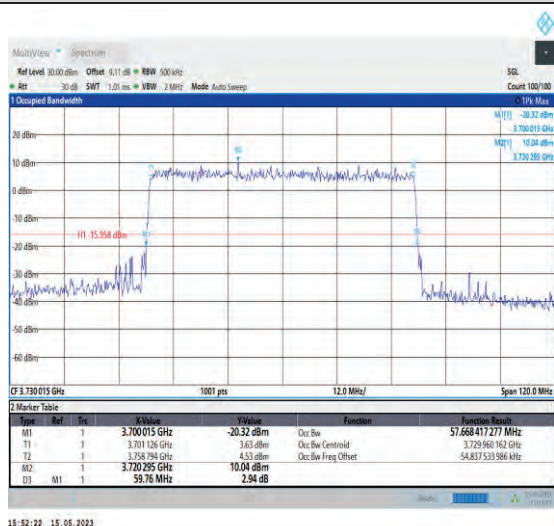
1-N77-3700-3980-PC1-30-60-L-9-CP-256QAM-Outer_Full-162@0-Ant1-57.668-59.760-≤60-PASS
