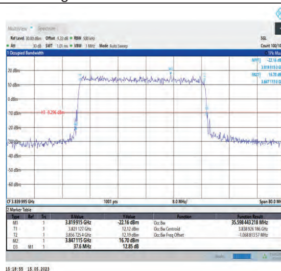
1-N77-3700-3980-PC1-30-40-M-1-DFT-QPSK-Outer_Full-100@0-Ant1-35.598-37.600-≤40-PASS
