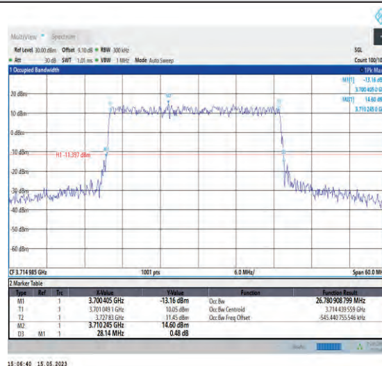
1-N77-3700-3980-PC1-30-30-L-3-DFT-16QAM-Outer_Full-75@0-Ant1-26.781-28.140-≤30-PASS
