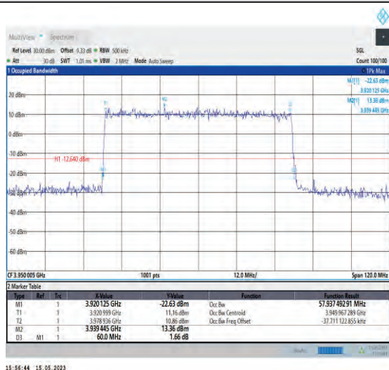
1-N77-3700-3980-PC1-30-60-H-3-DFT-16QAM-Out_ Full-162@0-Ant1-57.937-60.000-≤60-PASS
