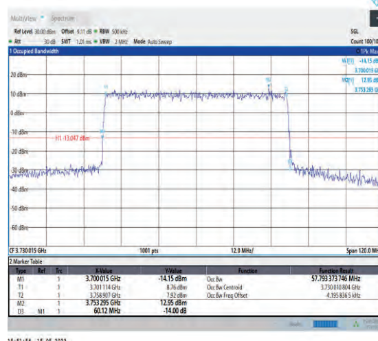
1-N77-3700-3980-PC1-30-60-L-6-CP-QPSK-Outer_Full-162@0-Ant1-57.793-60.120-≤60-PASS
