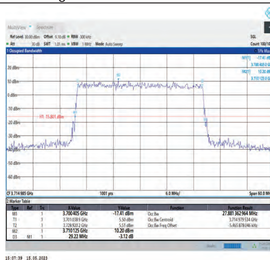
1-N77-3700-3980-PC1-30-30-L-9-CP-256QAM-Outer_Full-78@0-Ant1-27.881-29.220-≤30-PASS
