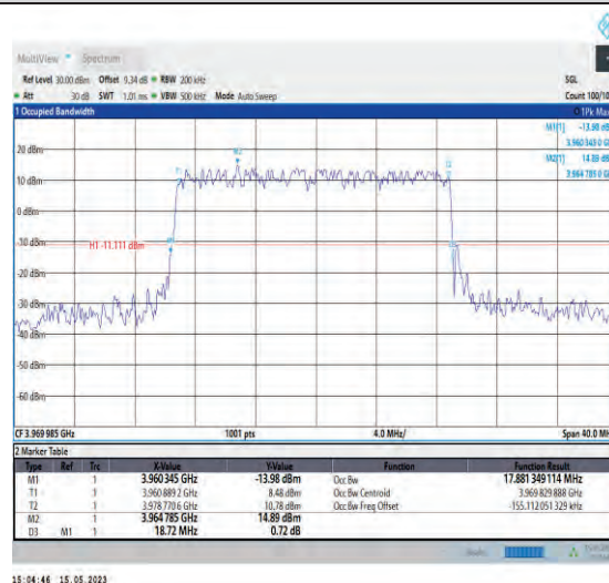
1-N77-3700-3980-PC1-30-20-H-4-DFT-64QAM-Out_ Full-50@0-Ant1-17.881-18.720-≤20-PASS
