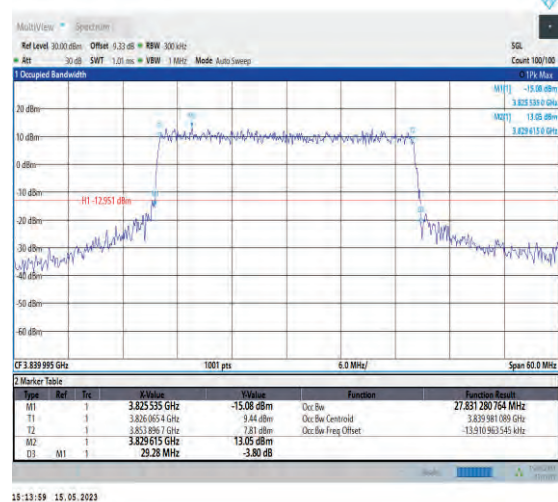
1-N77-3700-3980-PC1-30-30-M-6-CP-QPSK-Out_er_Full-78@0-Ant1-27.831-29.280-≤30-PASS
