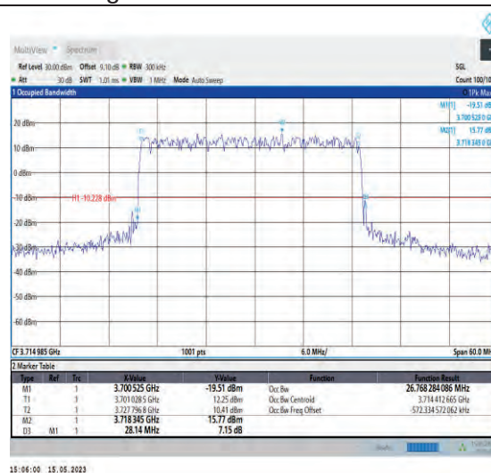
1-N77-3700-3980-PC1-30-30-L-1-DFT-QPSK-Outer_Full-75@0-Ant1-26.768-28.140-≤30-PASS
