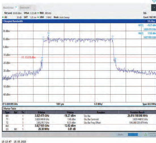
1-N77-3700-3980-PC1-30-30-M-5-DFT-256QAM-Out_er_Full-75@0-Ant1-26.816-28.380-≤30-PASS
