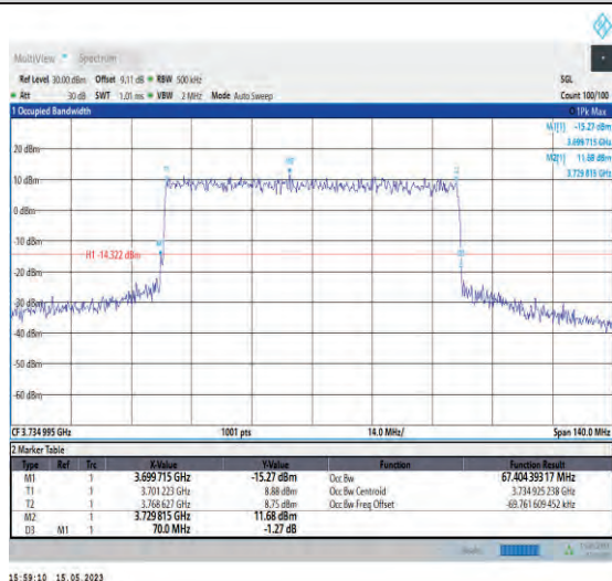
1-N77-3700-3980-PC1-30-70-L-6-CP-QPSK-Outer_Full-189@0-Ant1-67.404-70.000-≤70-PASS
