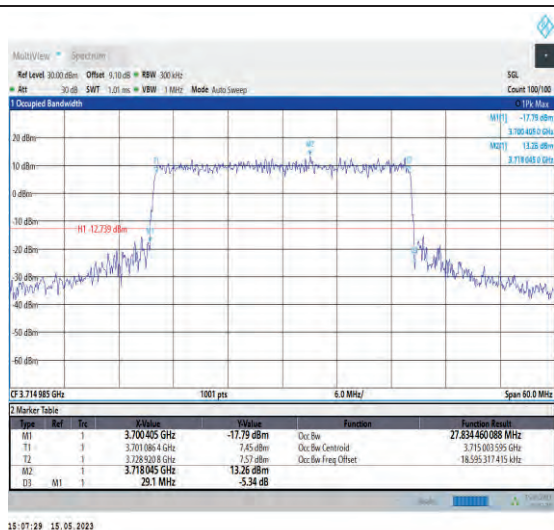
1-N77-3700-3980-PC1-30-30-L-8-CP-64QAM-Outer_Full-78@0-Ant1-27.834-29.100-≤30-PASS
