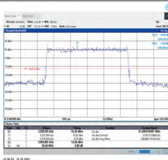
1-N77-3700-3980-PC1-30-60-H-4-DFT-64QAM-Out_ Full-162@0-Ant1-57.649-59.640-≤60-PASS
