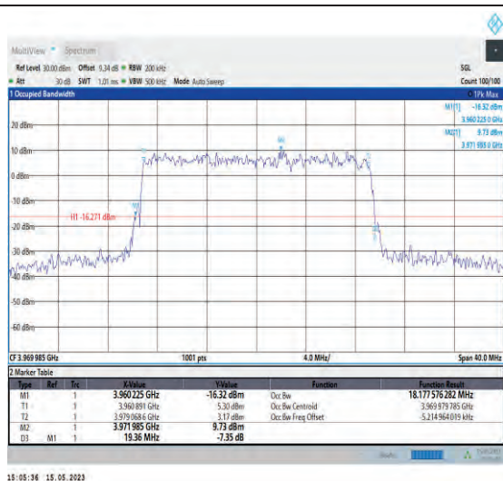
1-N77-3700-3980-PC1-30-20-H-9-CP-256QAM-Outer_Full-51@0-Ant1-18.178-19.360-≤20-PASS
