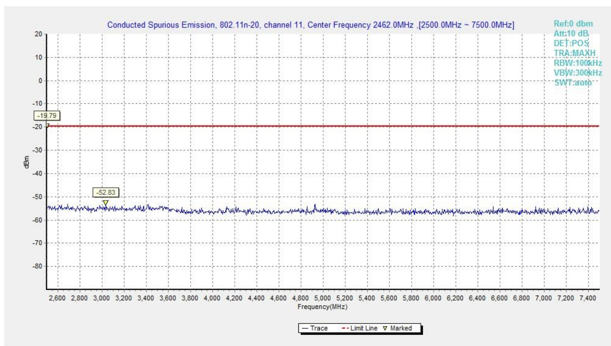
Fig.A.6.1.100 Conducted Spurious Emission (802.11n-HT20, Ch11, 2.5 GHz-7.5 GHz)
