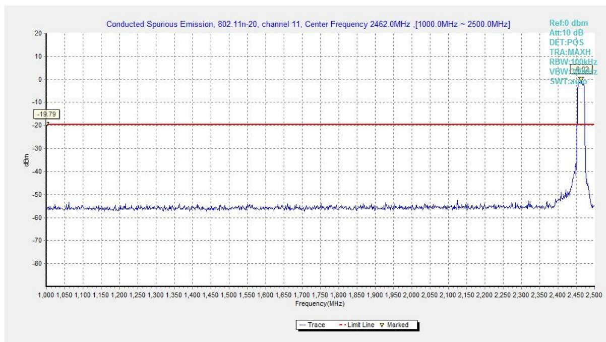
Fig.A.6.1.99 Conducted Spurious Emission (802.11n-HT20, Ch11, 1 GHz-2.5 GHz)
