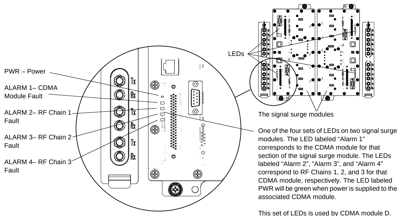
Figure 4–12 Alarm LEDs
