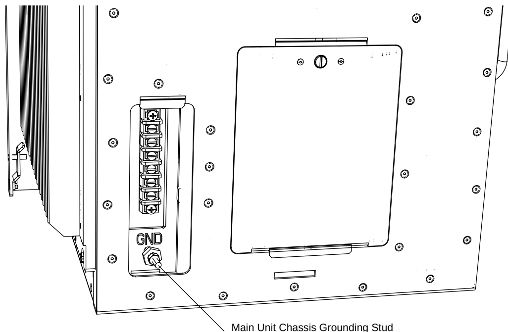
Figure 4-5 Connecting the Ground Cable to the Main Unit
