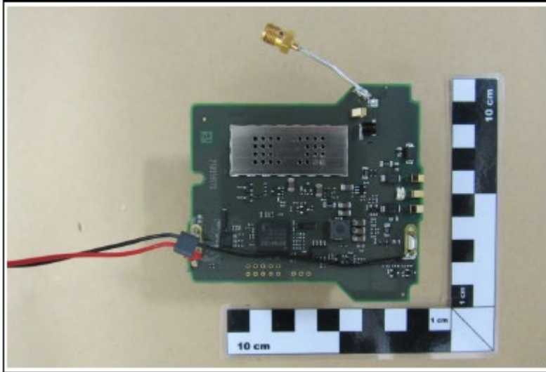
CONDUCTED SAMPLE
