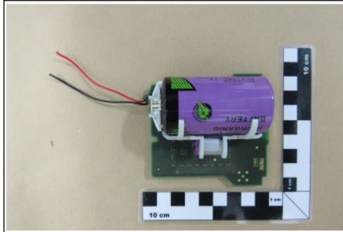
RADIATED SAMPLE
