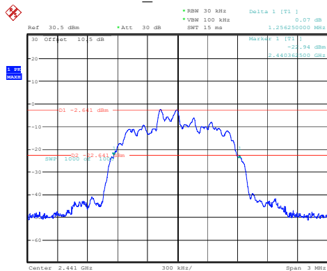
2DH1_Middle 1.256MHz
