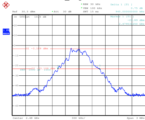
DH1_High 0.945MHz
