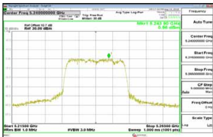
802.11a_20MHz_5240MHz
