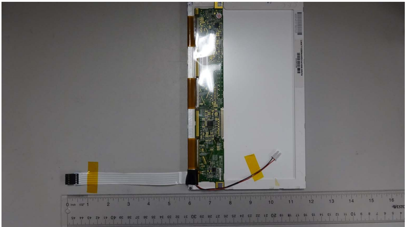
LCD Panel (Rear View)
