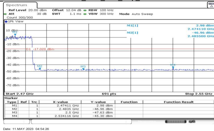
3DH5_Ant1_High_Hop_2480
