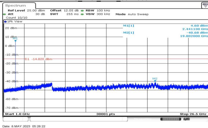
DH5_Ant1_2441_1000-26500
