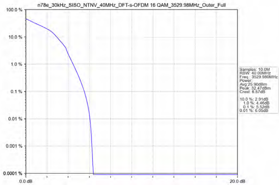
n78e_30kHz_SISO_NTNV_40MHz_DFT-s-OFDM_16_QAM_3529.98MHz_Outer_Full_Ant13
