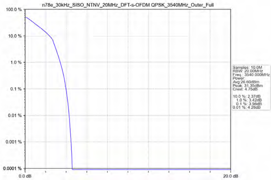
n78e_30kHz_SISO_NTNV_20MHz_DFT-s-OFDM_QPSK_3540MHz_Outer_Full_Ant13
