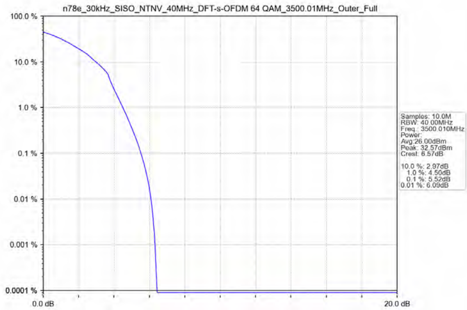
n78e_30kHz_SISO_NTNV_40MHz_DFT-s-OFDM_64_QAM_3500.01MHz_Outer_Full_Ant13
