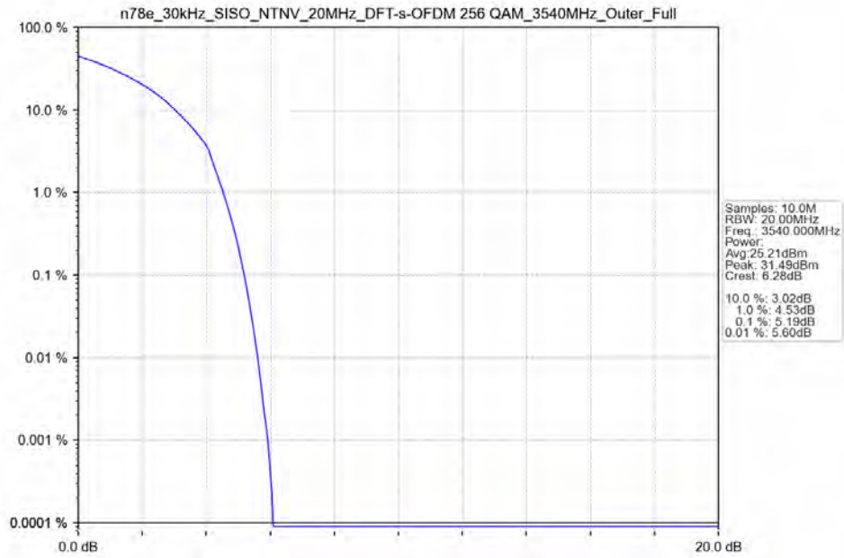
n78e 30kHz SISO NTN 20MHz DFT-s-OFDM 256 QAM 3540MHz Outer Full Ant13
