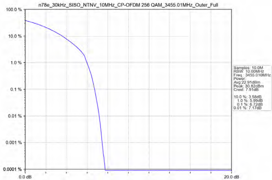
n78e 30kHz SISO NTN 10MHz CP-OFDM 256 QAM 3455.01MHz Outer Full Ant13
