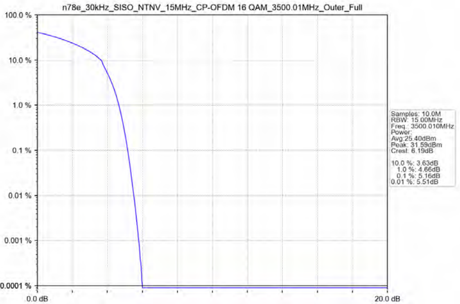
n78e 30kHz SISO NTN 15MHz CP-OFDM 16 QAM 3500.01MHz Outer Full Ant13
