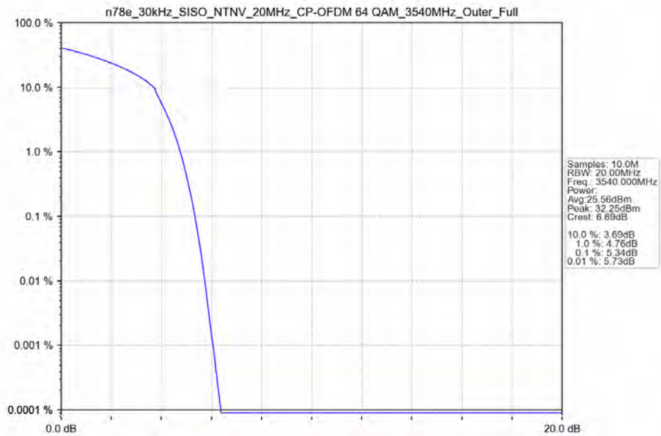
n78e_30kHz_SISO_NTNV_20MHz_CP-OFDM 64 QAM_3540MHz_Outer_Full_Ant13
