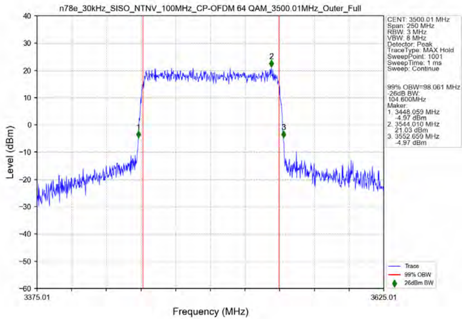
n78e 30kHz SISO NTN 100MHz CP-OFDM 64 QAM 3500.01MHz Outer Full Ant13
