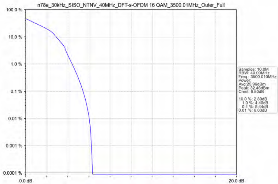
n78e_30kHz_SISO_NTNV_40MHz_DFT-s-OFDM_16_QAM_3500.01MHz_Outer_Full_Ant13
