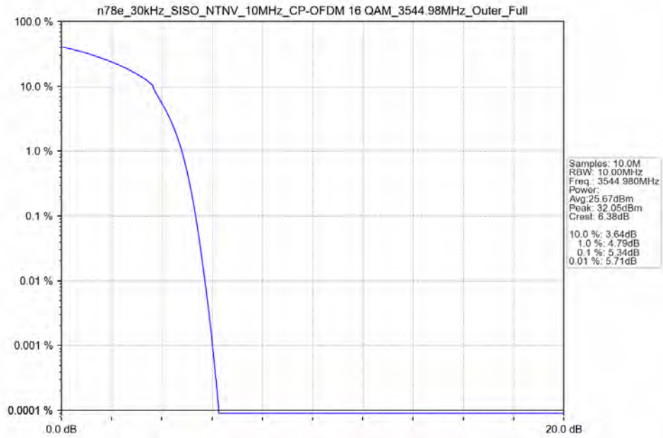
n78e_30kHz_SISO_NTNV_10MHz_CP-OFDM 16 QAM 3544.98MHz_Outer_Full_Ant13
