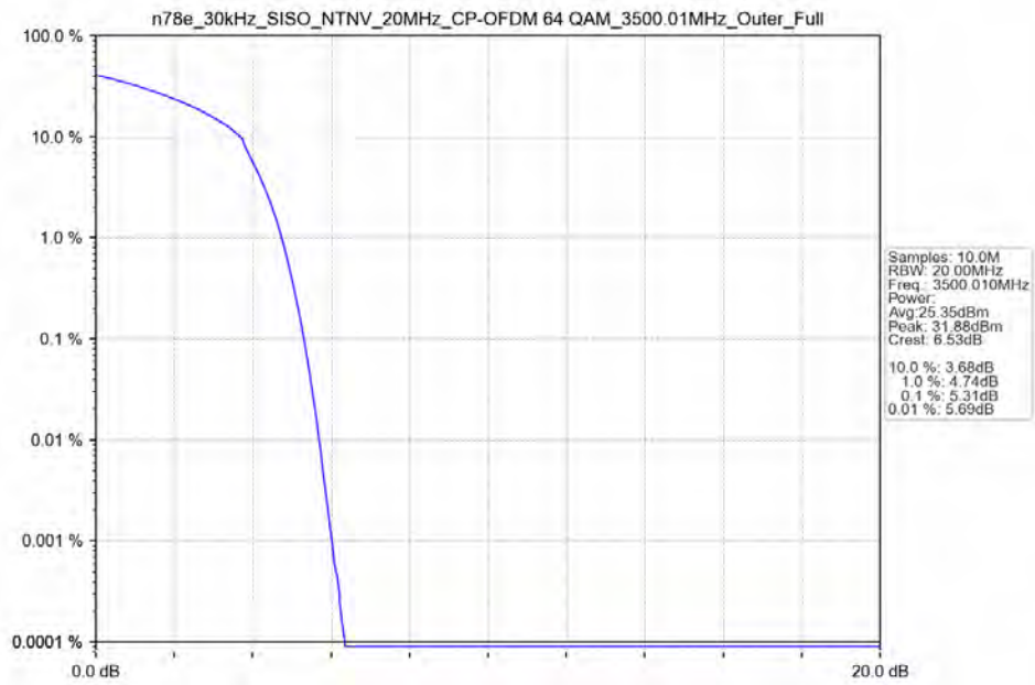
n78e_30kHz_SISO_NTNV_20MHz_CP-OFDM 64 QAM_3500.01MHz_Outer_Full_Ant13
