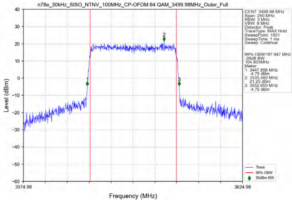
n78e_30kHz_SISO_NTNV_100MHz_CP-OFDM 64 QAM_3499.98MHz_Outer_Full_Ant13
