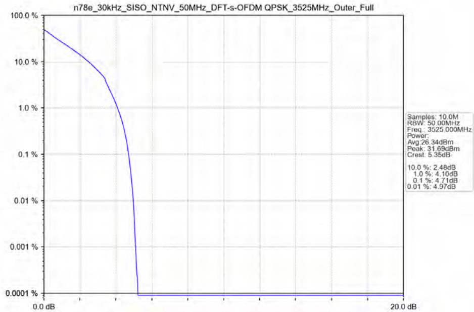
n78e_30kHz_SISO_NTNV_50MHz_DFT-s-OFDM_QPSK_3525MHz_Outer_Full_Ant13
