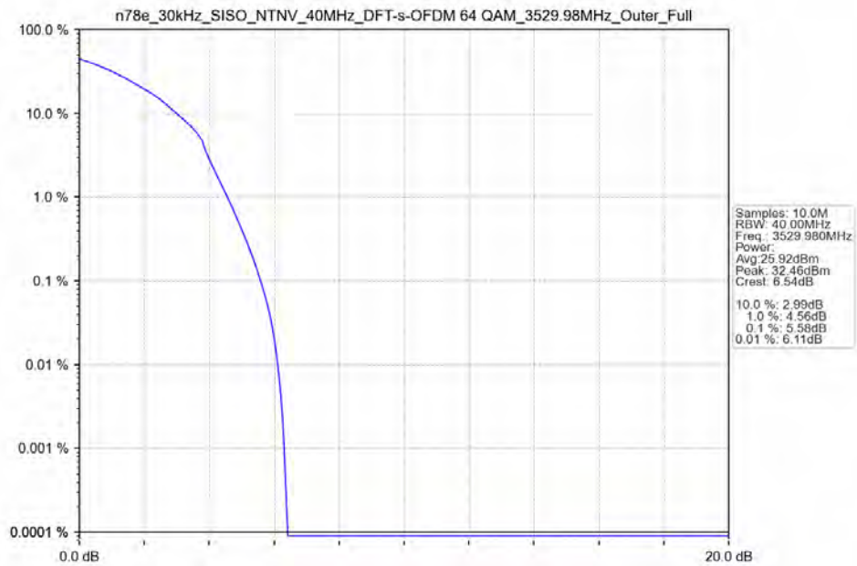
n78e_30kHz_SISO_NTNV_40MHz_DFT-s-OFDM_64_QAM_3529.98MHz_Outer_Full_Ant13
