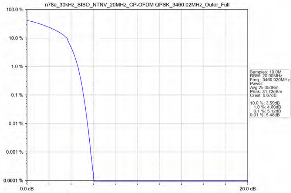
n78e 30kHz SISO NTN 20MHz CP-OFDM QPSK 3460.02MHz Outer Full Ant13
