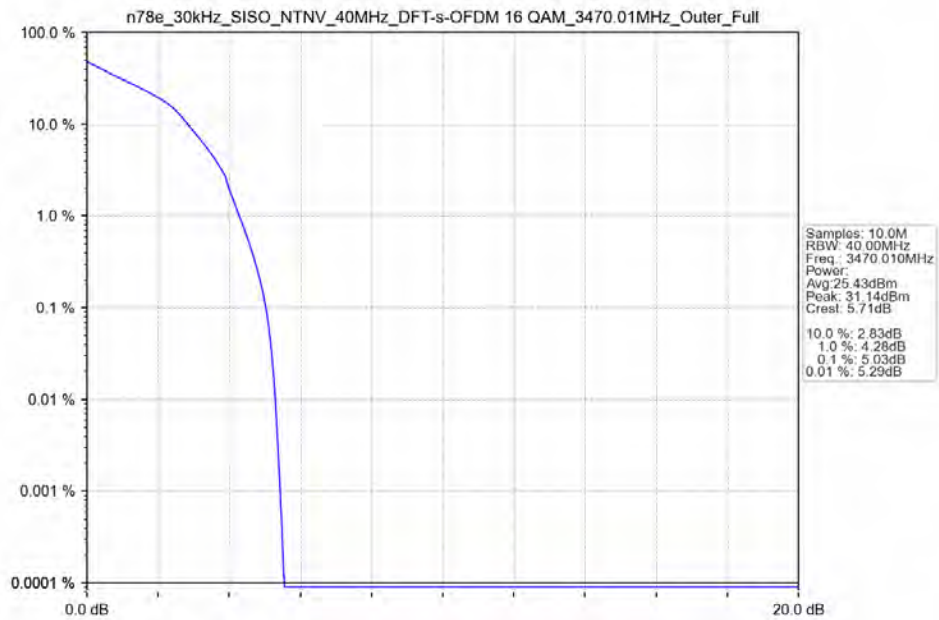
n78e_30kHz_SISO_NTNV_40MHz_DFT-s-OFDM_16_QAM_3470.01MHz_Outer_Full_Ant13
