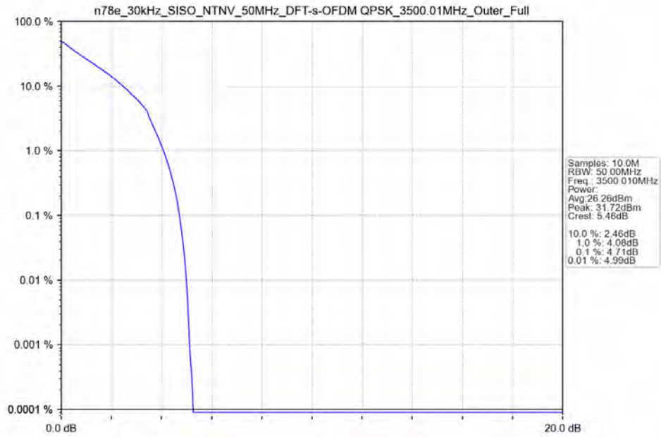
n78e_30kHz_SISO_NTNV_50MHz_DFT-s-OFDM_QPSK_3500.01MHz_Outer_Full_Ant13
