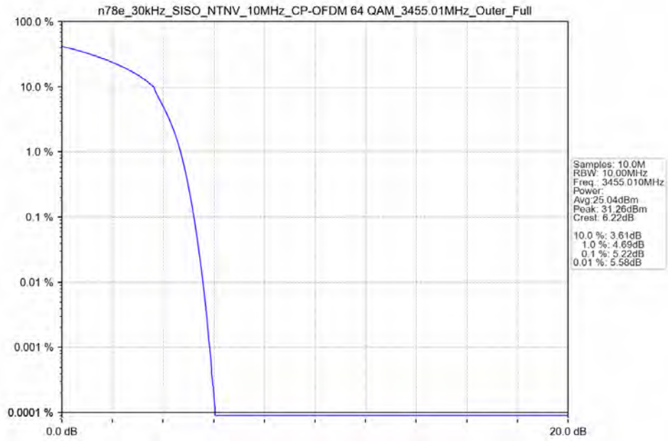
n78e_30kHz_SISO_NTNV_10MHz_CP-OFDM 64 QAM 3455.01MHz_Outer_Full_Ant13
