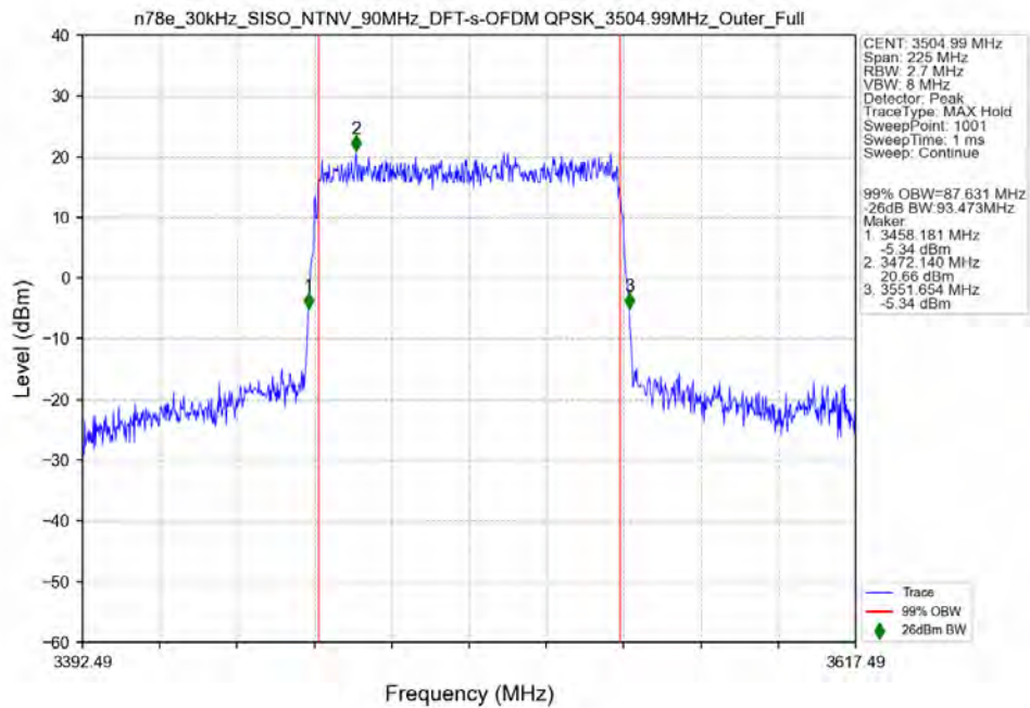
n78e_30kHz_SISO_NTNV_90MHz_DFT-s-OFDM_QPSK_3504.99MHz_Outer_Full_Ant13
