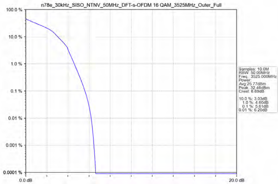
n78e_30kHz_SISO_NTNV_50MHz_DFT-s-OFDM_16_QAM_3525MHz_Outer_Full_Ant13
