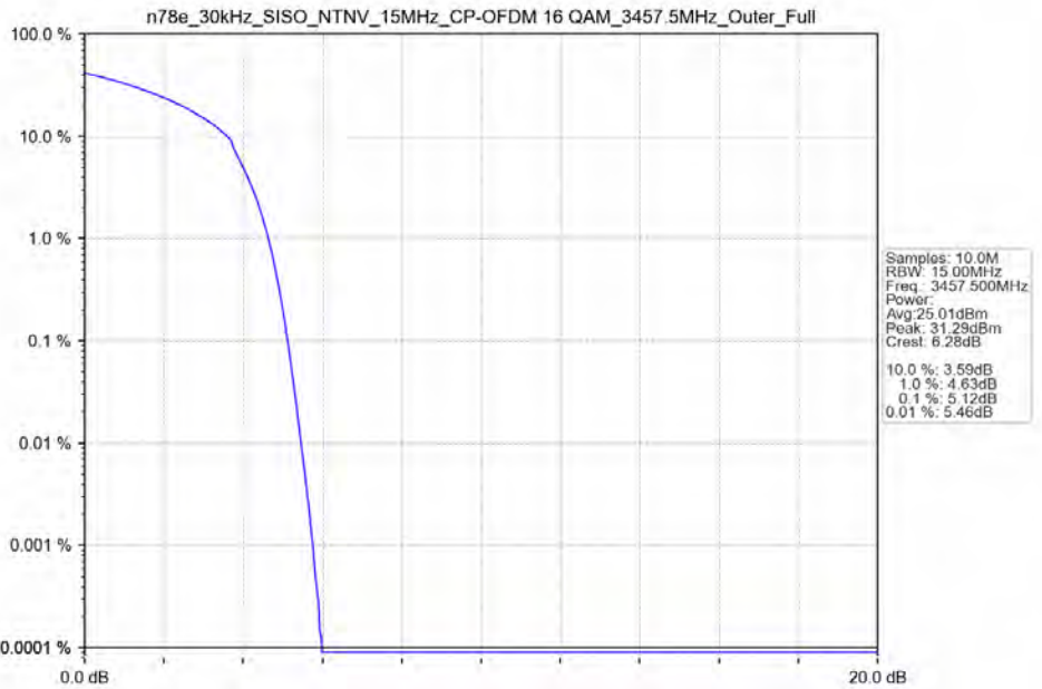
n78e 30kHz SISO NTN 15MHz CP-OFDM 16 QAM 3457.5MHz Outer Full Ant13
