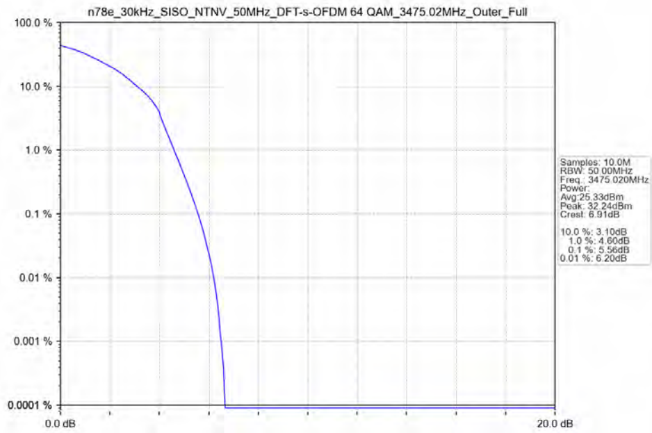
n78e_30kHz_SISO_NTNV_50MHz_DFT-s-OFDM_64_QAM_3475.02MHz_Outer_Full_Ant13
