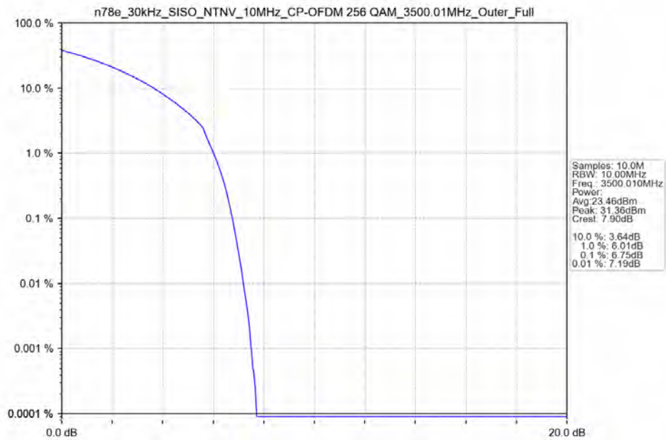
n78e 30kHz SISO NTN 10MHz CP-OFDM 256 QAM 3500.01MHz Outer Full Ant13
