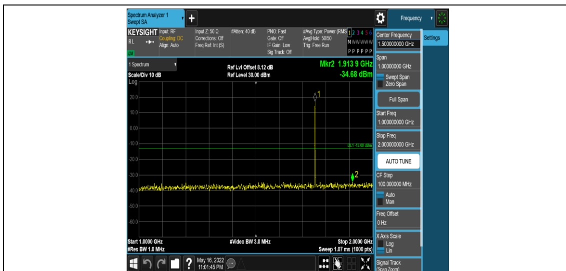
Band4-1.4MHz-16QAM-20393-1RB#0-Range4:1000~2000MHz
