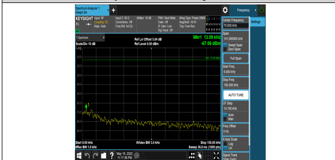
Band4-3MHz-16QAM-19965-1RB#0-Range1:0.009~0.15MHz
