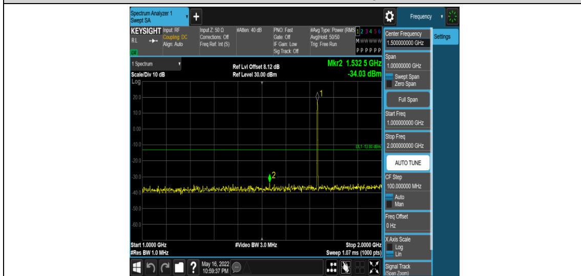
Band4-1.4MHz-16QAM-20175-1RB#0-Range4:1000~2000MHz
