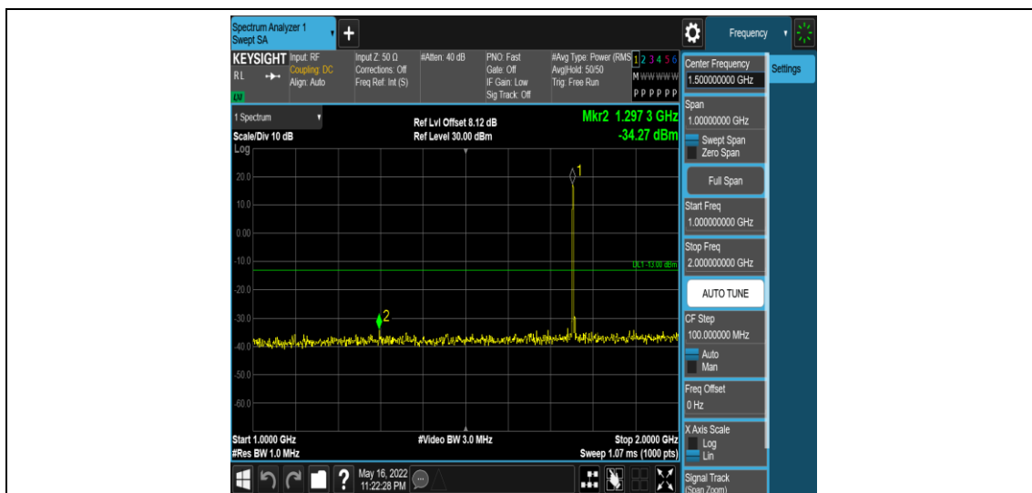
Band4-3MHz-16QAM-20385-1RB#0-Range4:1000~2000MHz
