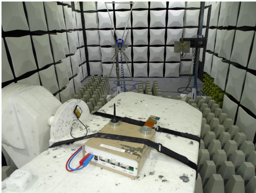
Photo 2: Test setup for radiated measurements above 1 GHz
