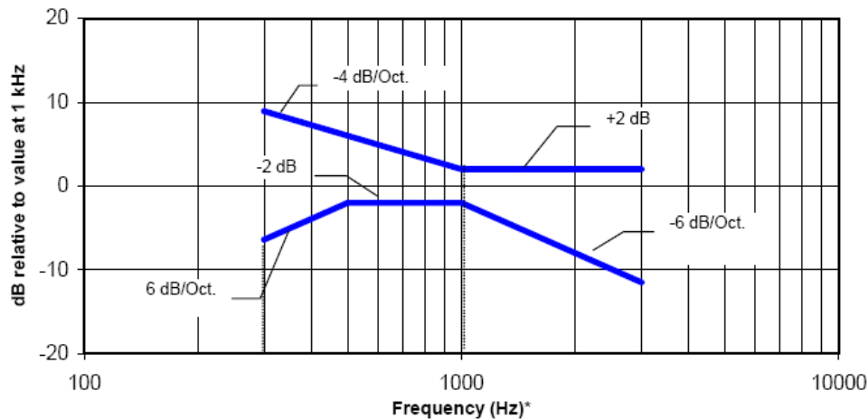
Figure 4 : Magnetic field frequency response for WDs with field strength -15 dB (A/m) at 1 kHz
