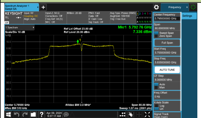
802.11ac-VHT80 Power Spectral Density - Ant 0
