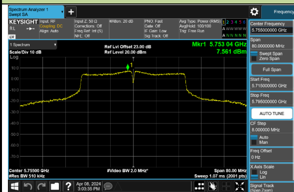
802.11ac-VHT80 Power Spectral Density - Ant 0
