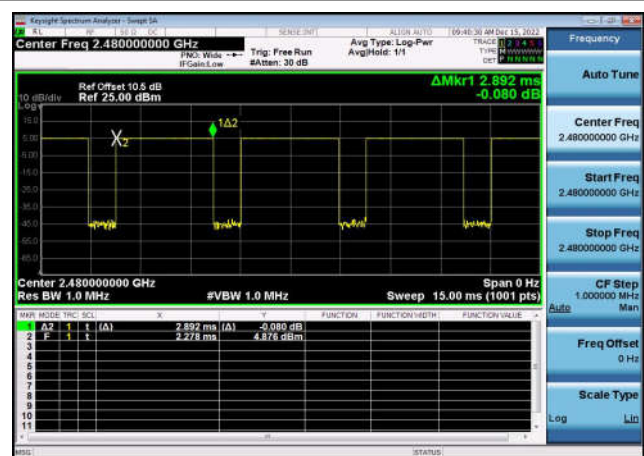
GFSK,2480,DH5,Transmission Time
