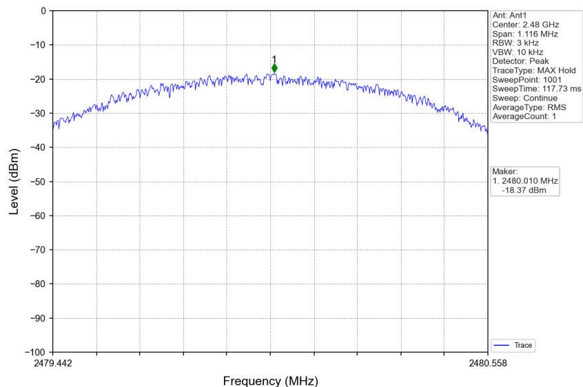
1M_HCH_2480MHz_DataRate= Ant1_NTNV
