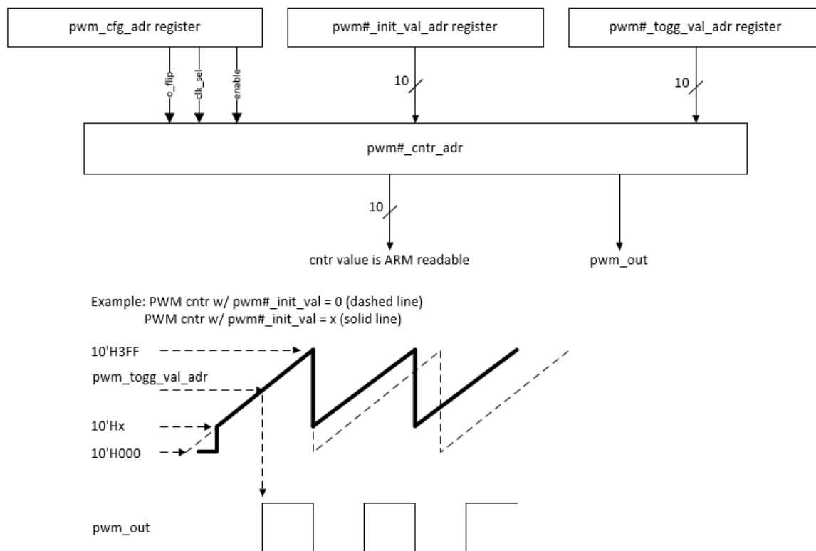
Figure 11. PWM Block Diagram
