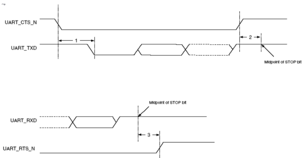
Figure 12. UART Timing
