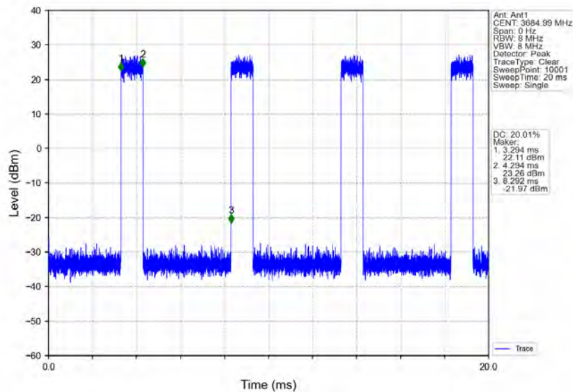
n78d_30kHz_MIMO_NTNV_30MHz_CP-OFDM 64 QAM_3684.99MHz_Inner_Full
