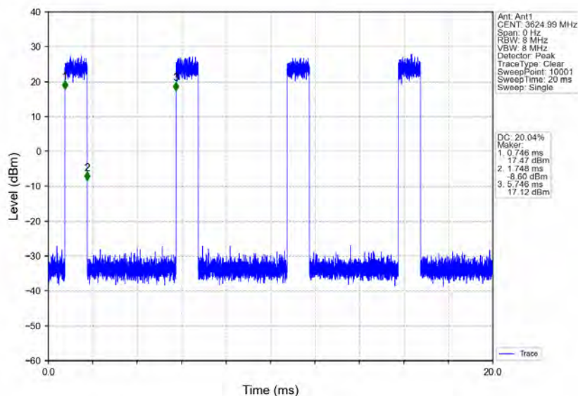
n78d_30kHz_MIMO_NTNV_30MHz_CP-OFDM 64 QAM_3624.99MHz_Inner_Full
