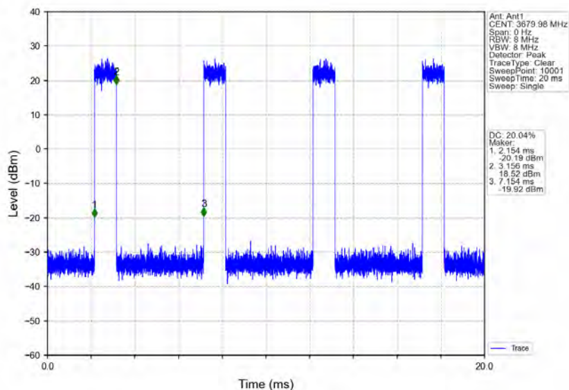
n78d_30kHz_MIMO_NTNV_40MHz_CP-OFDM 64 QAM_3679.98MHz_Inner_Full
