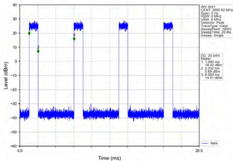
n78d_30kHz_MIMO_NTNV_40MHz_CP-OFDM_64_QAM_3570MHz_Inner_Full
