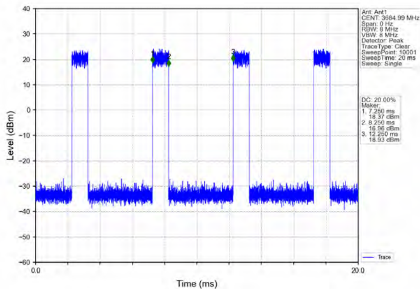
n78d_30kHz_MIMO_NTNV_30MHz_CP-OFDM_256_QAM_3684.99MHz_Inner_Full
