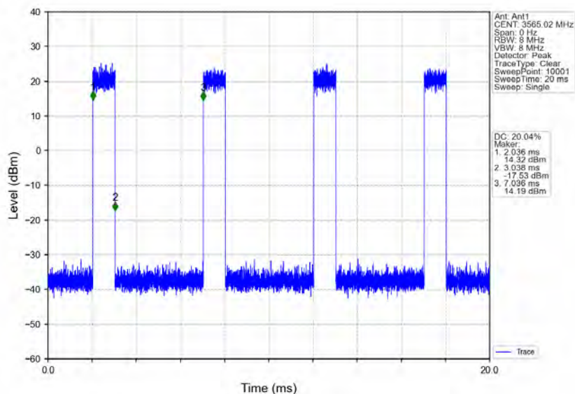
n78d_30kHz_MIMO_NTNV_30MHz_CP-OFDM_256_QAM_3565.02MHz_Inner_Full
