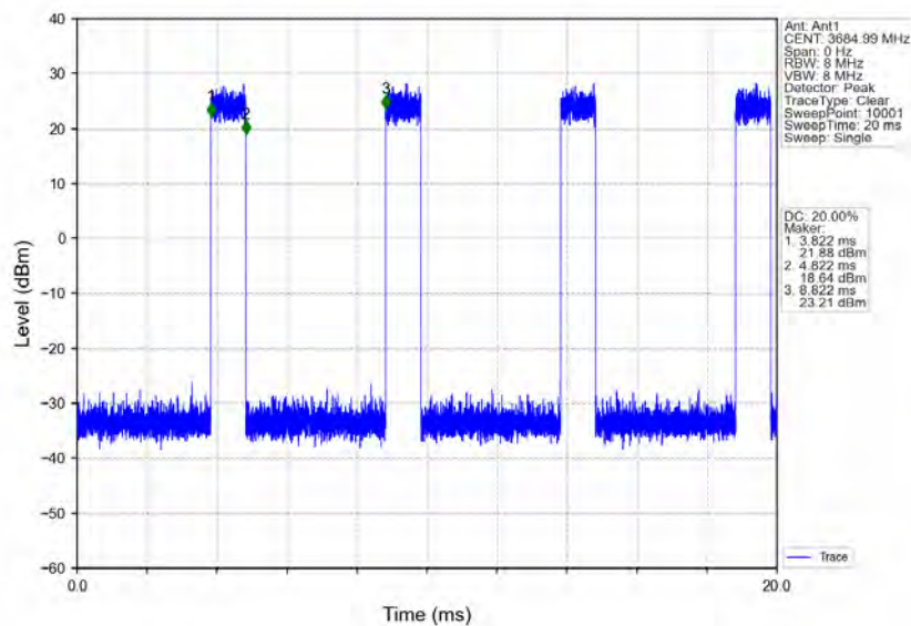
n78d_30kHz_MIMO_NTNV_30MHz_CP-OFDM_QPSK_3684.99MHz_Inner_Full
