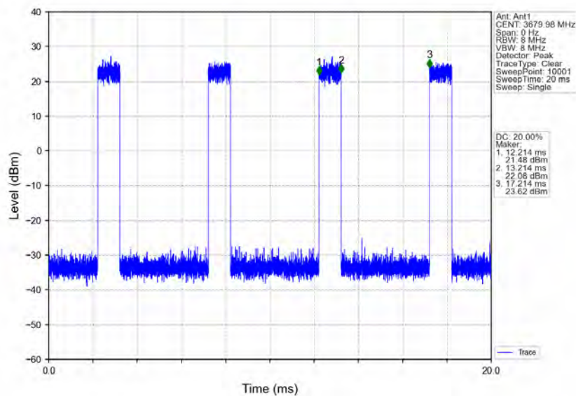
n78d_30kHz_MIMO_NTNV_40MHz_CP-OFDM_16_QAM_3679.98MHz_Inner_Full
