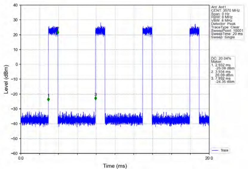
n78d_30kHz_MIMO_NTNV_40MHz_CP-OFDM_QPSK_3570MHz_Inner_Full
