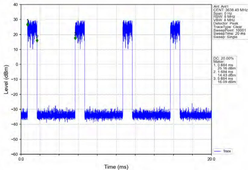
n78d_30kHz_MIMO_NTNV_30MHz_CP-OFDM 64 QAM_3624.99MHz_Inner_1RB_Right
