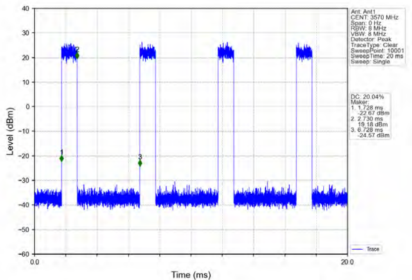
n78d_30kHz_MIMO_NTNV_40MHz_CP-OFDM_64_QAM_3570MHz_Inner_Full
