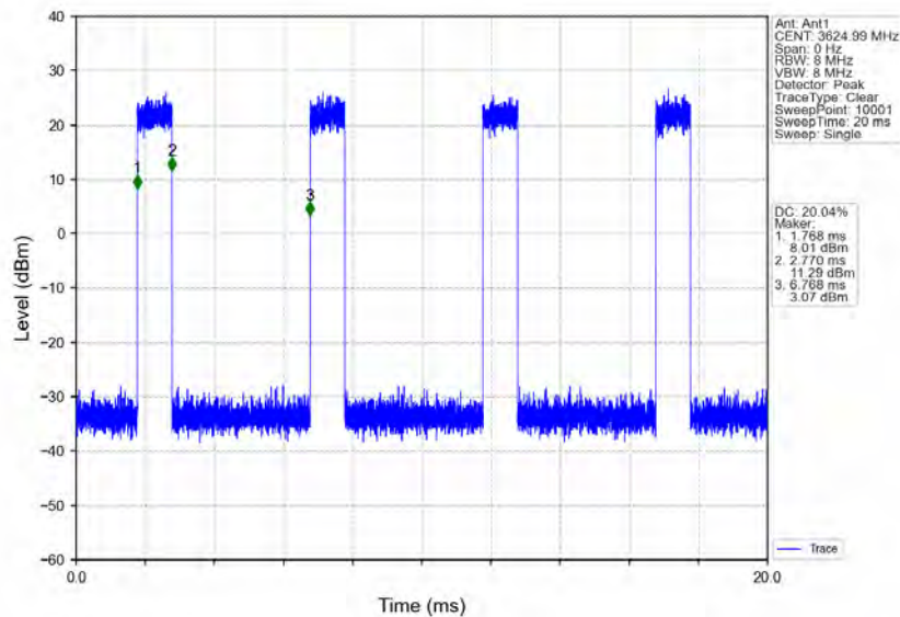
n78d_30kHz_MIMO_NTNV_50MHz_CP-OFDM_QPSK_3624.99MHz_Inner_Full
