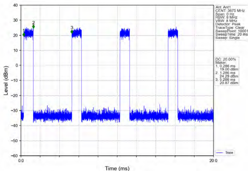
n78d_30kHz_MIMO_NTNV_50MHz_CP-OFDM_QPSK_3675MHz_Inner_Full
