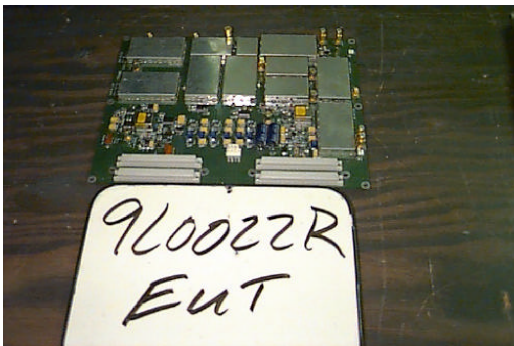
Photo 11 - Motherboard top with shields
