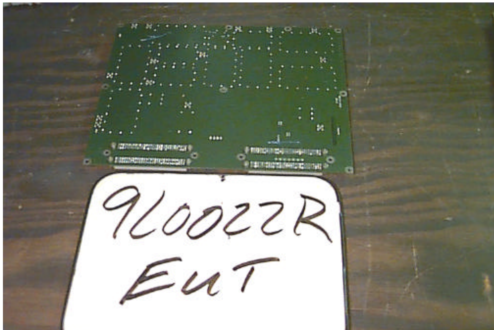
Photo 13 - Motherboard bottom
