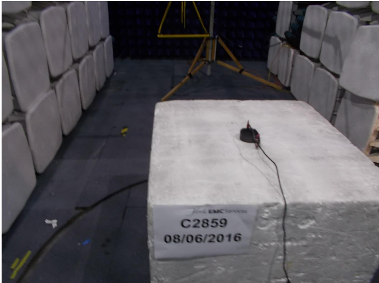
Photograph 3 Radiated Electric Field Preliminary Measurements 30MHz to 1GHz
