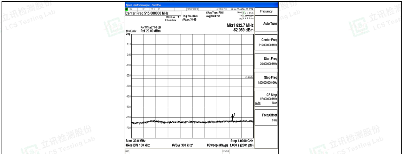
Band66_20MHz_QPSK_132572_1RB#0_30~1000_30~1000
