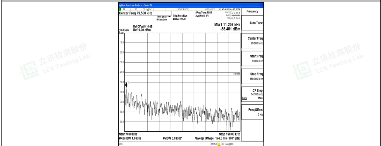
Band66_20MHz_16QAM_132322_1RB#0_0.009~0.15_0.009~0.15
