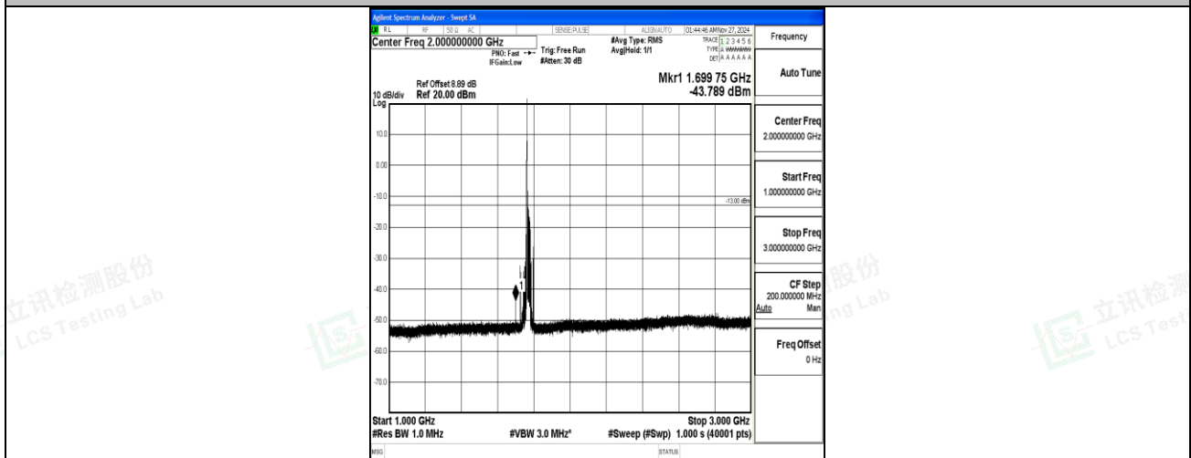
Band66_20MHz_QPSK_132572_1RB#0_1000~3000_1000~3000
