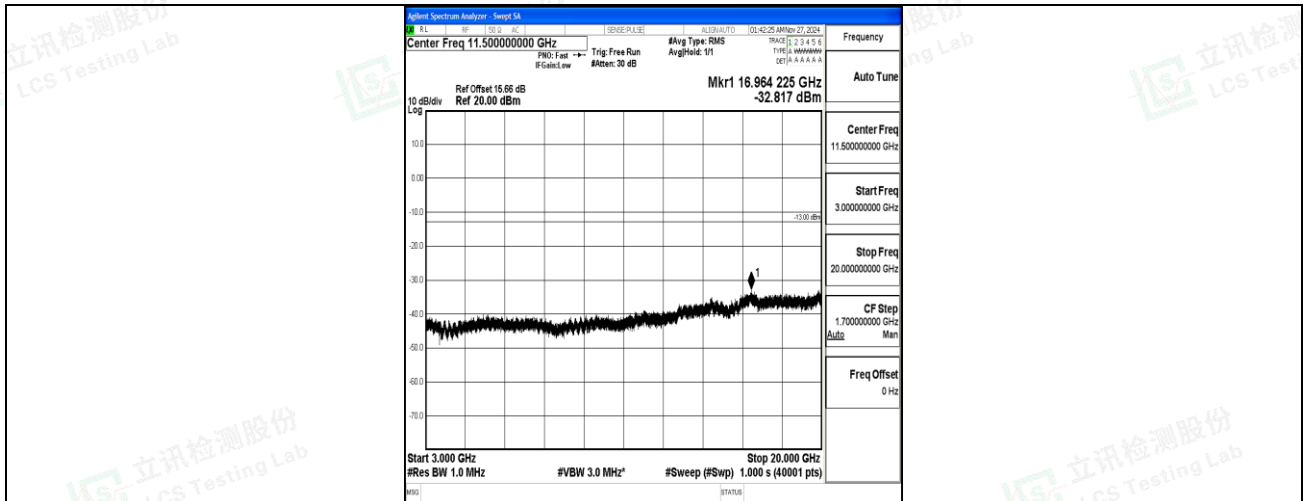
Band66_20MHz_QPSK_132072_1RB#0_3000~20000_3000~20000
