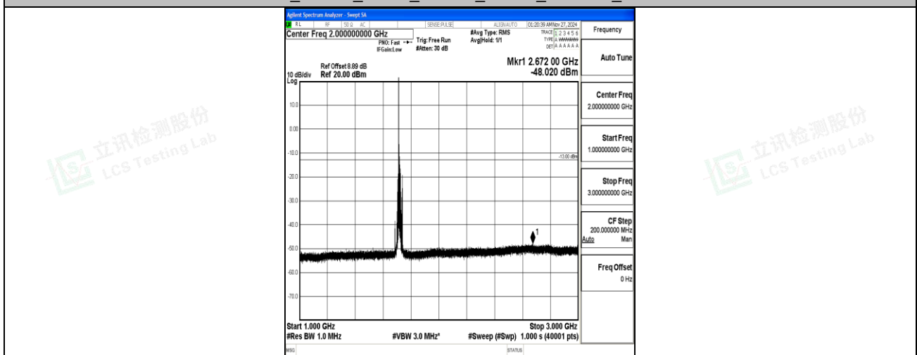
Band66_15MHz_QPSK_132047_1RB#0_1000~3000_1000~3000
