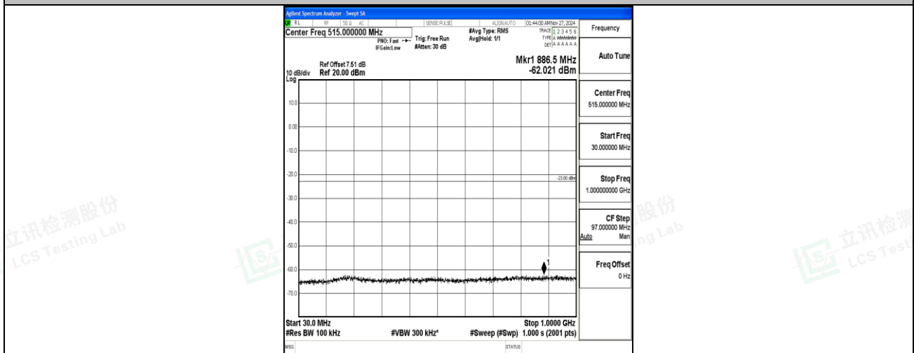
Band66_20MHz_16QAM_132322_1RB#0_30~1000_30~1000
