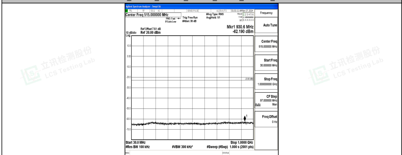
Band66_10MHz_16QAM_132622_1RB#0_30~1000_30~1000
