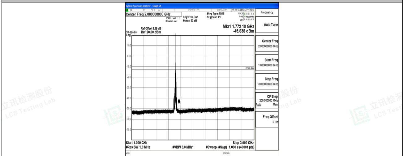
Band66_15MHz_16QAM_132047_1RB#0_1000~3000_1000~3000
