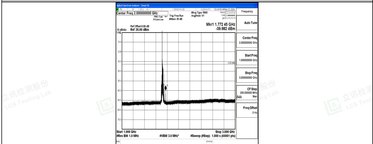
Band66_20MHz_16QAM_132072_1RB#0_1000~3000_1000~3000
