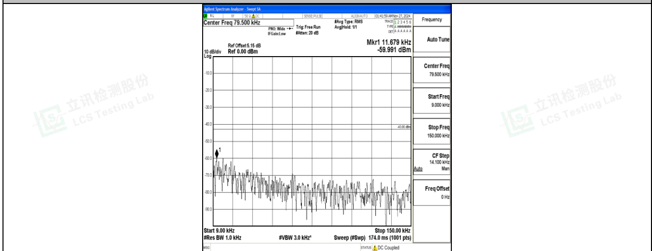
Band66_20MHz_QPSK_132072_1RB#0_0.009~0.15_0.009~0.15
