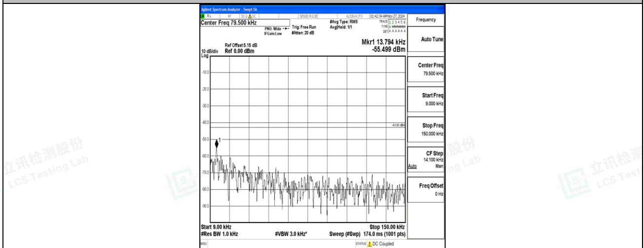
Band66_20MHz_16QAM_132072_1RB#0_0.009~0.15_0.009~0.15
