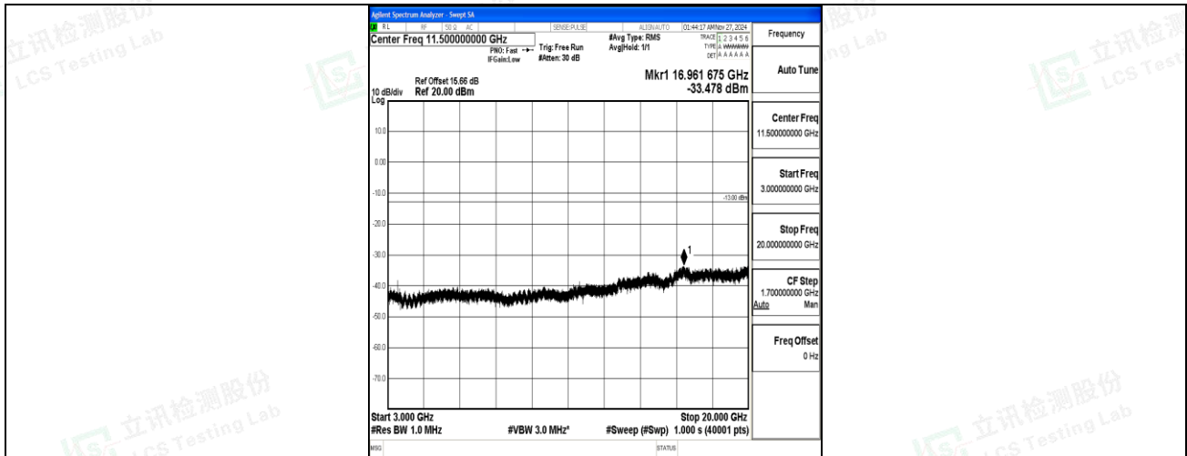
Band66_20MHz_16QAM_132322_1RB#0_3000~20000_3000~20000
