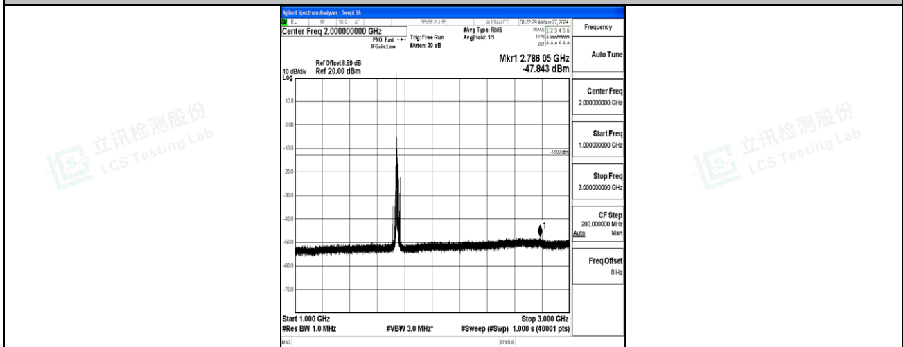
Band66_15MHz_16QAM_132322_1RB#0_1000~3000_1000~3000
