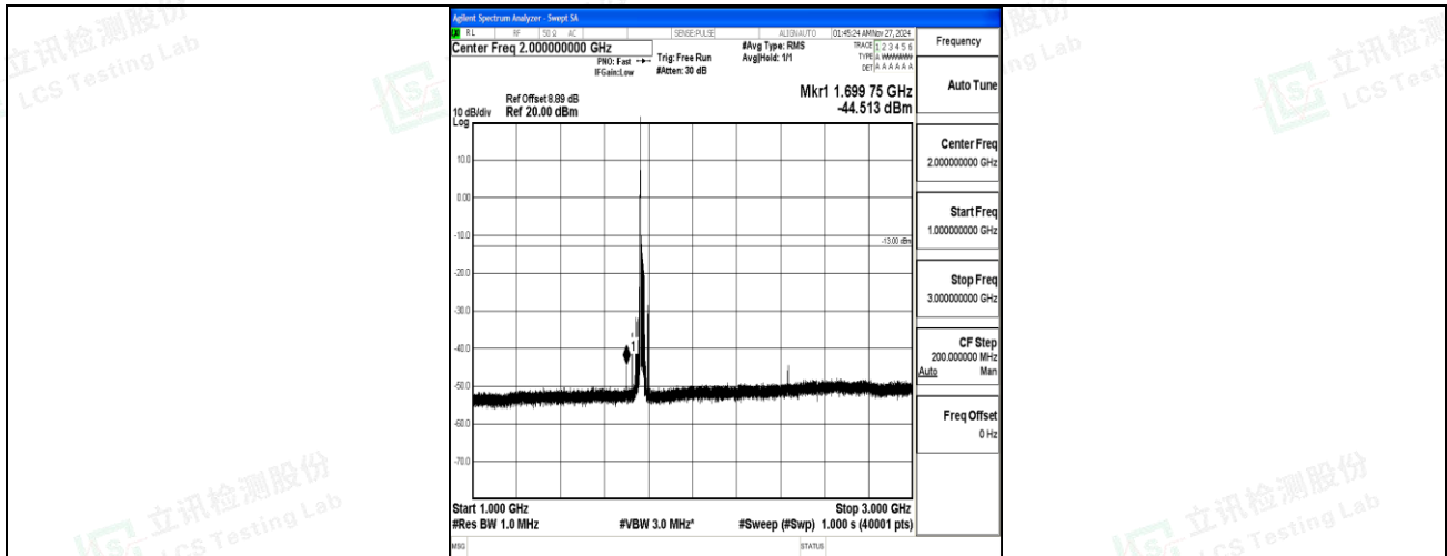
Band66_20MHz_16QAM_132572_1RB#0_1000~3000_1000~3000
