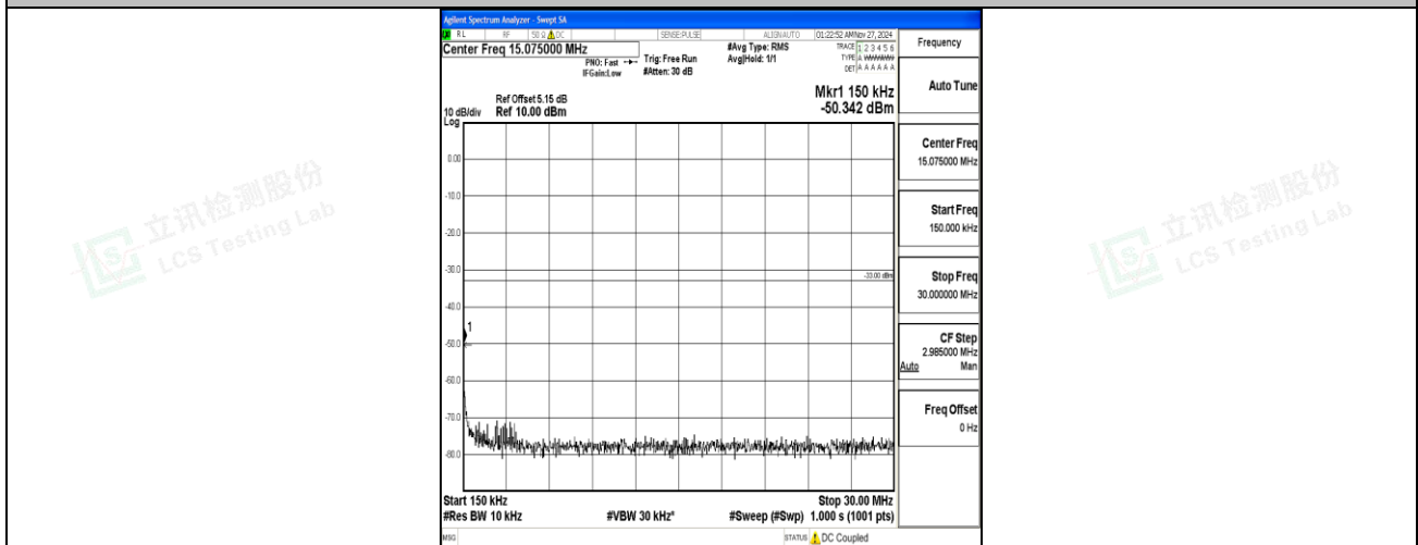
Band66_15MHz_QPSK_132597_1RB#0_0.15~30_0.15~30
