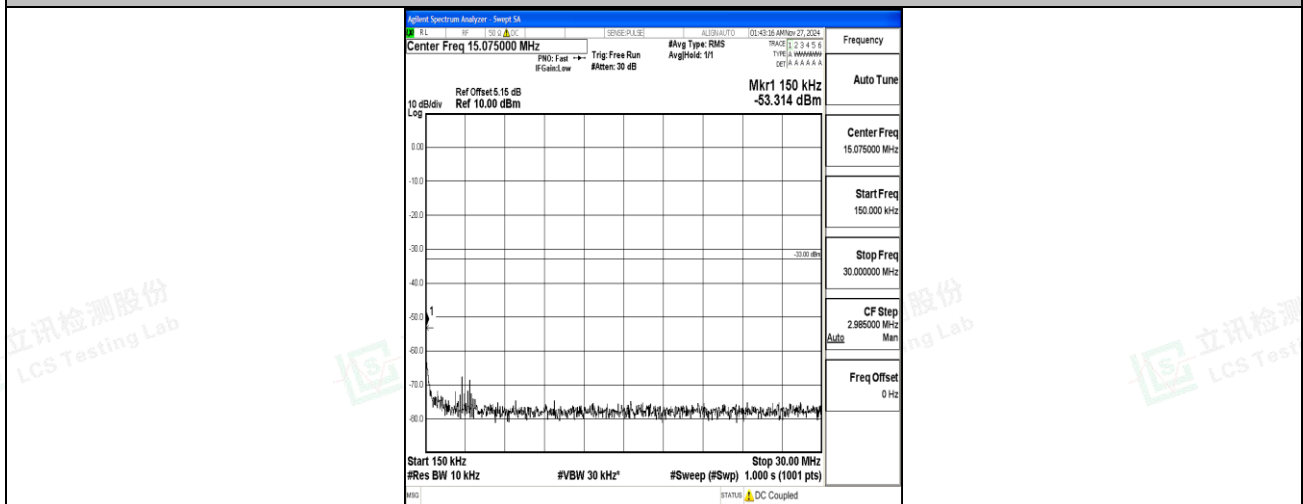
Band66_20MHz_QPSK_132322_1RB#0_0.15~30_0.15~30
