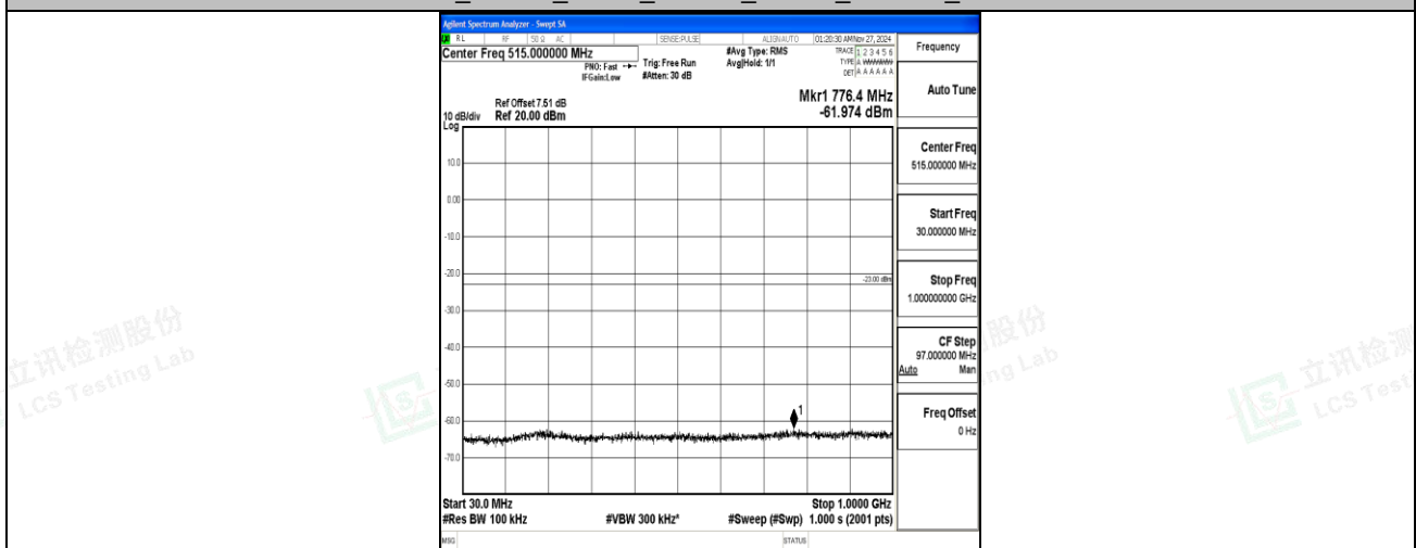
Band66_15MHz_QPSK_132047_1RB#0_30~1000_30~1000
