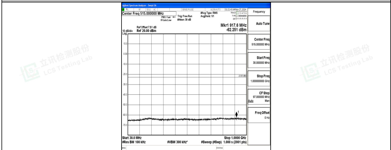
Band66_15MHz_QPSK_132322_1RB#0_30~1000_30~1000
