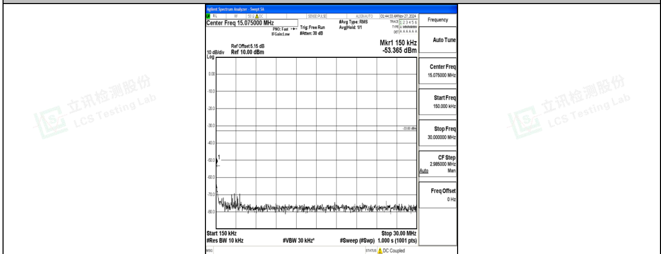
Band66_20MHz_QPSK_132572_1RB#0_0.15~30_0.15~30
