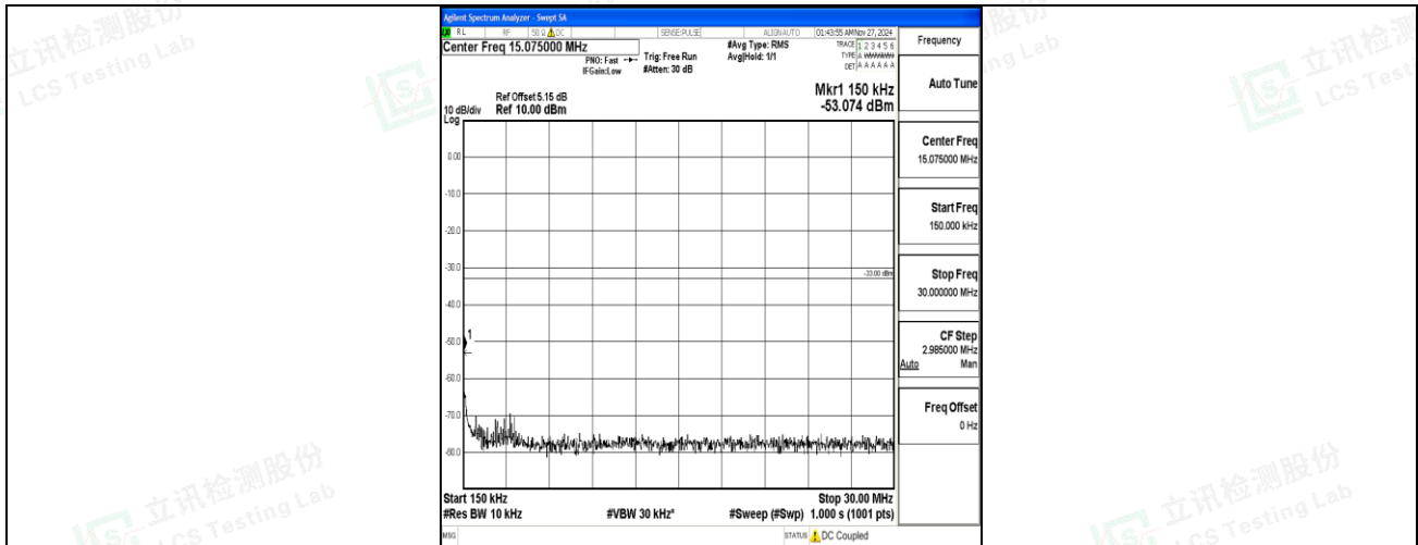
Band66_20MHz_16QAM_132322_1RB#0_0.15~30_0.15~30
