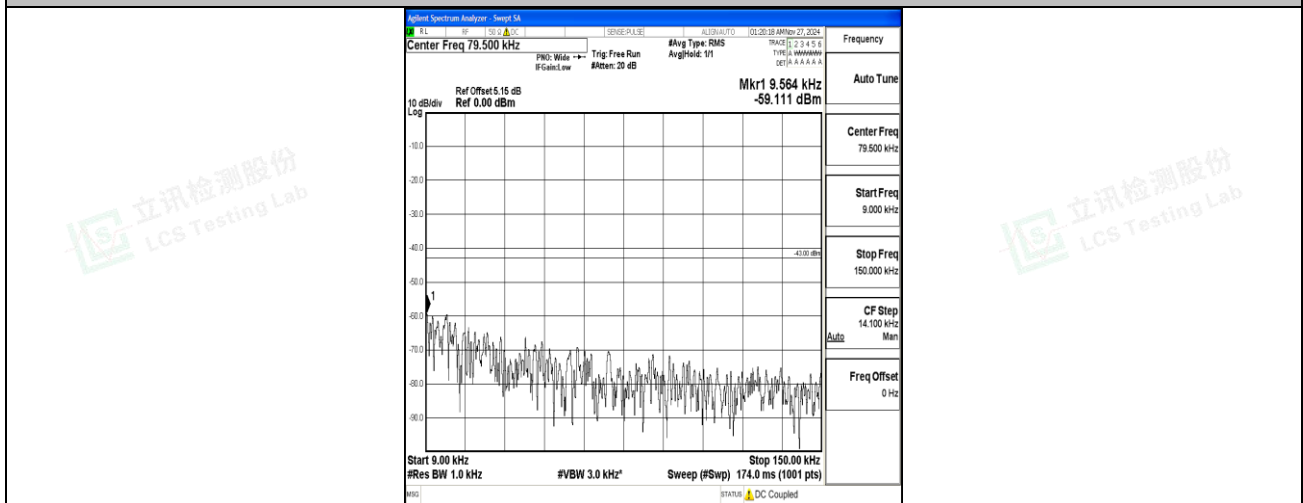
Band66_15MHz_QPSK_132047_1RB#0_0.009~0.15_0.009~0.15
