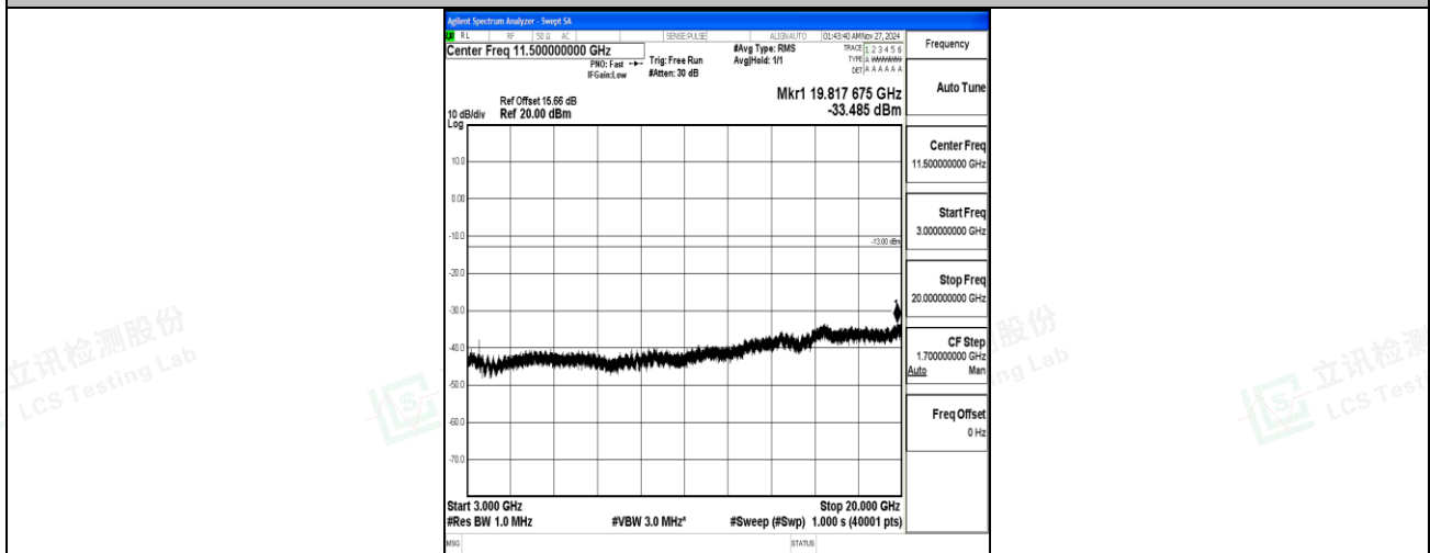
Band66_20MHz_QPSK_132322_1RB#0_3000~20000_3000~20000
