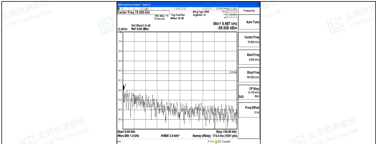
Band66_20MHz_16QAM_132572_1RB#0_0.009~0.15_0.009~0.15
