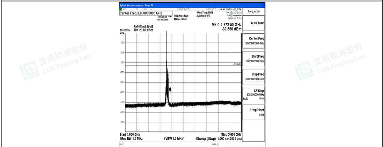
Band66_20MHz_QPSK_132072_1RB#0_1000~3000_1000~3000
