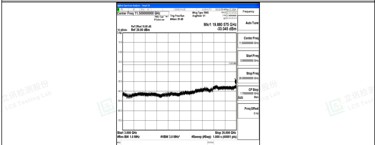
Band66_15MHz_QPSK_132322_1RB#0_3000~20000_3000~20000
