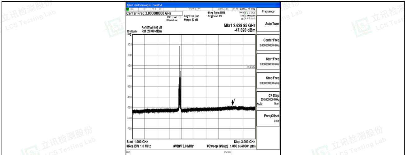
Band66_10MHz_16QAM_132622_1RB#0_1000~3000_1000~3000
