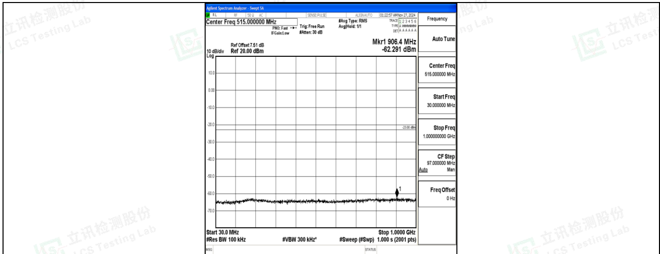
Band66_15MHz_QPSK_132597_1RB#0_30~1000_30~1000
