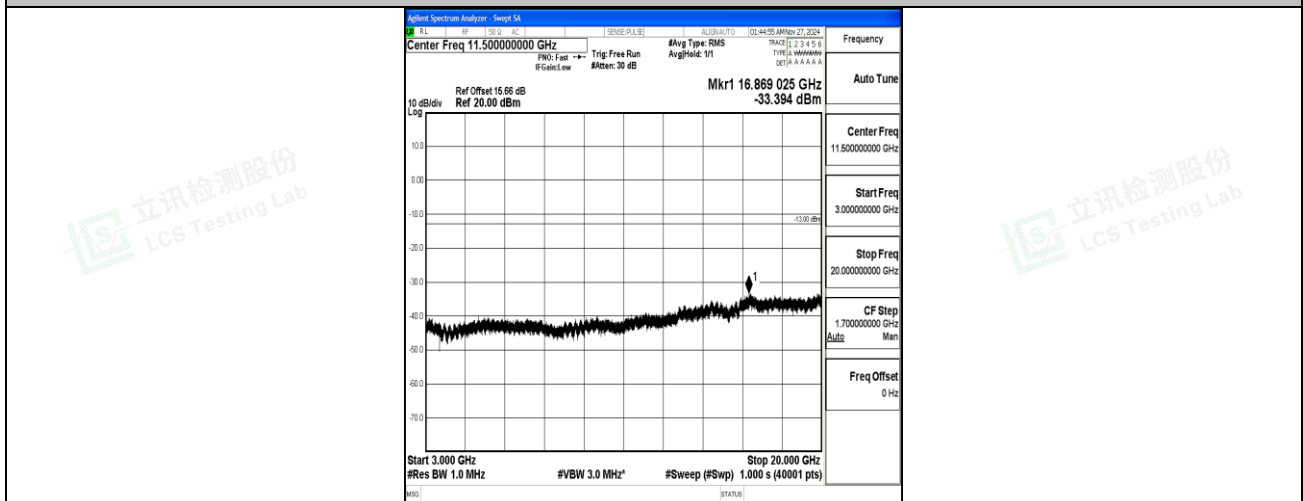
Band66_20MHz_QPSK_132572_1RB#0_3000~20000_3000~20000
