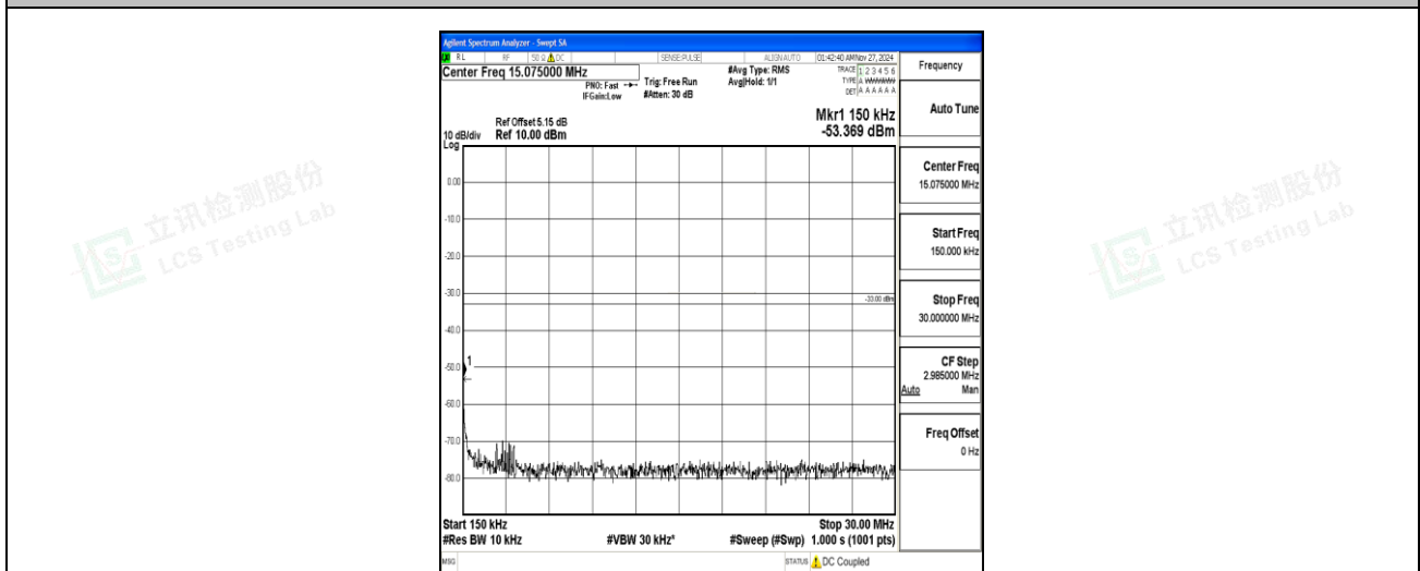
Band66_20MHz_16QAM_132072_1RB#0_0.15~30_0.15~30
