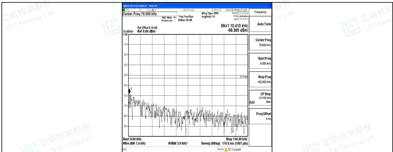
Band66_10MHz_16QAM_132622_1RB#0_0.009~0.15_0.009~0.15
