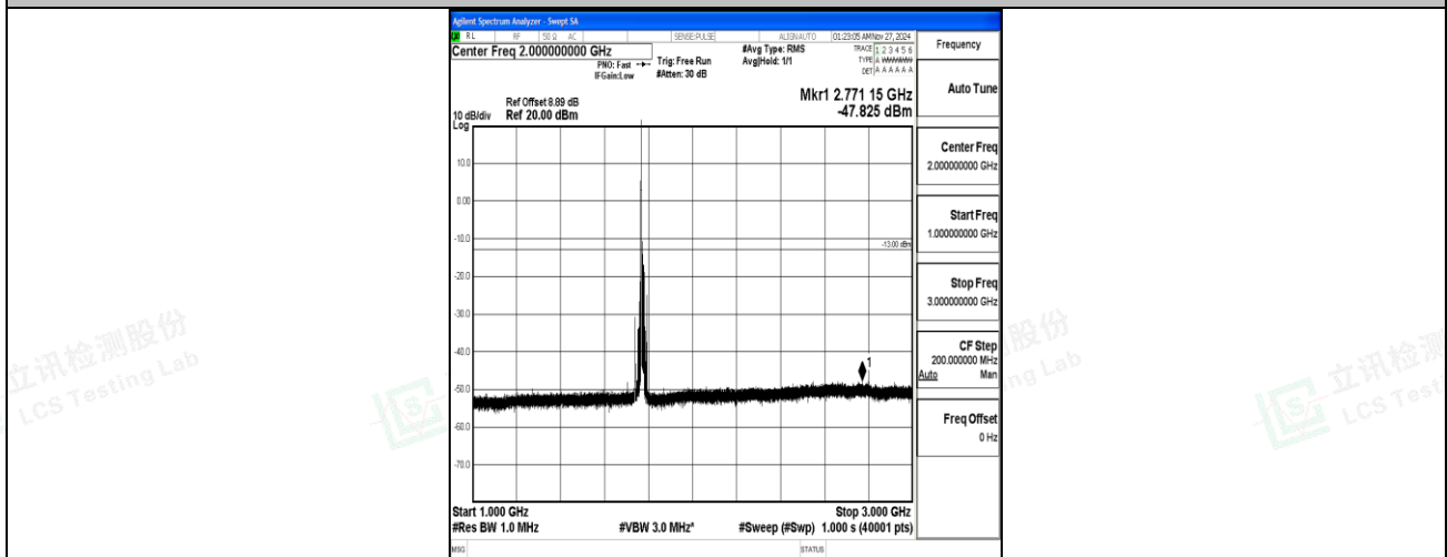
Band66_15MHz_QPSK_132597_1RB#0_1000~3000_1000~3000
