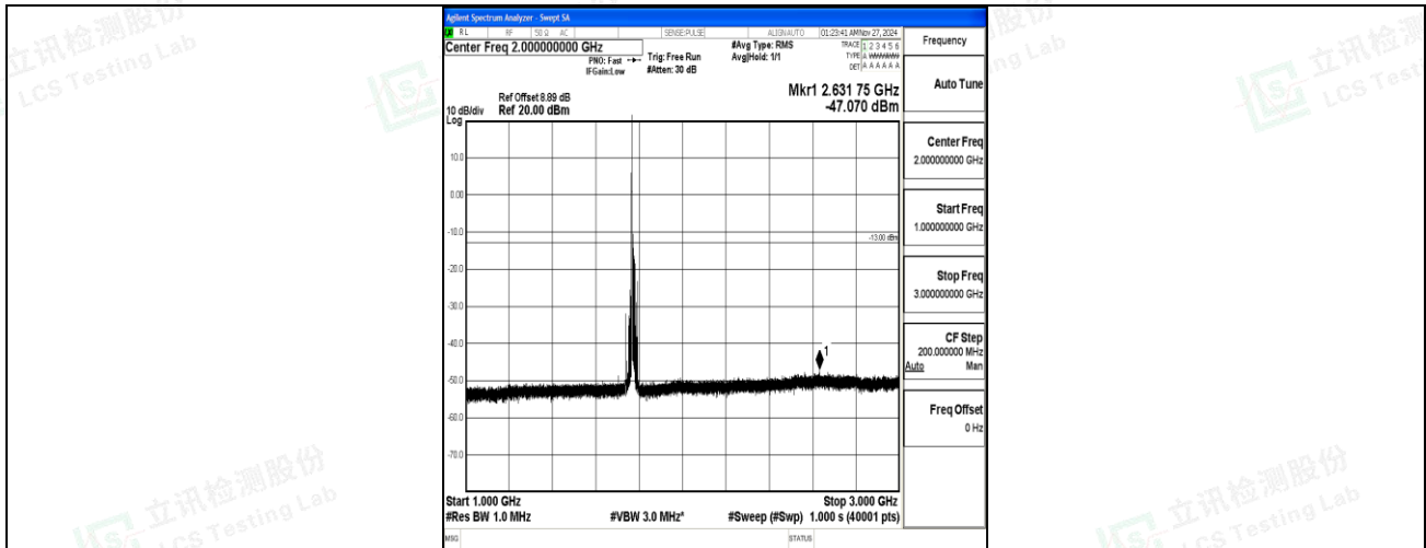
Band66_15MHz_16QAM_132597_1RB#0_1000~3000_1000~3000
