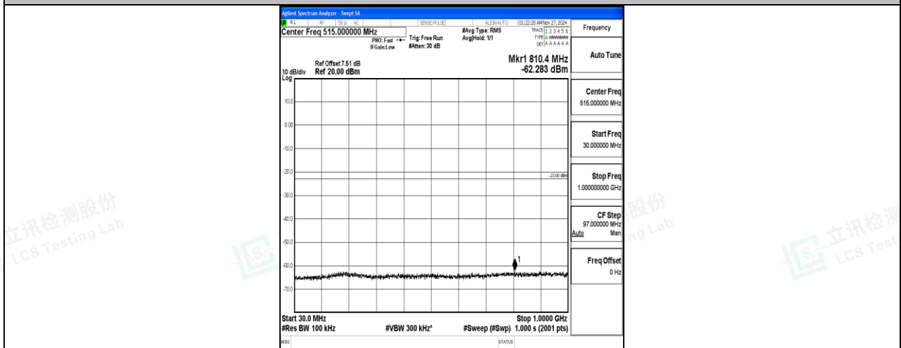
Band66_15MHz_16QAM_132322_1RB#0_30~1000_30~1000
