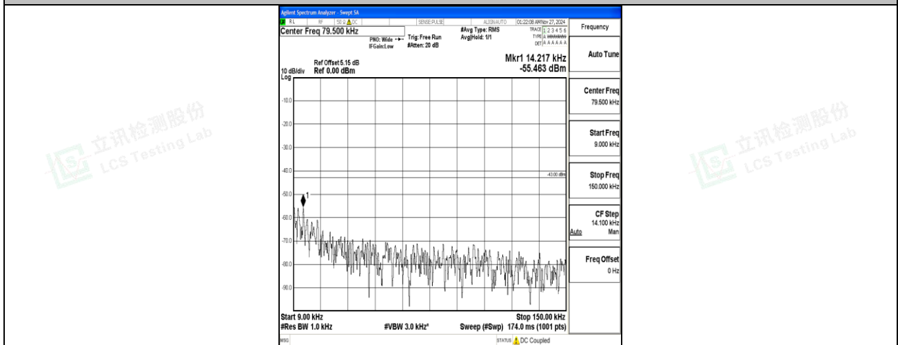
Band66_15MHz_16QAM_132322_1RB#0_0.009~0.15_0.009~0.15
