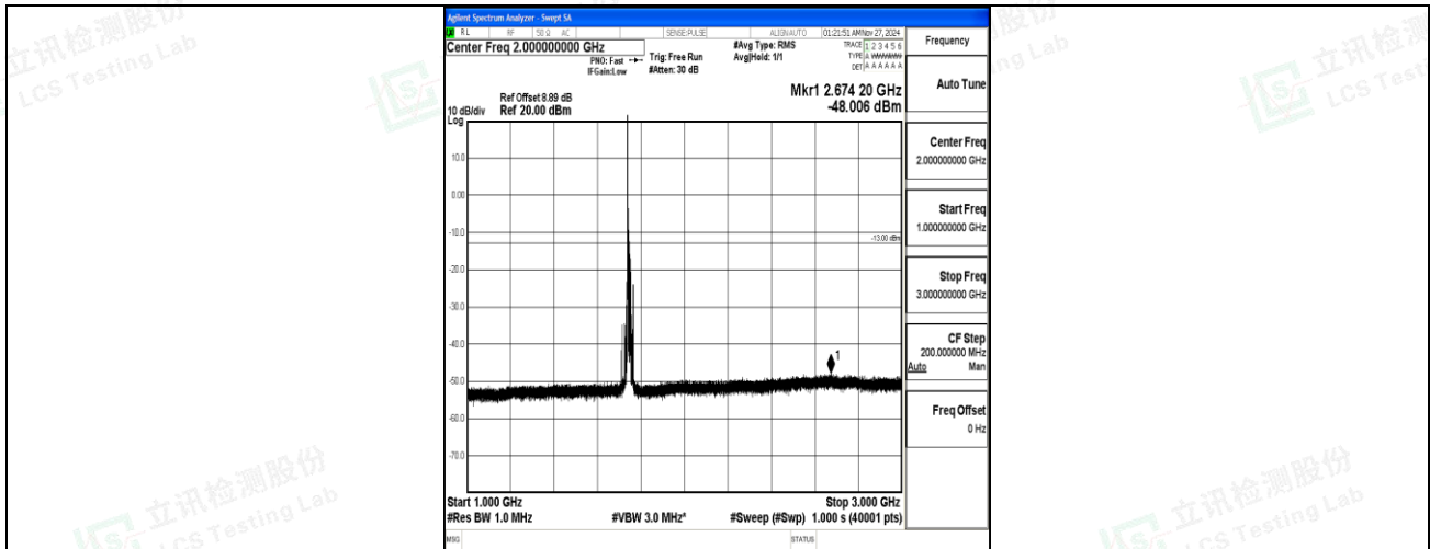
Band66_15MHz_QPSK_132322_1RB#0_1000~3000_1000~3000
