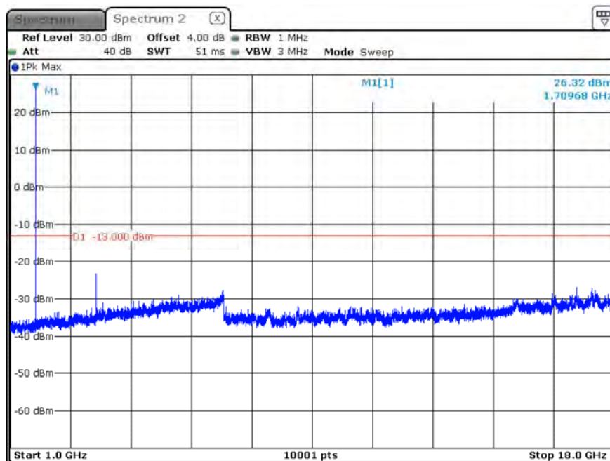
B4_CH19957_1.4M_1RB0_QPSK_Above 1G
