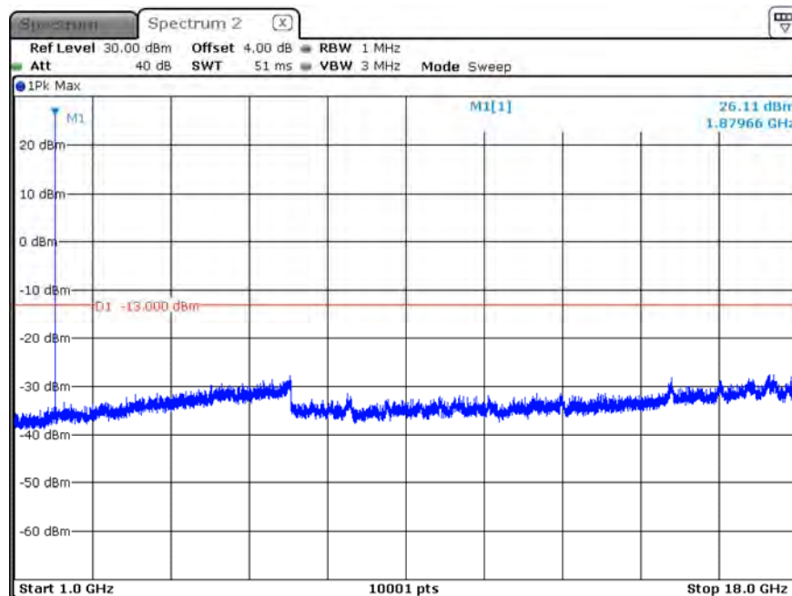
B2_CH18900_1.4M_1RB0_16-QAM_Above 1G
