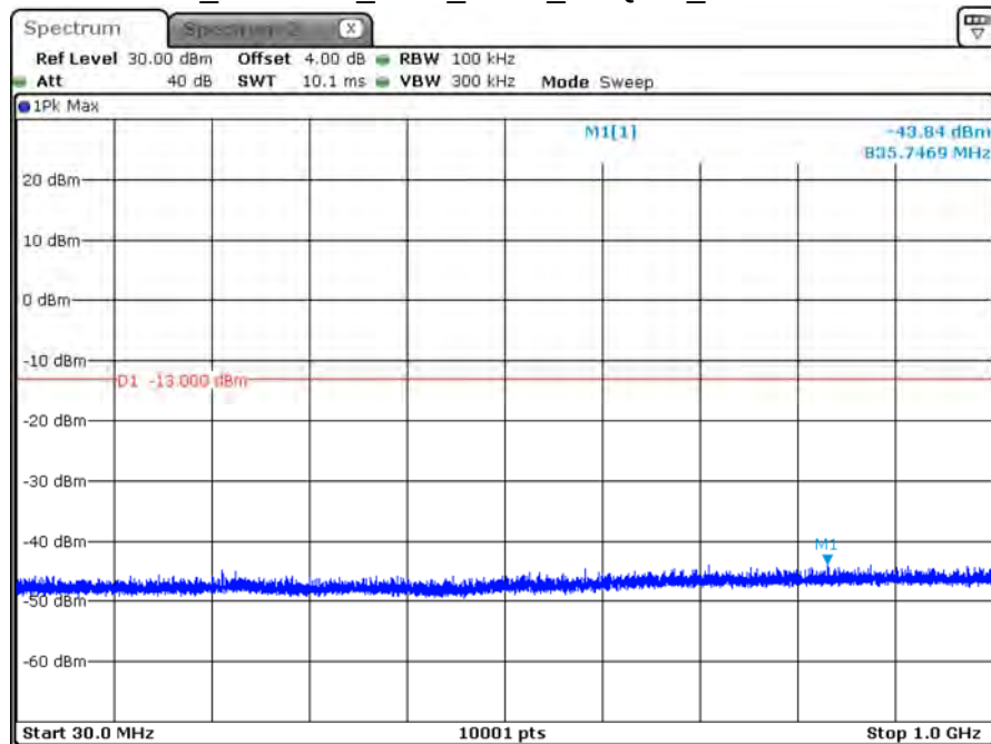
B2_CH18900_1.4M_1RB0_16-QAM_Below 1G
