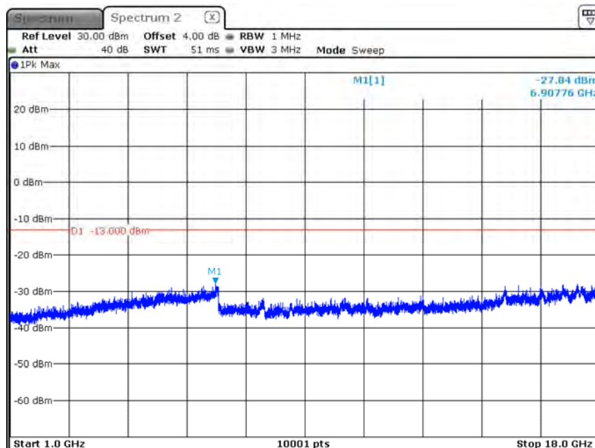
B5_CH20525_1.4M_1RB0_16-QAM_Above 1G
