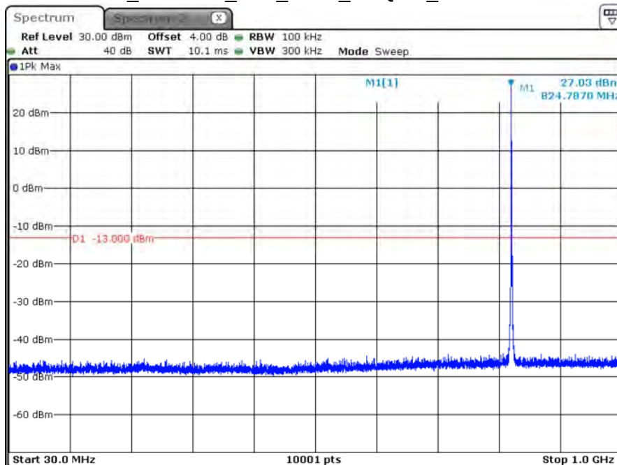
B5_CH20450_10M_1RB0_16-QAM_Below 1G
