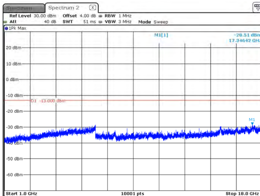
B5_CH20450_10M_1RB0_16-QAM_Above 1G
