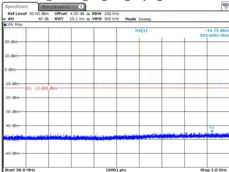
B4_CH20000_10M_1RB0_16-QAM_Below 1G
