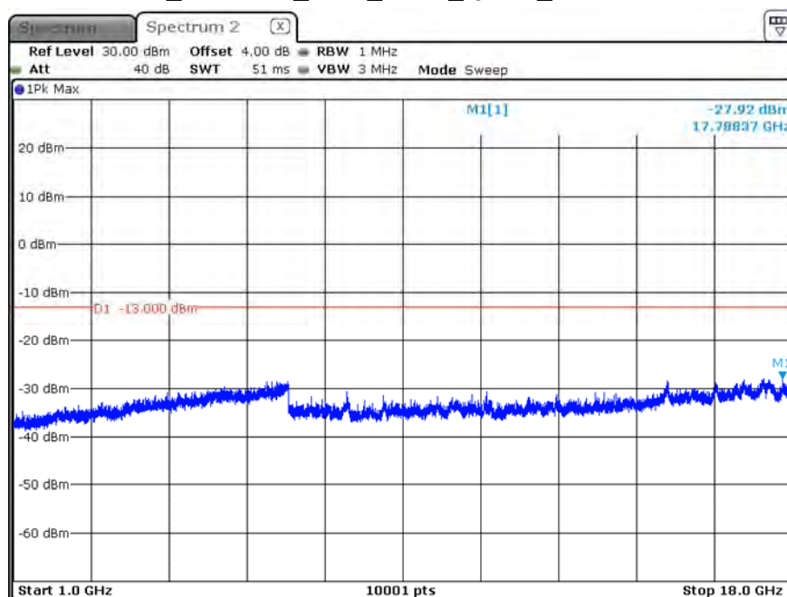
B5_CH20407_1.4M_1RB0_QPSK_Above 1G
