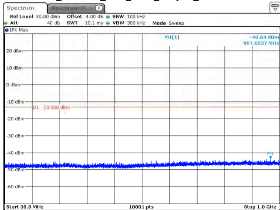
B4_CH19957_1.4M_1RB0_16-QAM_Below 1G
