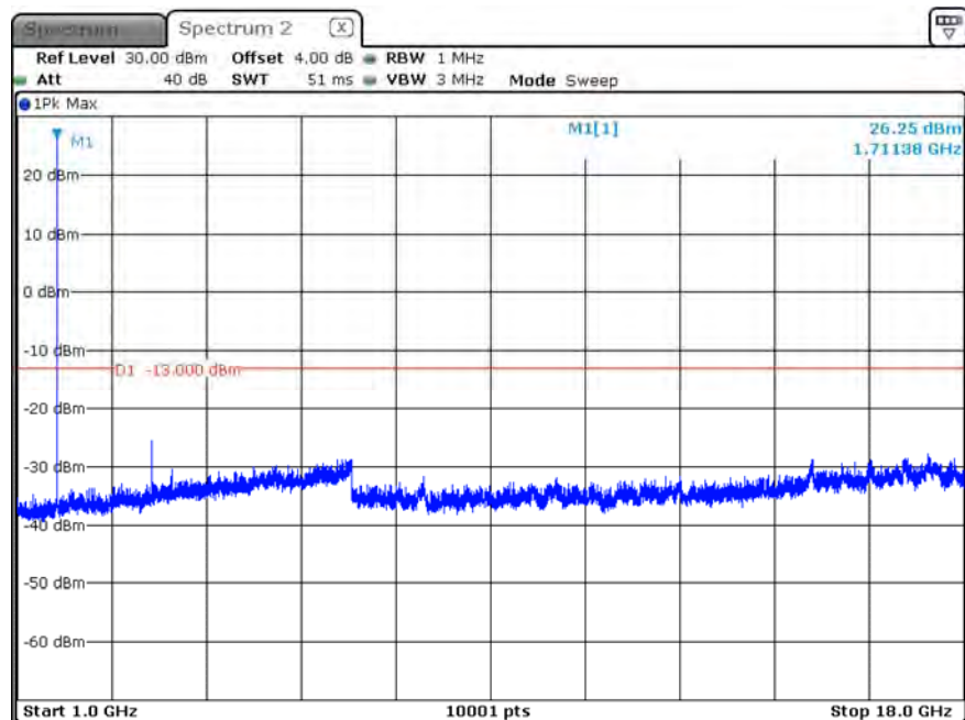
B4_CH19957_1.4M_1RB0_16-QAM_Above 1G
