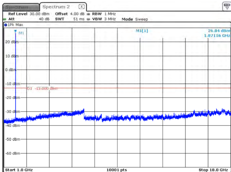
B2_CH18900_20M_1RB0_16-QAM_Above 1G
