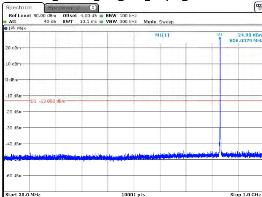
B5_CH20525_1.4M_1RB0_16-QAM_Below 1G
