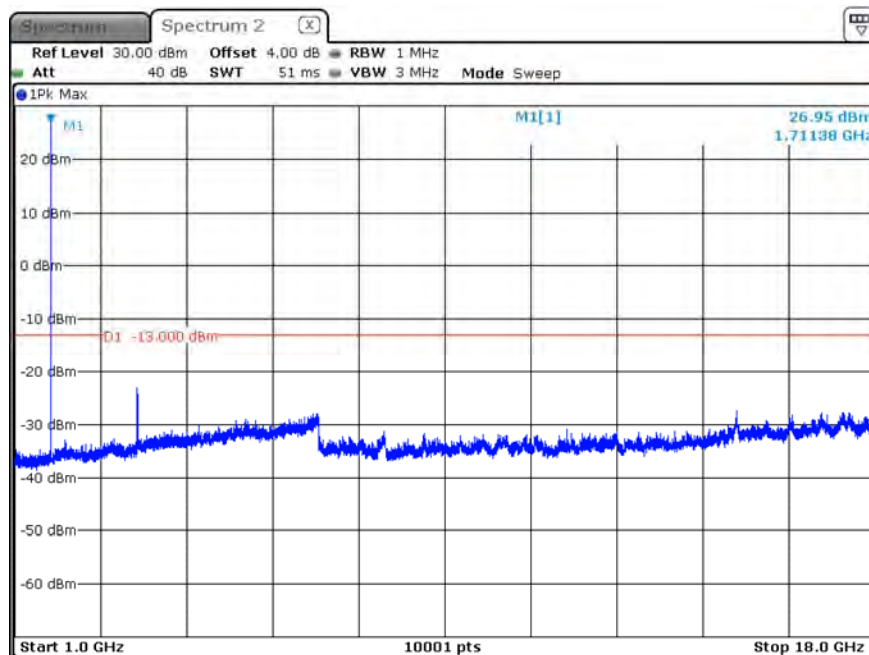
B4_CH20000_10M_1RB0_16-QAM_Above 1G
