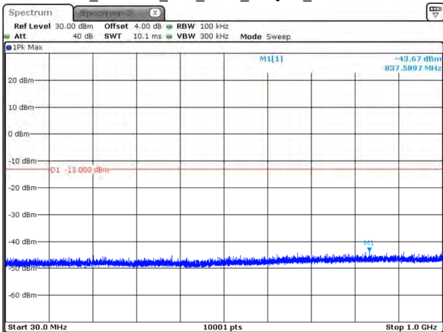
B2_CH18900_20M_1RB0_16-QAM_Below 1G
