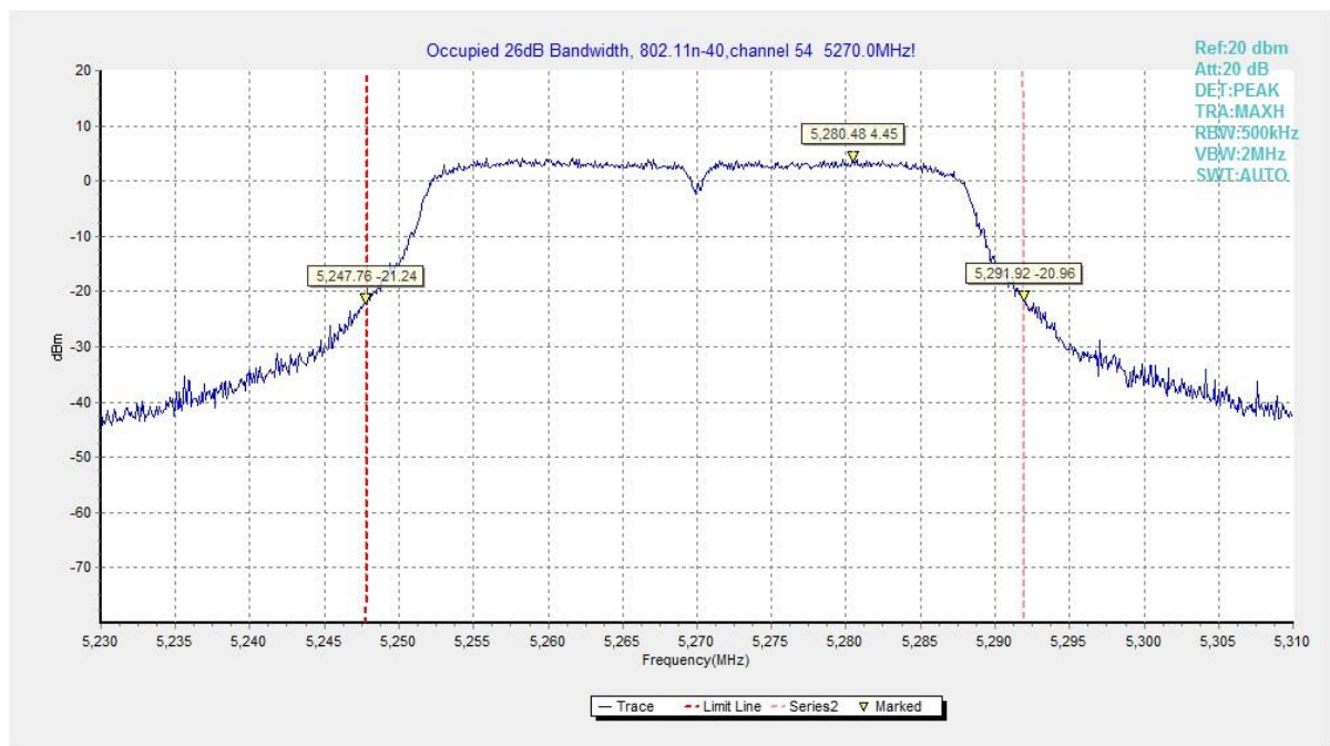
Fig. 21 Occupied 26dB Bandwidth (802.11n40, 5270MHz)
