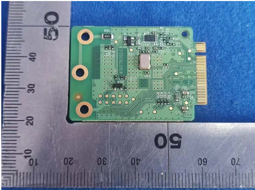
FIGURE 4 WIRELESS MODULE (MTxP250303ANT1) MAINBOARD BACK
