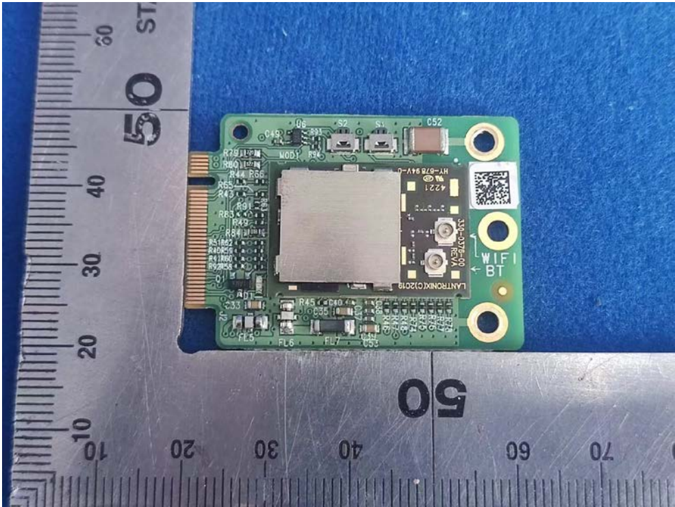
FIGURE 3 WIRELESS MODULE (MTxP250303ANT1) MAINBOARD FRONT
