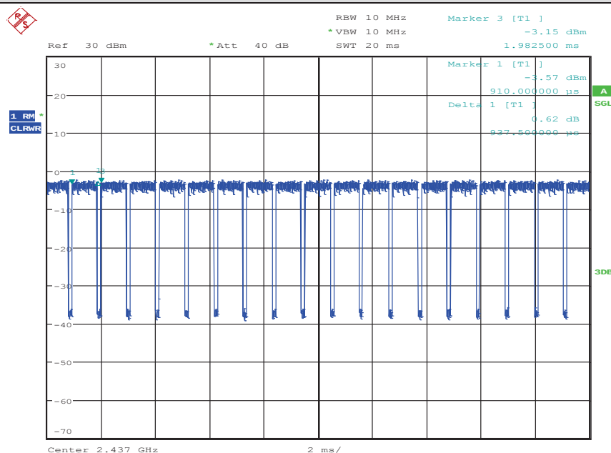
Test Graph_IEEE802.11 n (HT40) Duty Cycle:
