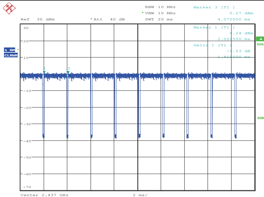
Test Graph_IEEE802.11 n (HT20) Duty Cycle:
