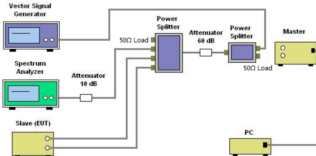
Radarsignal 0
