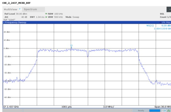
Figure 8.2-21: Conducted power spectral density reference level, 802.11n, MCS0, 2437 MHz
