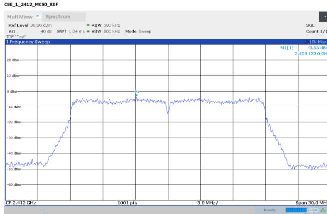
Figure 8.2-19: Conducted power spectral density reference level, 802.11n, MCS0, 2412 MHz
