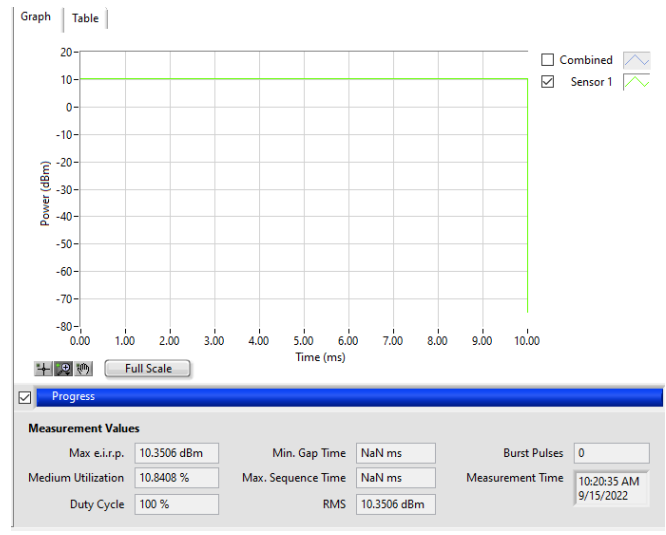
Figure 8.1-6: Conducted output power, 802.11g, 6 Mbps, 2462 MHz
