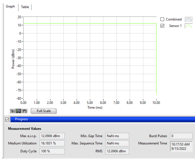
Figure 8.1-2: Conducted output power, 802.11b, 1 Mbps, 2440 MHz
