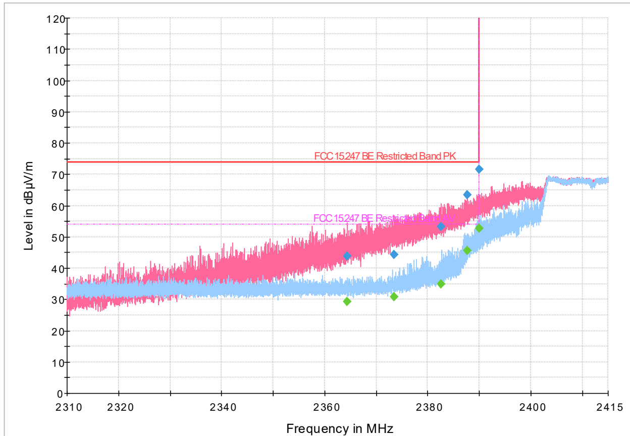
Figure 8.2-25: Radiated emissions spectral plot (2.31 GHz - 2.415 GHz), 802.11n, MCS0
