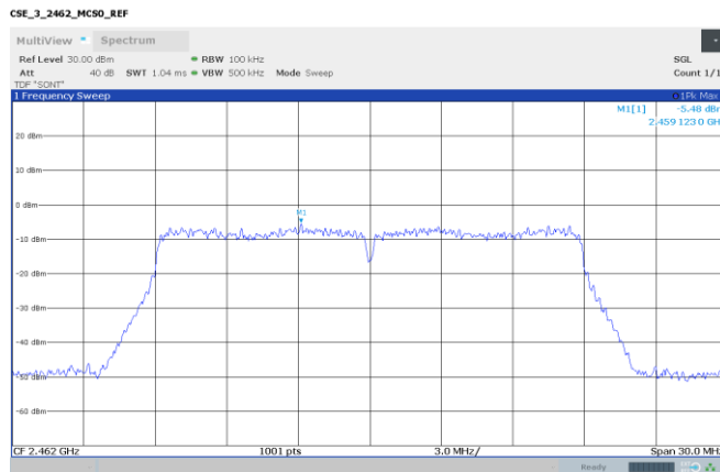
Figure 8.2-23: Conducted power spectral density reference level, 802.11n, MCS0, 2462 MHz
