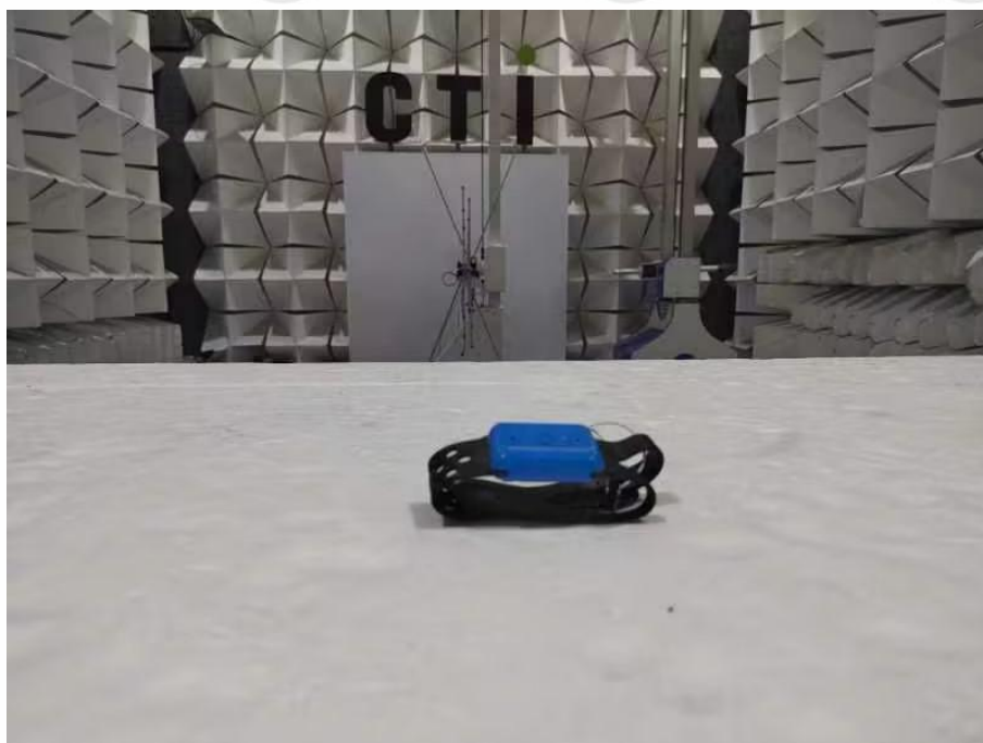
Radiated emission Test Setup-2(close up) (30MHz~1GHz)
