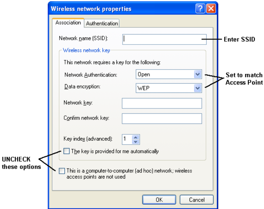
Figure 43: Add Wireless Network
