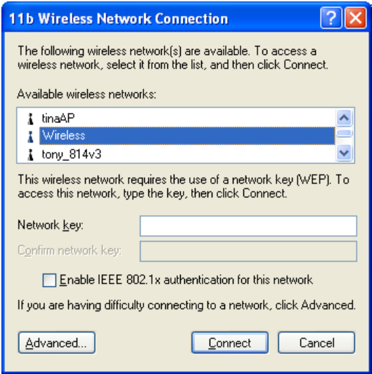
Figure 41: Wireless Networks (Windows XP)
