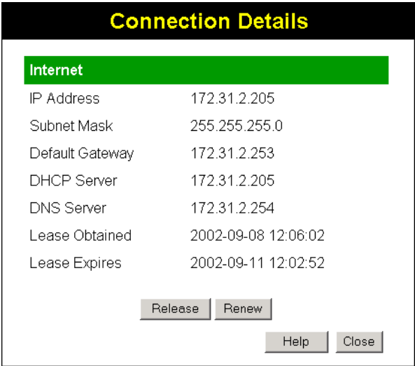
Figure 47: Connection Details - Fixed/Dynamic IP Address
