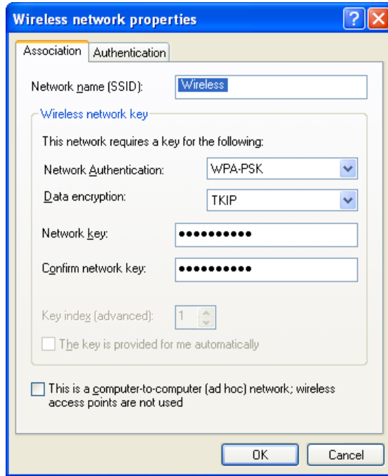
Figure 39: Wireless Network Properties- WPA-PSK
