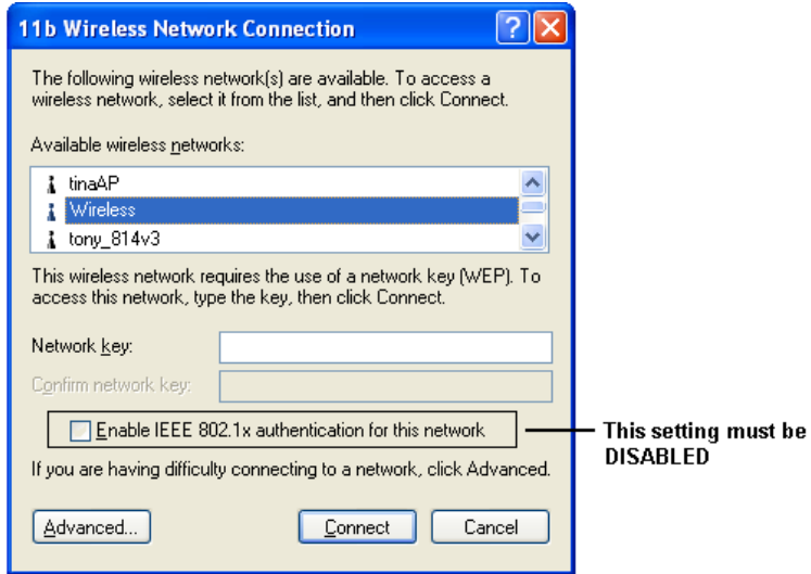
Figure 33: WEP (Windows XP)
