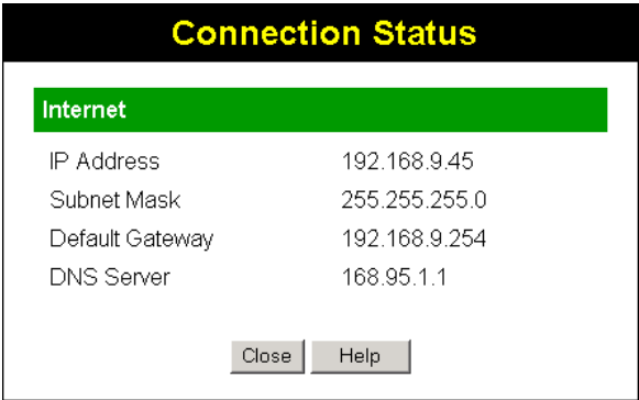
Figure 48: Connection Details - Fixed/Dynamic IP Address
