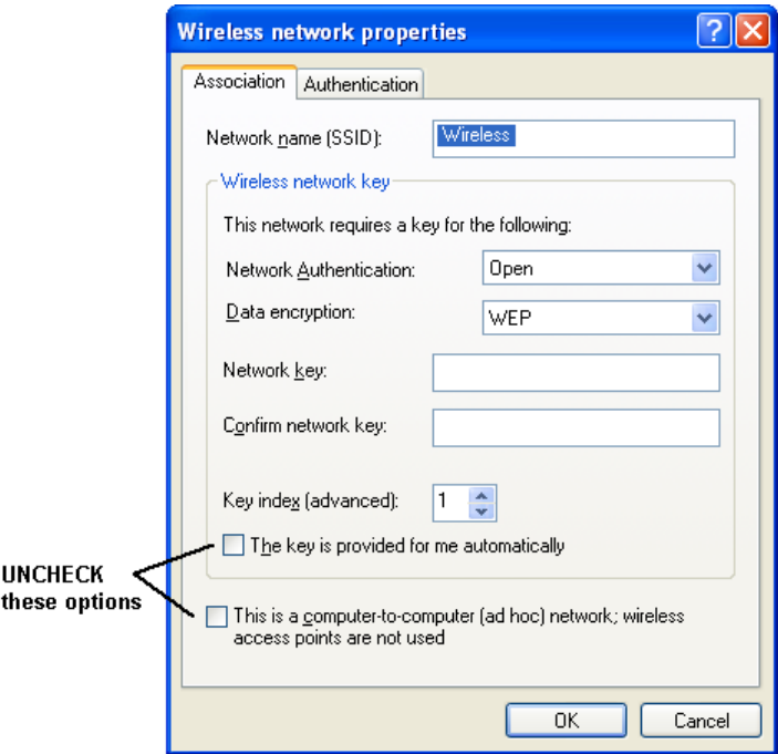
Figure 35: Wireless Network Properties - WEP
