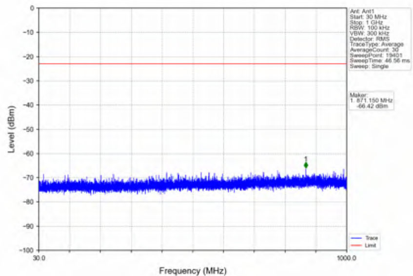
n41_15kHz_SISO_NTNV_30MHz_CP-OFDM_QPSK_2674.995MHz_Inner_1RB_Right
