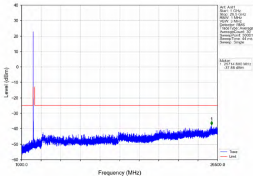
n41_15kHz_SISO_NTNV_15MHz_CP-OFDM QPSK_2503.5MHz_Outer_Full
