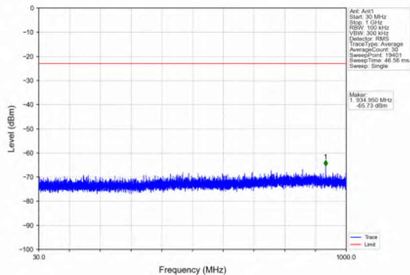
n41_15kHz_SISO_NTNV_20MHz_CP-OFDM QPSK_2679.99MHz_Outer_Full
