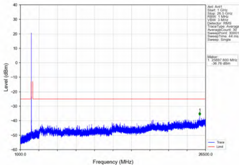
n41_15kHz_SISO_NTNV_20MHz_CP-OFDM_QPSK_2506.005MHz_Outer_Full
