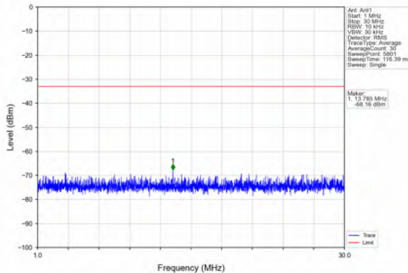
n41_15kHz_SISO_NTNV_30MHz_CP-OFDM_QPSK_2674.995MHz_Edge_1RB_Right
