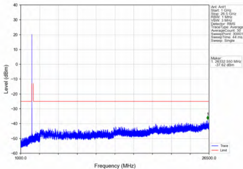
n41_15kHz_SISO_NTNV_15MHz_DFT-s-OFDM_QPSK_2503.5MHz_Edge_1RB_Left
