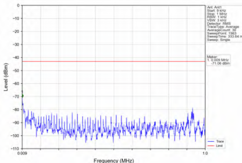
n41_15kHz_SISO_NTNV_30MHz_DFT-s-OFDM_QPSK_2674.995MHz_Outer_Full
