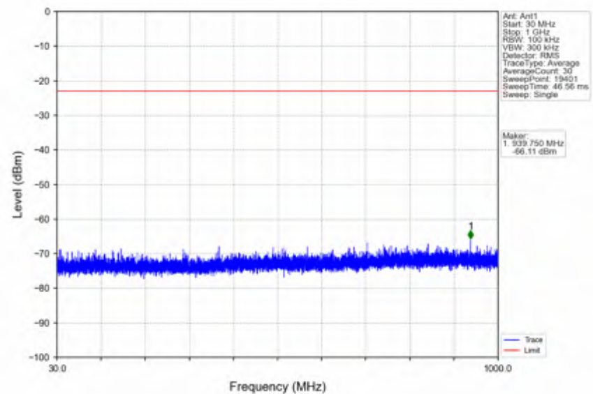
n41_15kHz_SISO_NTNV_30MHz_DFT-s-OFDM_QPSK_2511MHz_Outer_Full
