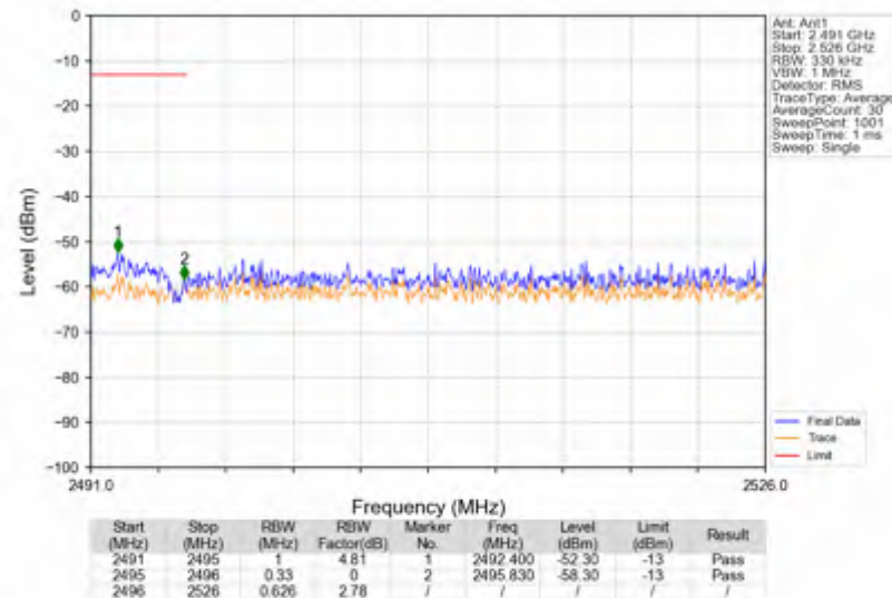
n41_15kHz_SISO_NTNV_30MHz_DFT-s-OFDM QPSK_2511MHz_Outer_Full
