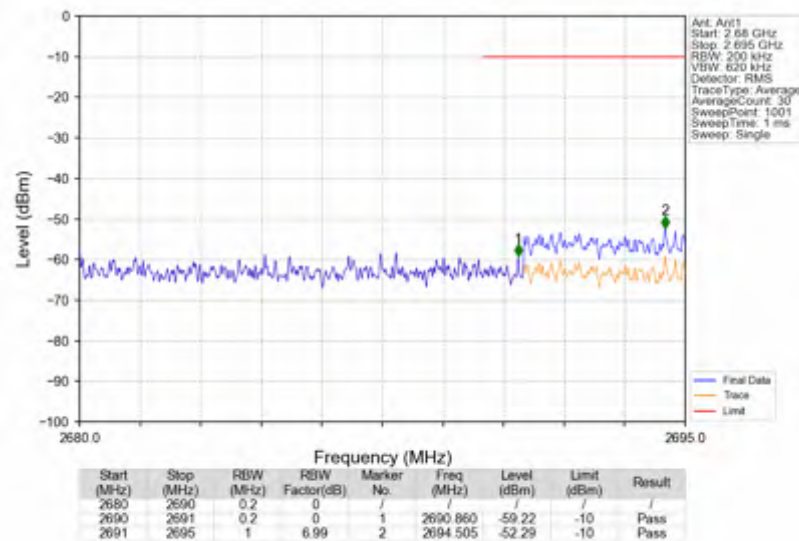
n41_15kHz_SISO_NTNV_10MHz_CP-OFDM QPSK_2685MHz_Outer_Full
