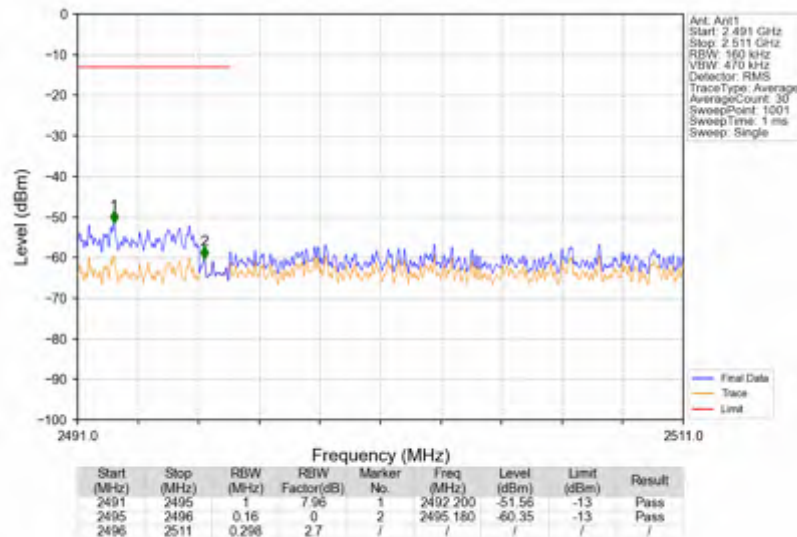
n41_15kHz_SISO_NTNV_15MHz_DFT-s-OFDM PI/2 BPSK_2503.5MHz_Outer_Full
