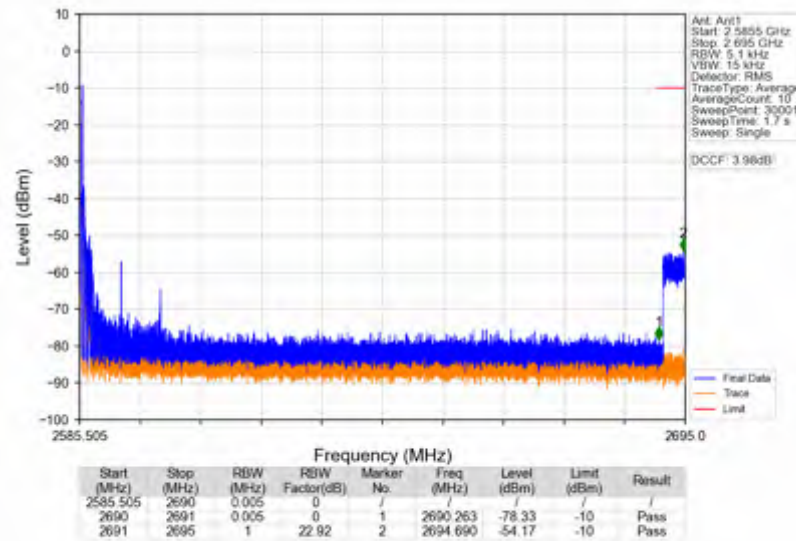
n41_15kHz_SISO_NTNV_15MHz_DFT-s-OFDM_QPSK_2593.005MHz_Edge_1RB_Left
