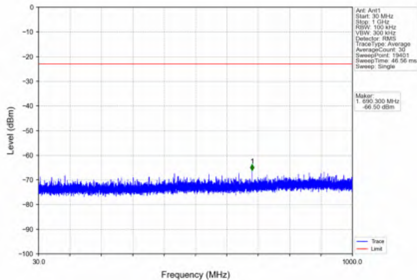
n41_15kHz_SISO_NTNV_20MHz_CP-OFDM_QPSK_2506.005MHz_Outer_Full
