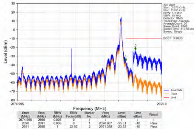
n41_15kHz_SISO_NTNV_15MHz_CP-OFDM_QPSK_2682.495MHz_Inner_1RB_Right
