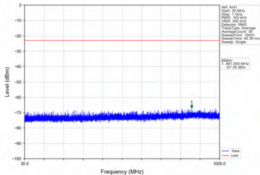
n41_15kHz_SISO_NTV_30MHz_CP-OFDM_QPSK_2511MHz_Outer_Full
