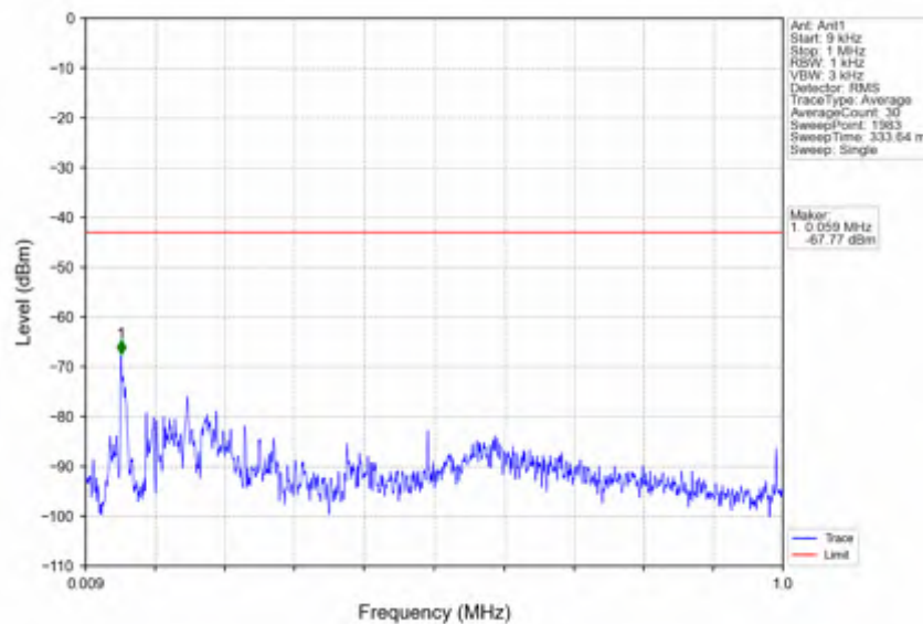
n41_15kHz_SISO_NTNV_20MHz_DFT-s-OFDM_QPSK_2679.99MHz_Outer_Full
