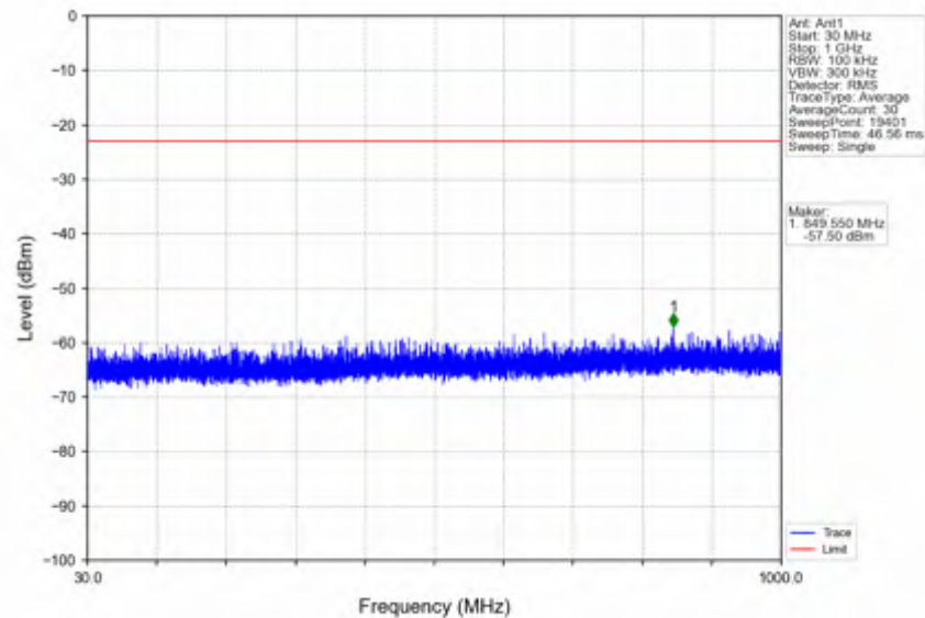
n41_15kHz_SISO_NTNV_20MHz_DFT-s-OFDM QPSK_2679.99MHz_Edge_1RB_Right
