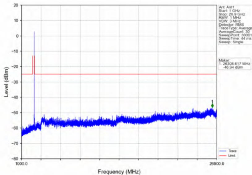
n41_15kHz_SISO_NTNV_15MHz_CP-OFDM QPSK_2682.495MHz_Outer_Full
