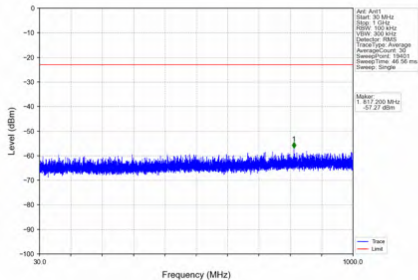
n41_15kHz_SISO_NTNV_15MHz_CP-OFDM QPSK_2503.5MHz_Edge_1RB_Left
