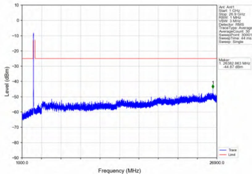
n41_15kHz_SISO_NTV_30MHz_CP-OFDM_QPSK_2511MHz_Outer_Full
