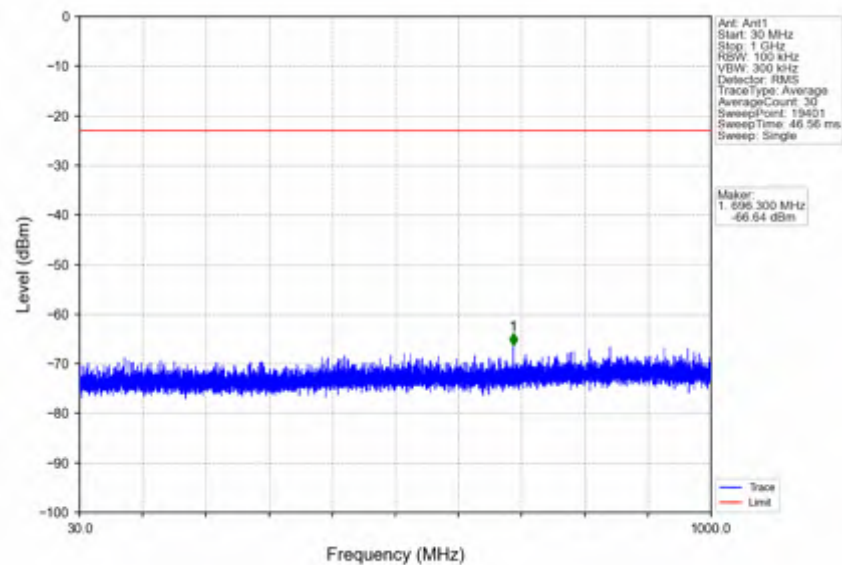
n41_15kHz_SISO_NTNV_30MHz_DFT-s-OFDM_PI/2_BPSK_2511MHz_Outer_Full
