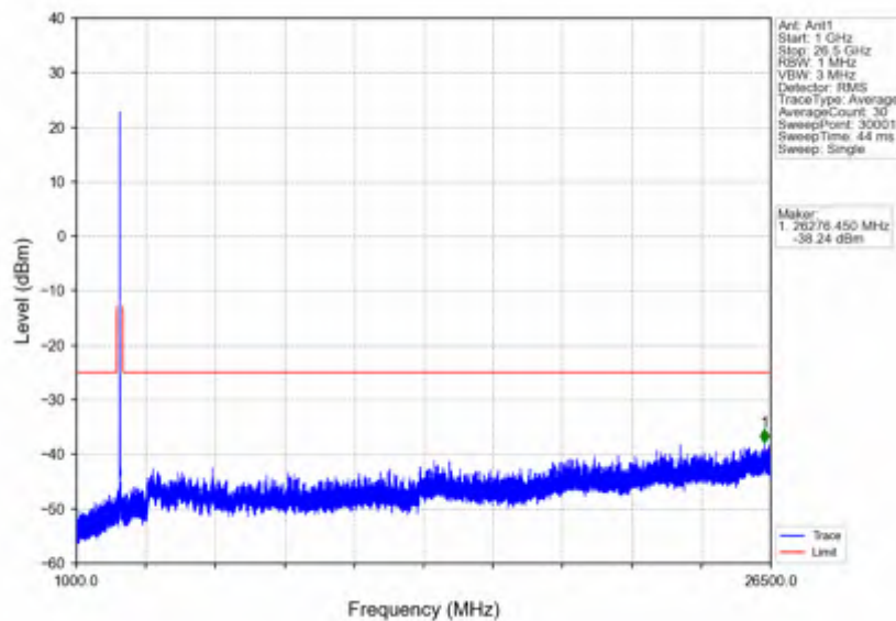
n41_15kHz_SISO_NTNV_20MHz_DFT-s-OFDM QPSK_2679.99MHz_Edge_1RB_Right
