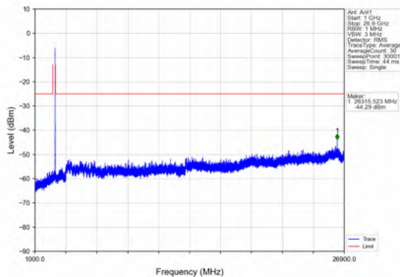
n41 15kHz SISO NTNV 15MHz CP-OFDM QPSK 2682.495MHz Outer Full
