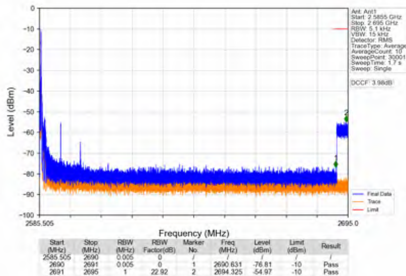
n41_15kHz_SISO_NTNV_15MHz_DFT-s-OFDM PI/2 BPSK_2593.005MHz_Edge_1RB_Left
