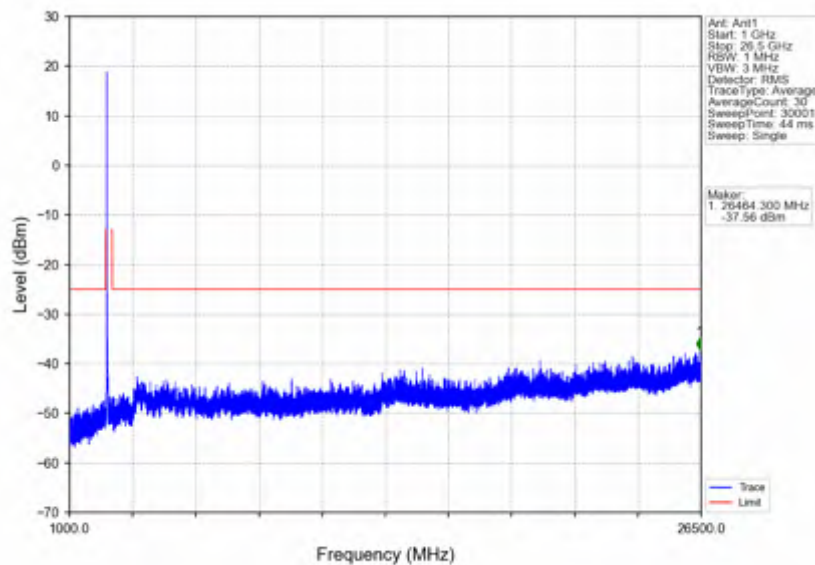
n41_15kHz_SISO_NTNV_30MHz_CP-OFDM QPSK_2511MHz_Outer_Full
