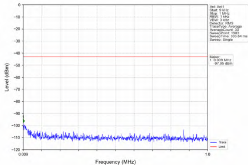
n41_15kHz_SISO_NTNV_30MHz_CP-OFDM QPSK_2511MHz_Outer_Full
