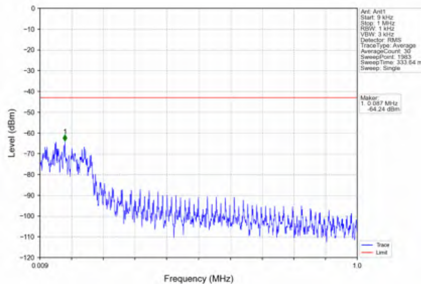
n41_15kHz_SISO_NTNV_15MHz_DFT-s-OFDM_QPSK_2593.005MHz_Edge_1RB_Left
