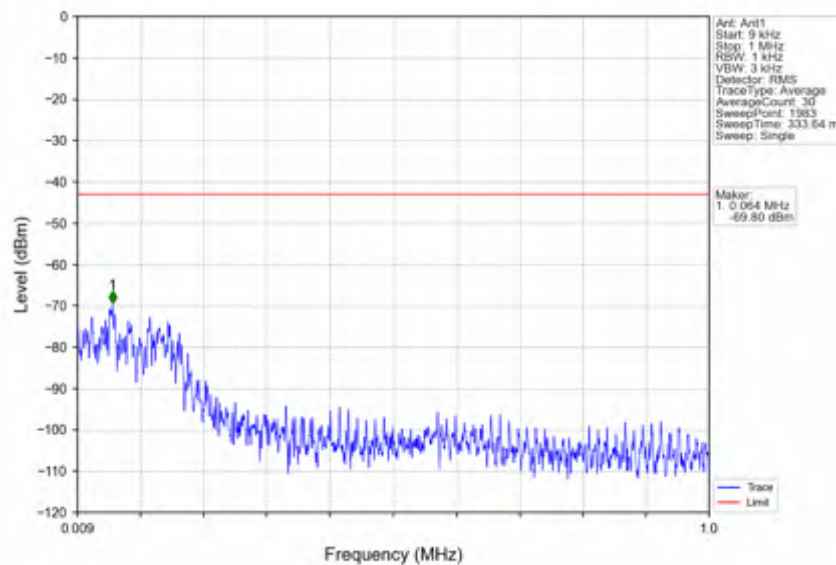
n41_15kHz_SISO_NTNV_40MHz_DFT-s-OFDM_PI/2_BPSK_2670MHz_Edge_1RB_Right
