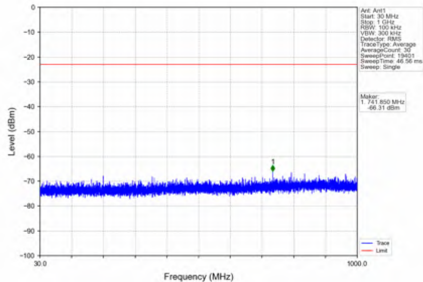
n41_15kHz_SISO_NTNV_15MHz_CP-OFDM_QPSK_2503.5MHz_Outer_Full
