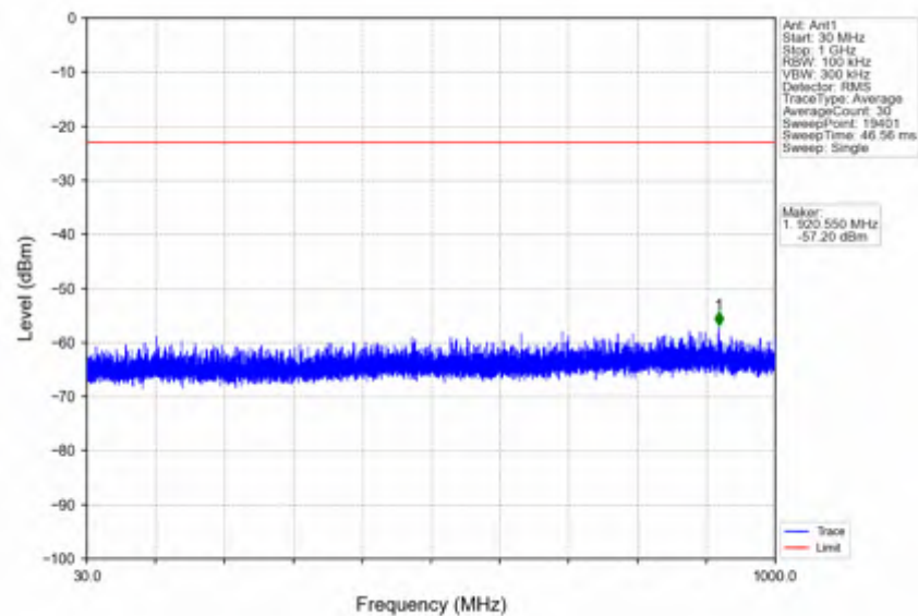
n41_15kHz_SISO_NTNV_15MHz_DFT-s-OFDM_QPSK_2682.495MHz_Edge_1RB_Right
