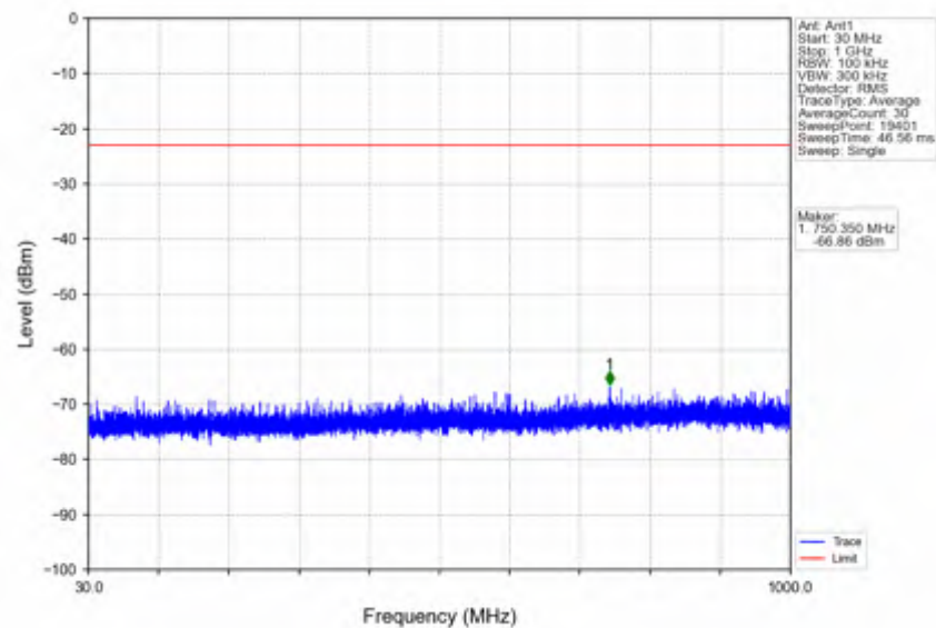
n41_15kHz_SISO_NTNV_10MHz_CP-OFDM QPSK_2501.01MHz_Outer_Full
