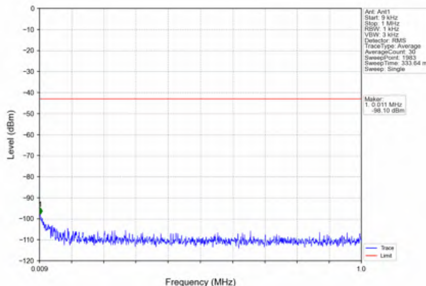
n41_15kHz_SISO_NTNV_15MHz_DFT-s-OFDM_QPSK_2682.495MHz_Outer_Full
