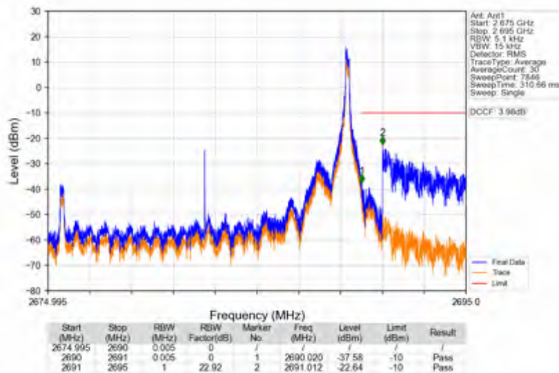
n41_15kHz_SISO_NTNV_15MHz_DFT-s-OFDM QPSK_2682.495MHz_Inner_1RB_Right
