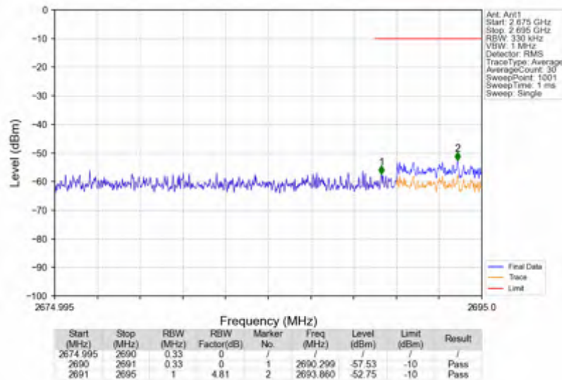
n41_15kHz_SISO_NTNV_15MHz_DFT-s-OFDM_QPSK_2682.495MHz_Outer_Full
