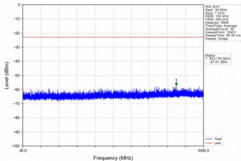
n41_15kHz_SISO_NTNV_15MHz_DFT-s-OFDM QPSK_2593.005MHz_Edge_1RB_Left
