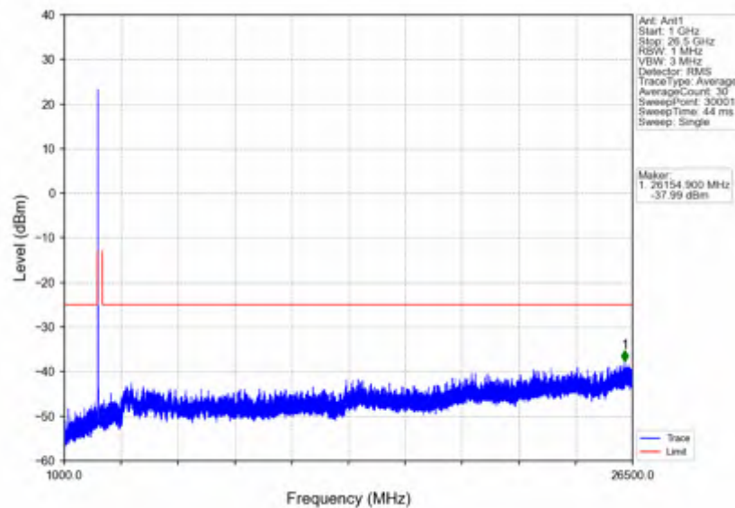
n41_15kHz_SISO_NTNV_15MHz_DFT-s-OFDM PI/2 BPSK_2503.5MHz_Outer_Full
