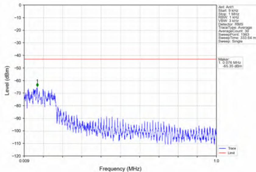
n41_15kHz_SISO_NTNV_30MHz_DFT-s-OFDM_QPSK_2593.005MHz_Edge_1RB_Left
