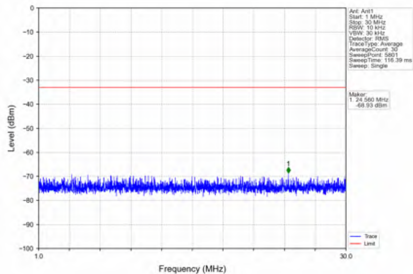
n41_15kHz_SISO_NTNV_30MHz_DFT-s-OFDM QPSK_2674.995MHz_Edge_1RB_Right
