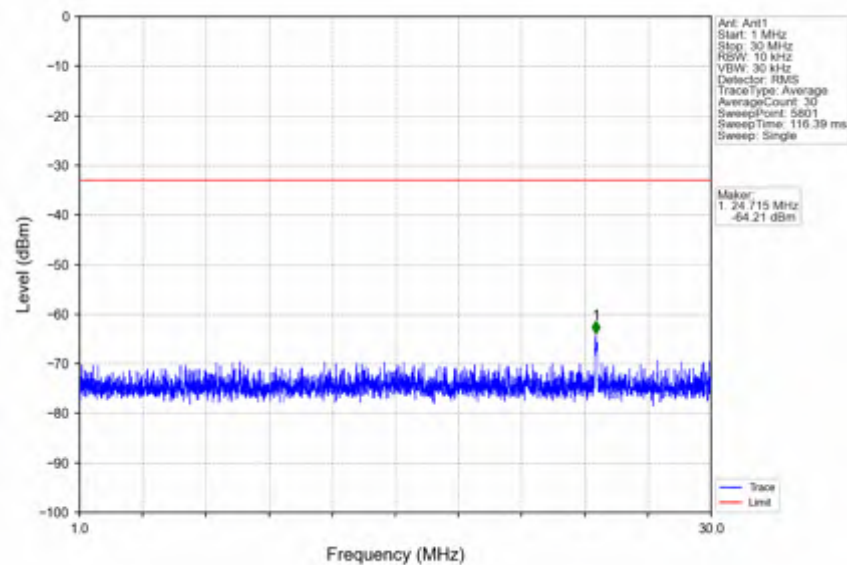
n41_15kHz_SISO_NTNV_15MHz_DFT-s-OFDM QPSK_2593.005MHz_Edge_1RB_Left
