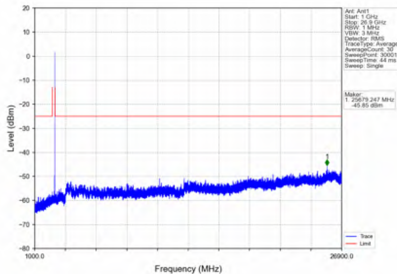
n41_15kHz_SISO_NTNV_15MHz_DFT-s-OFDM_QPSK_2682.495MHz_Edge_1RB_Right
