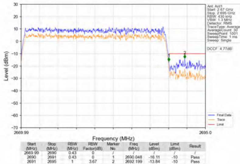
n41_15kHz_SISO_NTNV_20MHz_CP-OFDM QPSK_2679.99MHz_Outer_Full
