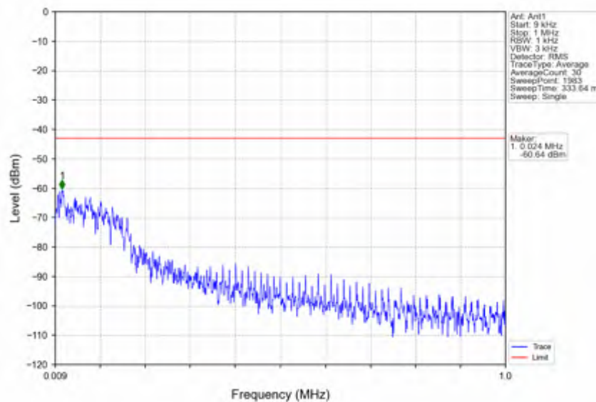
n41_15kHz_SISO_NTNV_15MHz_CP-OFDM_QPSK_2503.5MHz_Edge_1RB_Left
