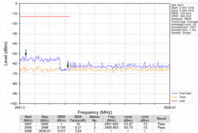
n41_15kHz_SISO_NTNV_10MHz_CP-OFDM QPSK_2501.01MHz_Outer_Full
