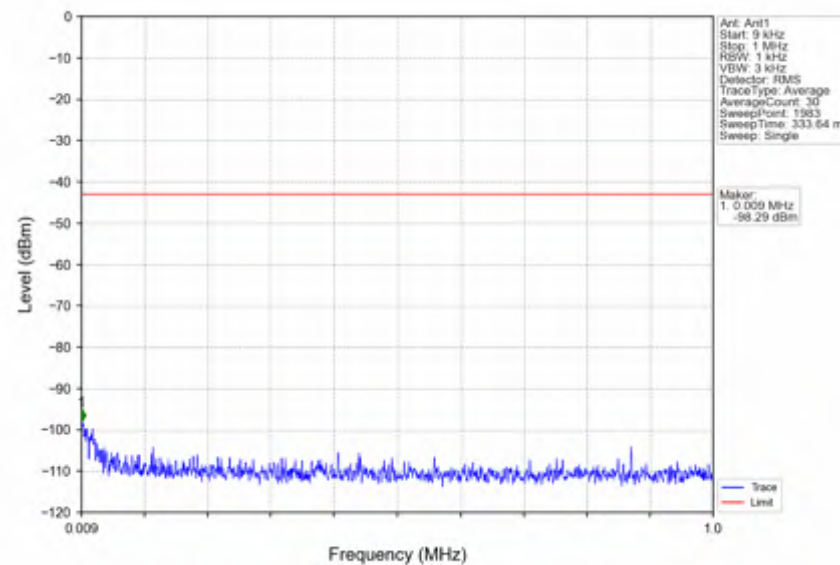
n41_15kHz_SISO_NTNV_30MHz_DFT-s-OFDM QPSK_2511MHz_Outer_Full
