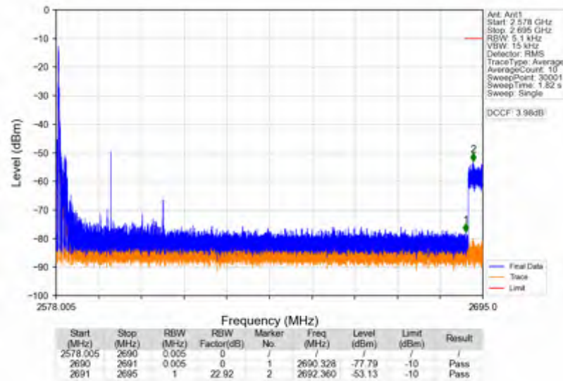
n41_15kHz_SISO_NTNV_30MHz_DFT-s-OFDM_QPSK_2593.005MHz_Edge_1RB_Left
