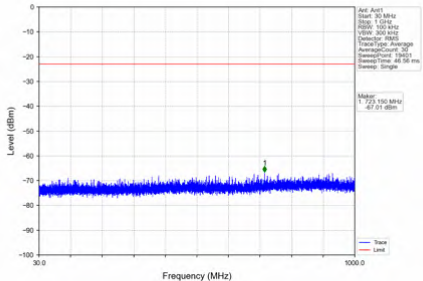
n41_15kHz_SISO_NTNV_15MHz_DFT-s-OFDM_QPSK_2682.495MHz_Outer_Full
