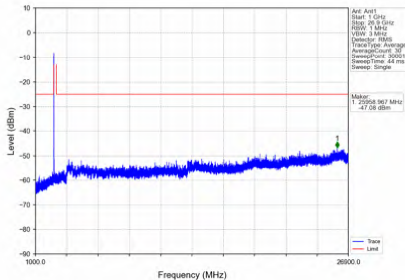
n41_15kHz_SISO_NTNV_10MHz_CP-OFDM QPSK_2501.01MHz_Outer_Full
