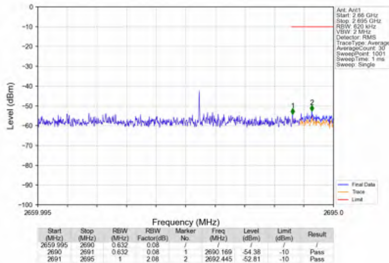
n41_15kHz_SISO_NTNV_30MHz_CP-OFDM QPSK_2674.995MHz_Outer_Full
