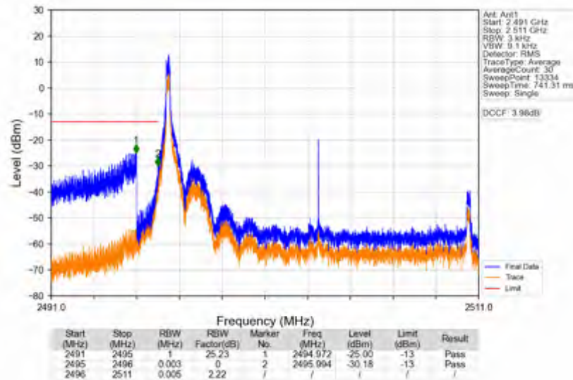
n41_15kHz_SISO_NTNV_15MHz_CP-OFDM_QPSK_2503.5MHz_Edge_1RB_Left
