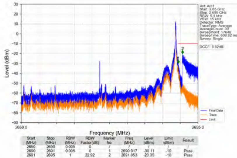
n41_15kHz_SISO_NTNV_40MHz_DFT-s-OFDM_PI/2_BPSK_2670MHz_Edge_1RB_Right
