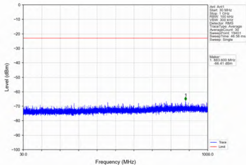
n41_15kHz_SISO_NTNV_15MHz_DFT-s-OFDM_QPSK_2682.495MHz_Inner_1RB_Right
