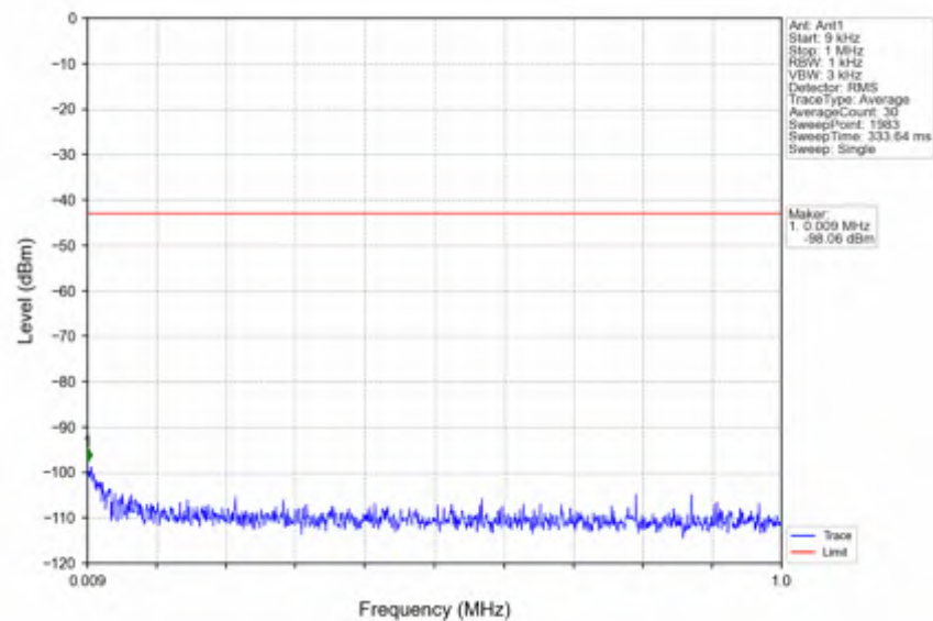
n41_15kHz_SISO_NTNV_10MHz_CP-OFDM QPSK_2501.01MHz_Outer_Full
