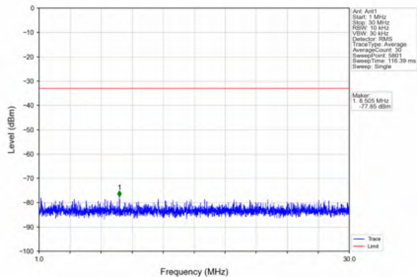
n41_15kHz_SISO_NTNV_20MHz_CP-OFDM QPSK_2679.99MHz_Outer_Full
