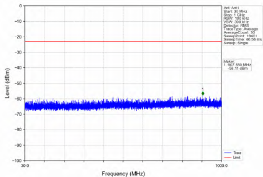
n41_15kHz_SISO_NTNV_30MHz_DFT-s-OFDM QPSK_2674.995MHz_Outer_Full
