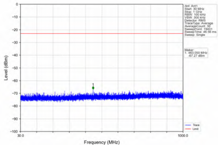
n41_15kHz_SISO_NTNV_15MHz_CP-OFDM_QPSK_2682.495MHz_Inner_1RB_Right
