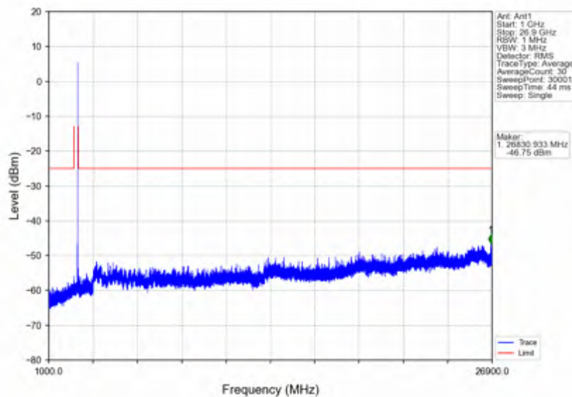
n41_15kHz_SISO_NTNV_30MHz_CP-OFDM QPSK_2674.995MHz_Outer_Full
