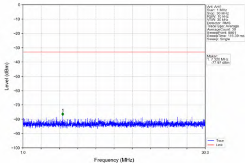
n41_15kHz_SISO_NTNV_15MHz_CP-OFDM_QPSK_2503.5MHz_Outer_Full
