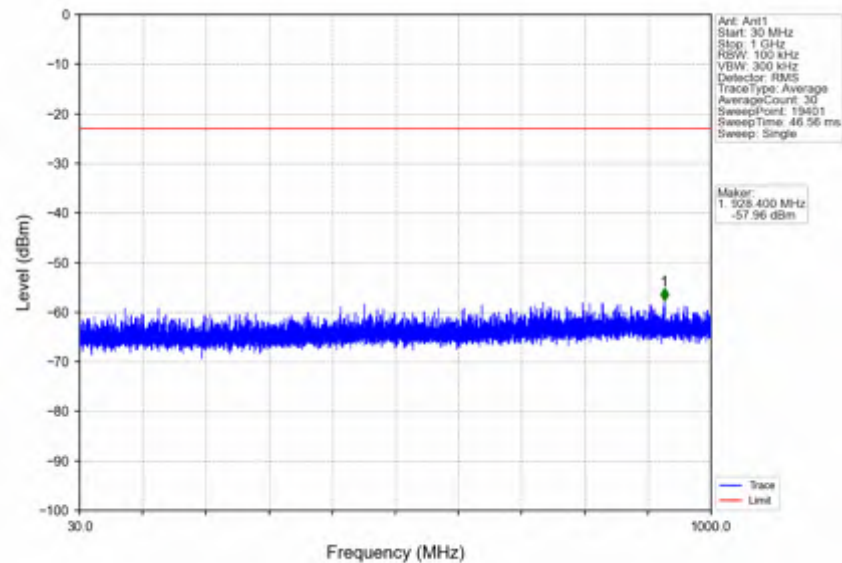
n41_15kHz_SISO_NTNV_20MHz_CP-OFDM QPSK_2679.99MHz_Edge_1RB_Right
