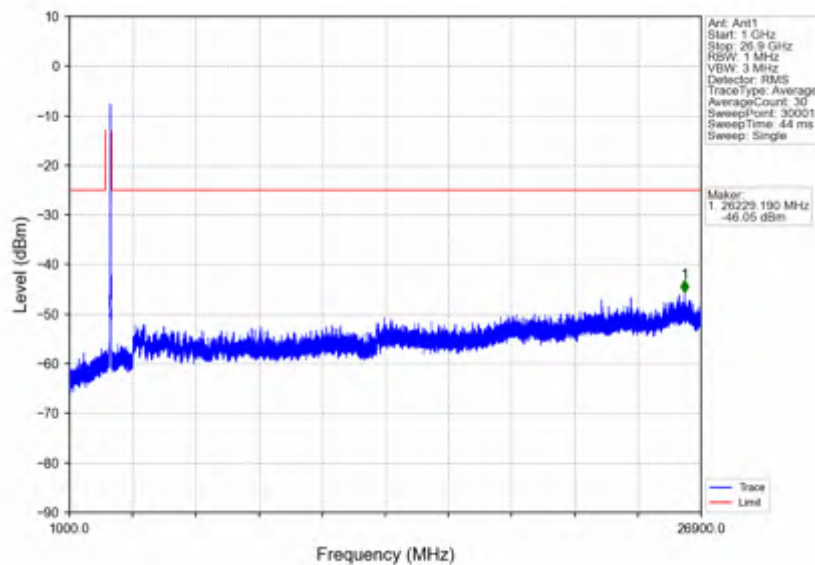
n41_15kHz_SISO_NTNV_30MHz_DFT-s-OFDM_QPSK_2674.995MHz_Inner_1RB_Right
