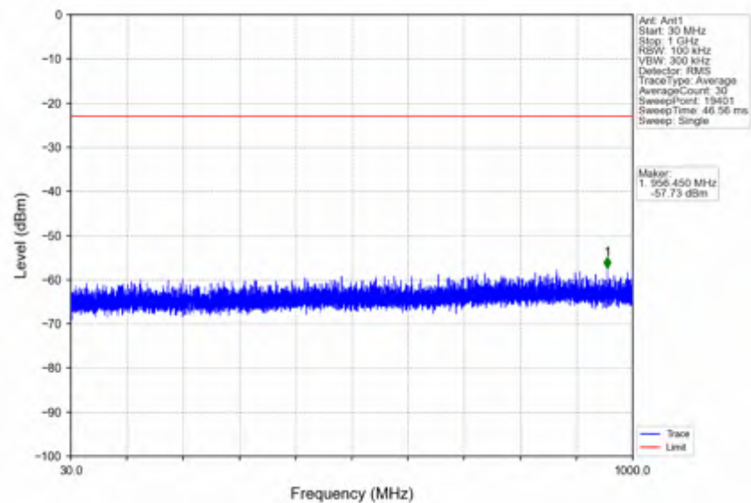
n41_15kHz_SISO_NTNV_30MHz_CP-OFDM_QPSK_2511MHz_Edge_1RB_Left
