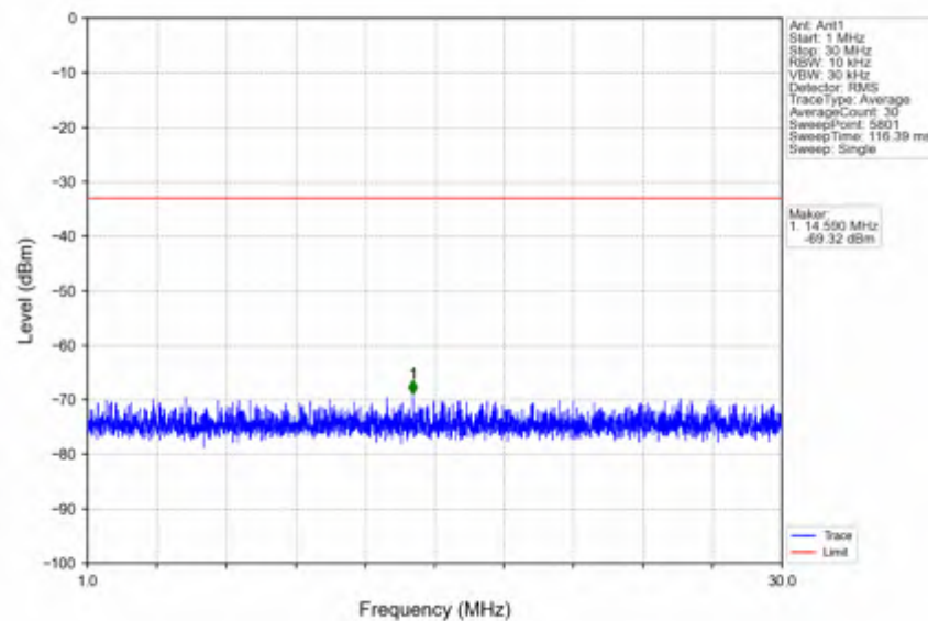
n41_15kHz_SISO_NTNV_15MHz_CP-OFDM QPSK_2593.005MHz_Edge_1RB_Left
