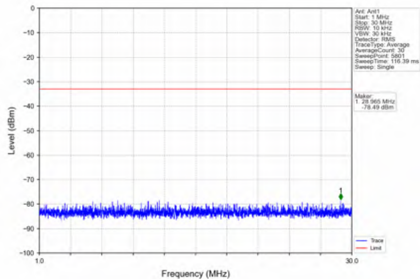
n41_15kHz_SISO_NTNV_20MHz_CP-OFDM_QPSK_2506.005MHz_Outer_Full
