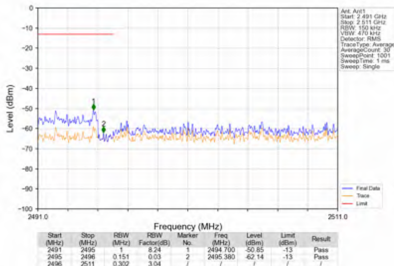
n41_15kHz_SISO_NTNV_15MHz_CP-OFDM QPSK_2503.5MHz_Outer_Full
