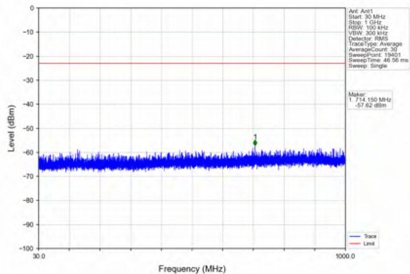
n41_15kHz_SISO_NTNV_15MHz_CP-OFDM_QPSK_2682.495MHz_Edge_1RB_Right
