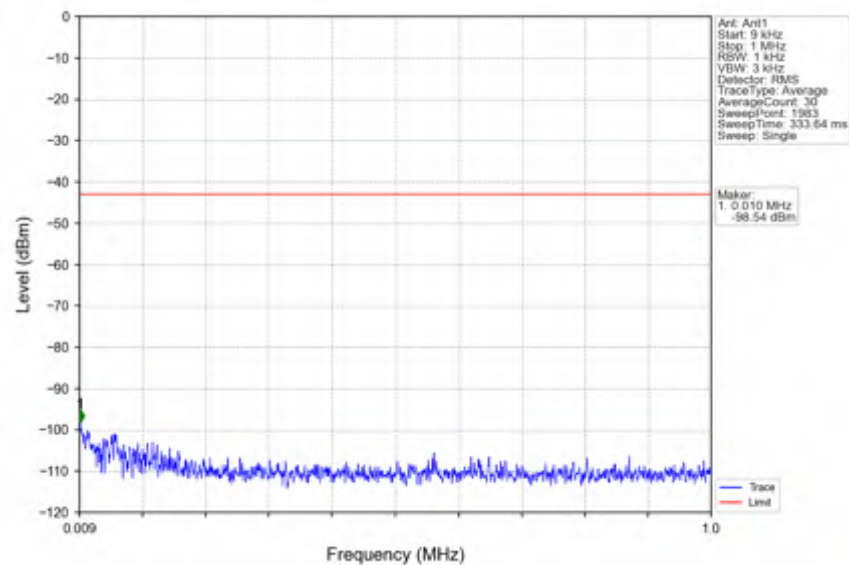
n41_15kHz_SISO_NTNV_15MHz_DFT-s-OFDM_QPSK_2682.495MHz_Inner_1RB_Right
