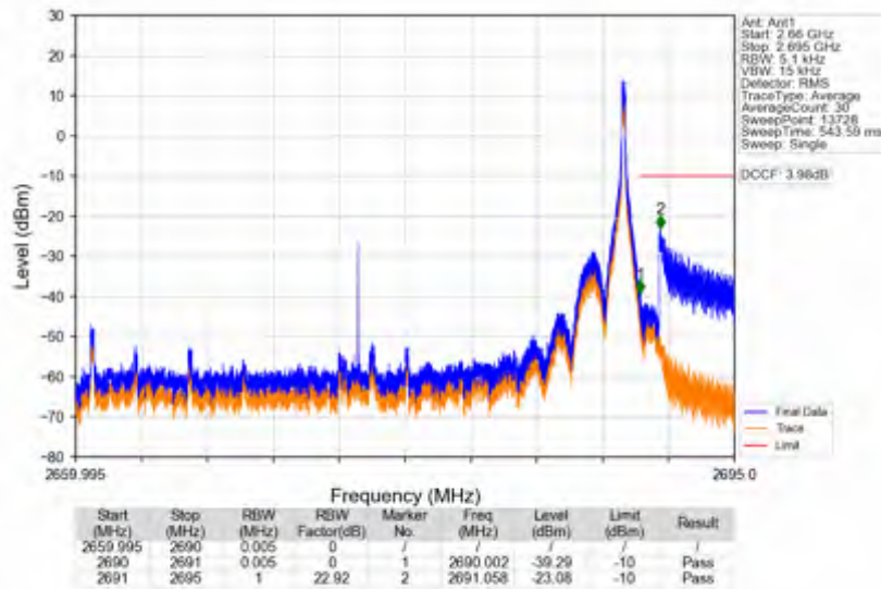
n41_15kHz_SISO_NTNV_30MHz_DFT-s-OFDM_QPSK_2674.995MHz_Inner_1RB_Right
