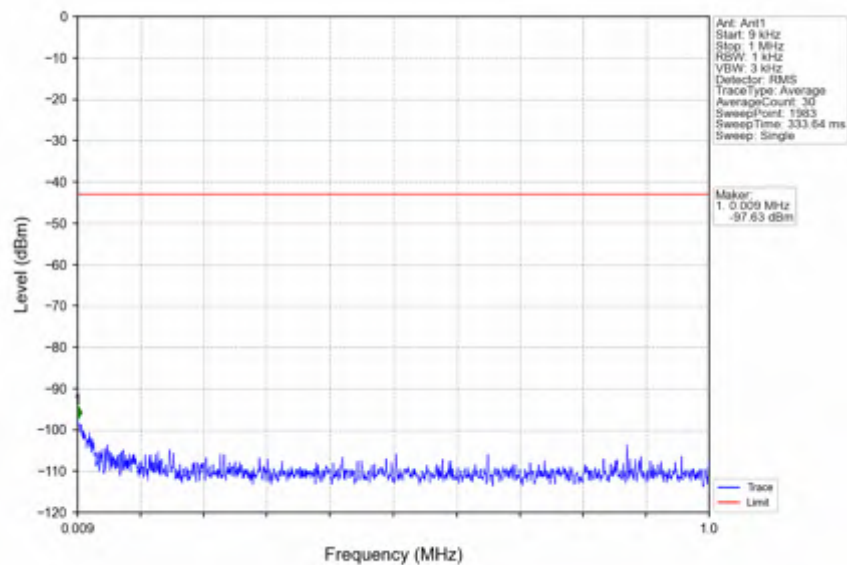
n41_15kHz_SISO_NTNV_30MHz_DFT-s-OFDM PI/2 BPSK_2511MHz_Outer_Full
