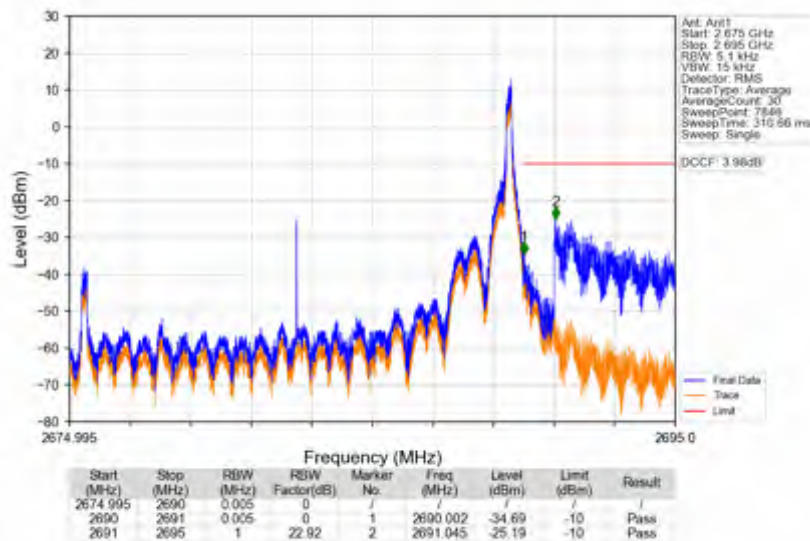
n41_15kHz_SISO_NTNV_15MHz_DFT-s-OFDM QPSK_2682.495MHz_Edge_1RB_Right
