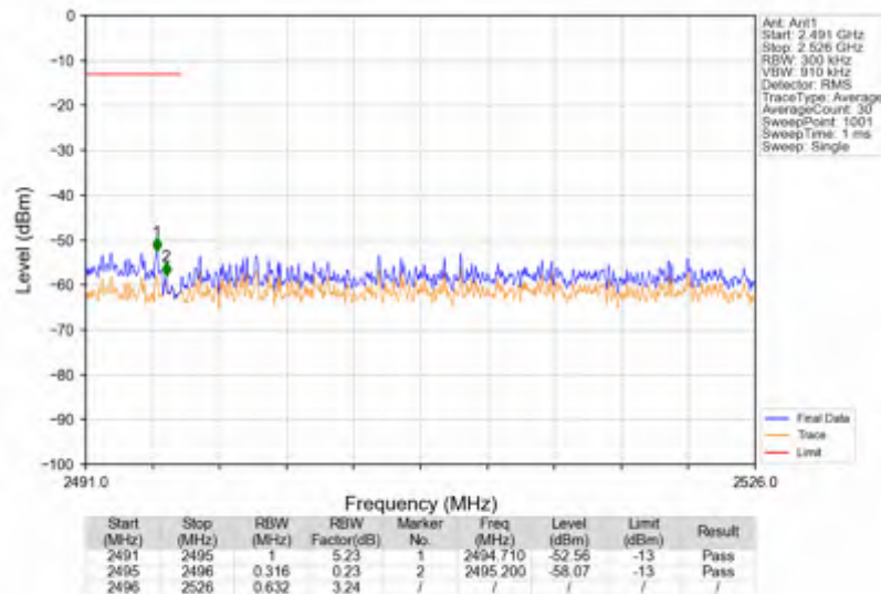
n41_15kHz_SISO_NTNV_30MHz_CP-OFDM QPSK_2511MHz_Outer_Full
