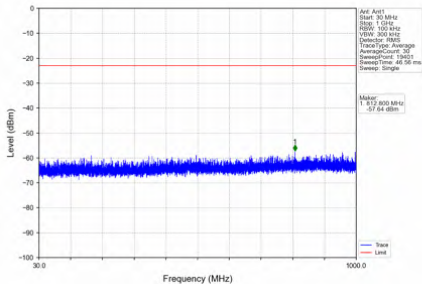
n41_15kHz_SISO_NTNV_15MHz_DFT-s-OFDM_QPSK_2503.5MHz_Edge_1RB_Left
