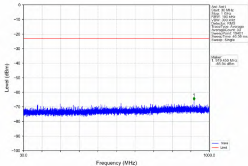
n41_15kHz_SISO_NTNV_10MHz_CP-OFDM_QPSK_2685MHz_Outer_Full
