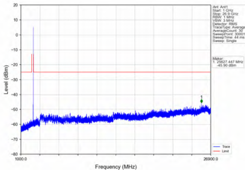
n41_15kHz_SISO_NTNV_20MHz_CP-OFDM QPSK_2679.99MHz_Outer_Full
