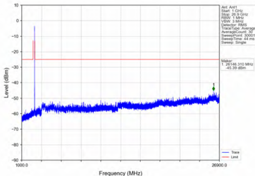
n41_15kHz_SISO_NTNV_15MHz_DFT-s-OFDM QPSK_2682.495MHz_Inner_1RB_Right
