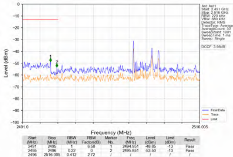
n41_15kHz_SISO_NTNV_20MHz_CP-OFDM_QPSK_2506.005MHz_Outer_Full
