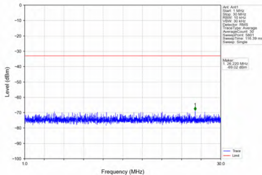
n41_15kHz_SISO_NTNV_30MHz_DFT-s-OFDM QPSK_2674.995MHz_Outer_Full
