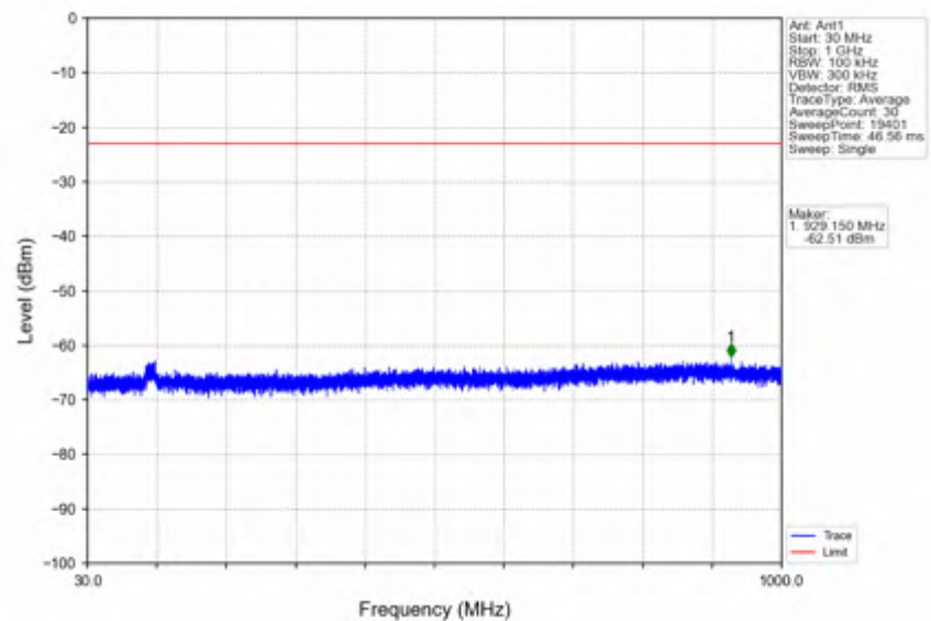
n41_15kHz_SISO_NTNV_20MHz_DFT-s-OFDM QPSK_2679.99MHz_Outer_Full
