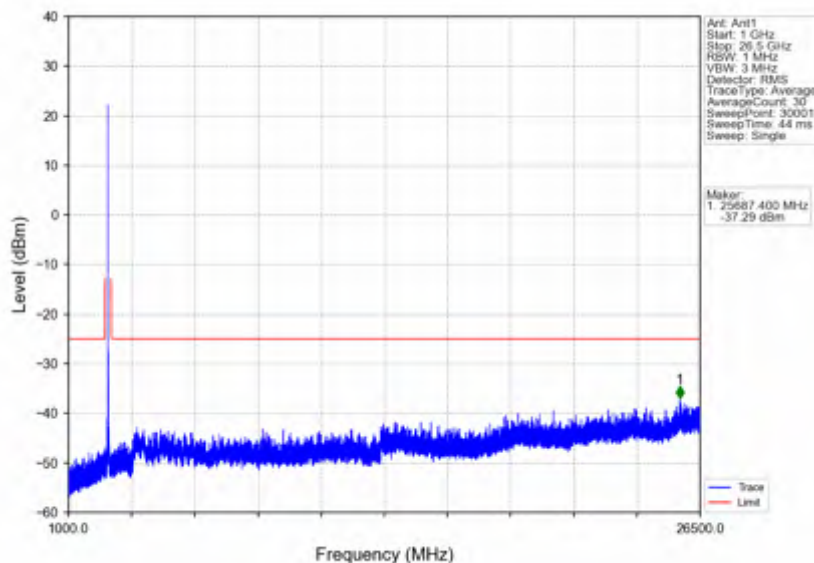
n41_15kHz_SISO_NTNV_30MHz_DFT-s-OFDM QPSK_2674.995MHz_Edge_1RB_Right
