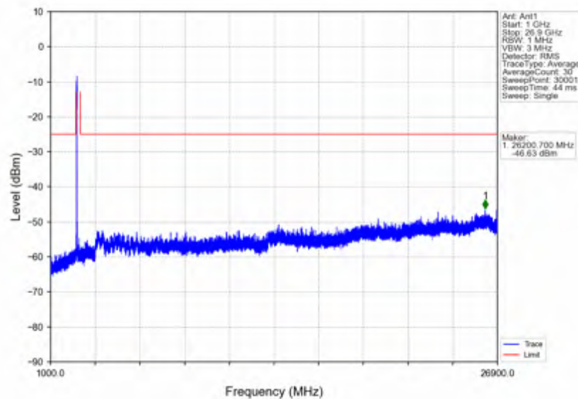
n41_15kHz_SISO_NTNV_30MHz_DFT-s-OFDM_PI/2_BPSK_2511MHz_Outer_Full
