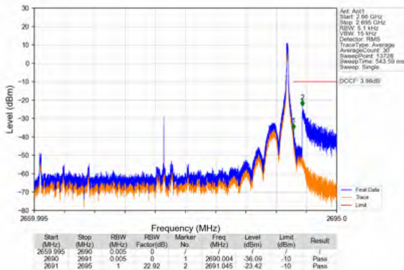
n41_15kHz_SISO_NTNV_30MHz_DFT-s-OFDM QPSK_2674.995MHz_Edge_1RB_Right
