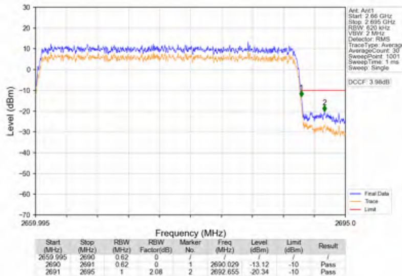
n41_15kHz_SISO_NTNV_30MHz_DFT-s-OFDM_QPSK_2674.995MHz_Outer_Full
