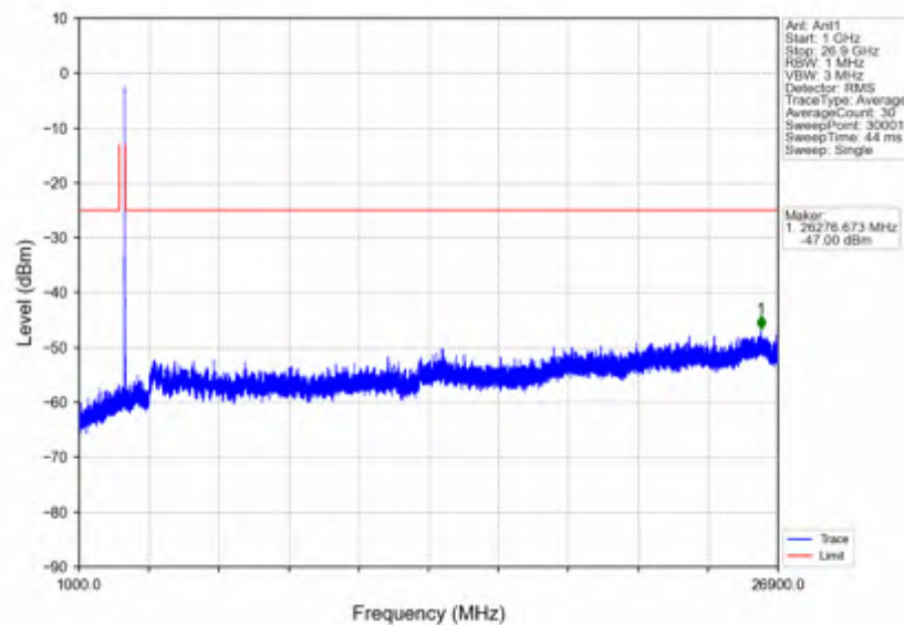
n41_15kHz_SISO_NTNV_10MHz_CP-OFDM_QPSK_2685MHz_Outer_Full
