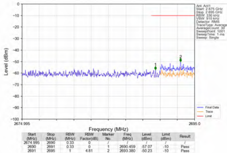
n41_15kHz_SISO_NTNV_15MHz_CP-OFDM QPSK_2682.495MHz_Outer_Full
