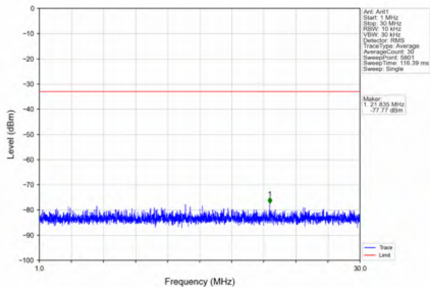
n41_15kHz_SISO_NTNV_30MHz_CP-OFDM_QPSK_2674.995MHz_Outer_Full
