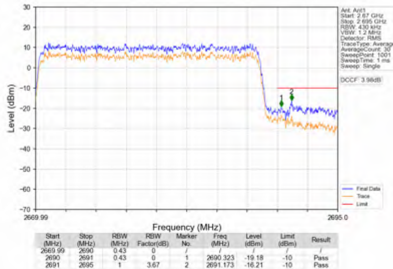
n41_15kHz_SISO_NTNV_20MHz_DFT-s-OFDM_QPSK_2679.99MHz_Outer_Full
