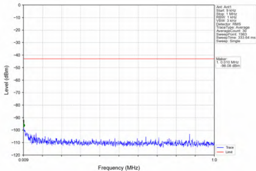
n41_15kHz_SISO_NTNV_10MHz_CP-OFDM_QPSK_2685MHz_Outer_Full
