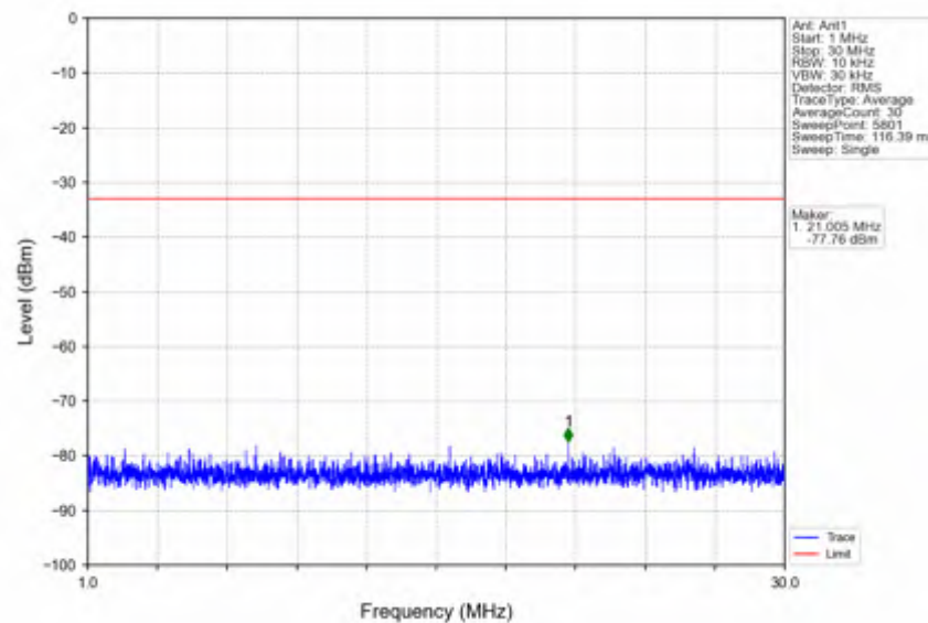
n41_15kHz_SISO_NTNV_15MHz_DFT-s-OFDM_QPSK_2503.5MHz_Outer_Full
