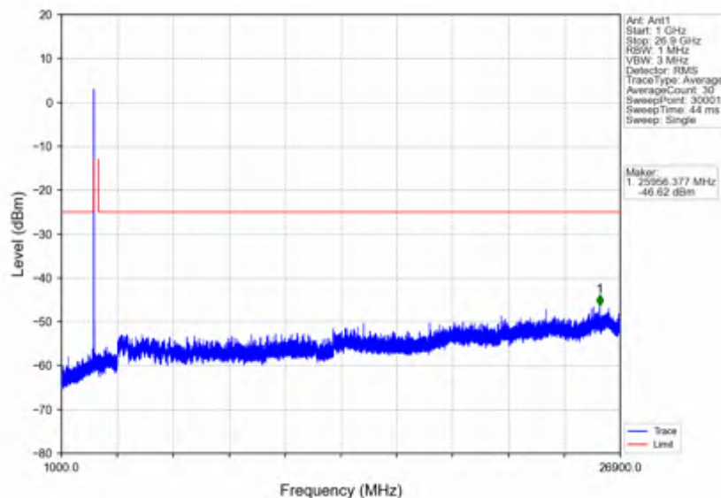
n41_15kHz_SISO_NTNV_15MHz_DFT-s-OFDM PI/2 BPSK_2593.005MHz_Edge_1RB_Left
