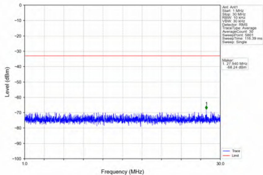
n41_15kHz_SISO_NTNV_15MHz_DFT-s-OFDM_QPSK_2682.495MHz_Edge_1RB_Right
