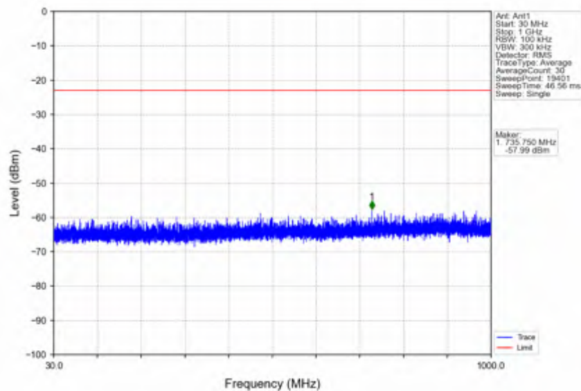
n41_15kHz_SISO_NTNV_20MHz_DFT-s-OFDM QPSK_2506.005MHz_Outer_Full
