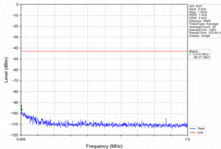
n41_15kHz_SISO_NTNV_15MHz_CP-OFDM_QPSK_2682.495MHz_Inner_1RB_Right
