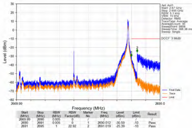
n41_15kHz_SISO_NTNV_20MHz_DFT-s-OFDM QPSK_2679.99MHz_Edge_1RB_Right
