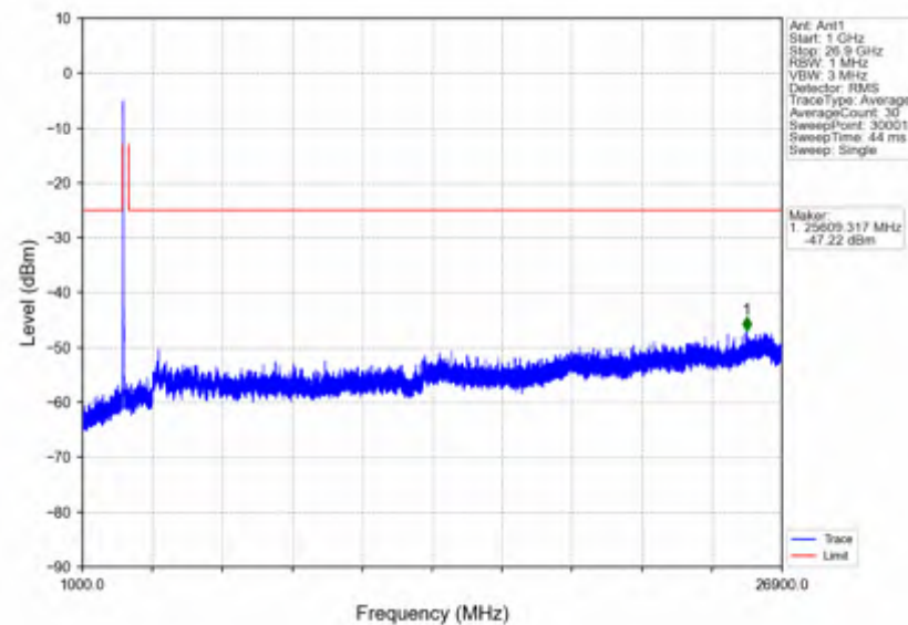
n41_15kHz_SISO_NTNV_15MHz_CP-OFDM_QPSK_2503.5MHz_Outer_Full
