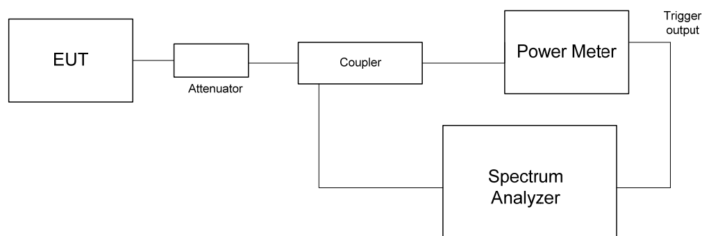
Figure 7.1.1 Peak output power test setup
