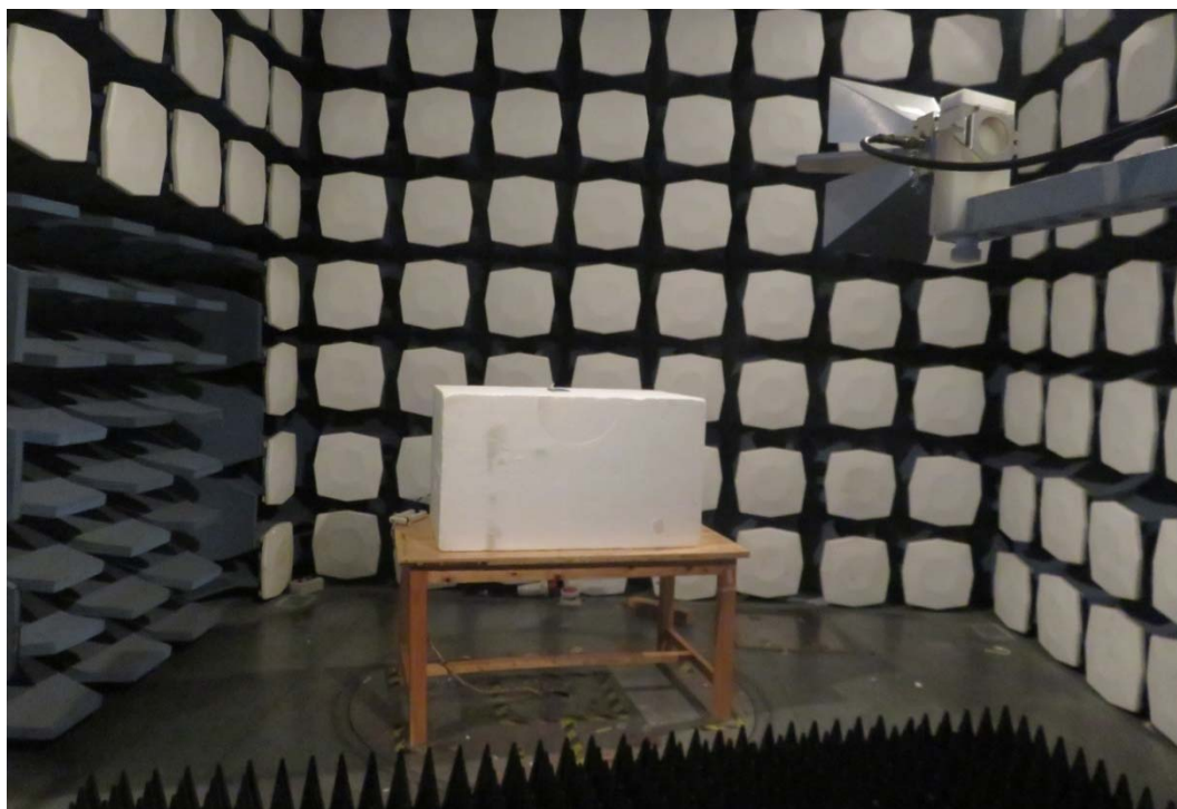
Above 1GHz
